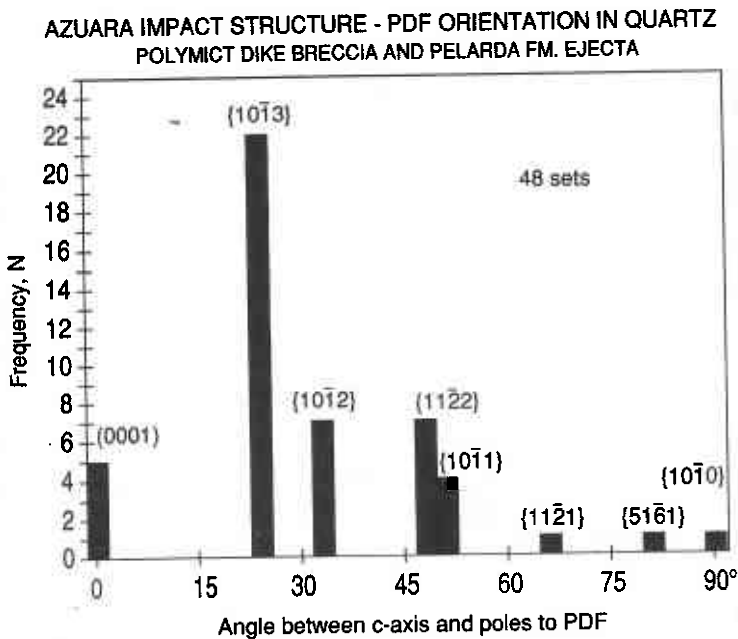
Fig. 8. Frequency diagram of crystallographic orientation of planar deformation features (PDFs) in quartz from Azuara mixed-breccia near Santa Cruz de Noguerras and from Pelarda Fm. ejecta. The diagram has been compiled from data put at our disposal by A. Therriault.
