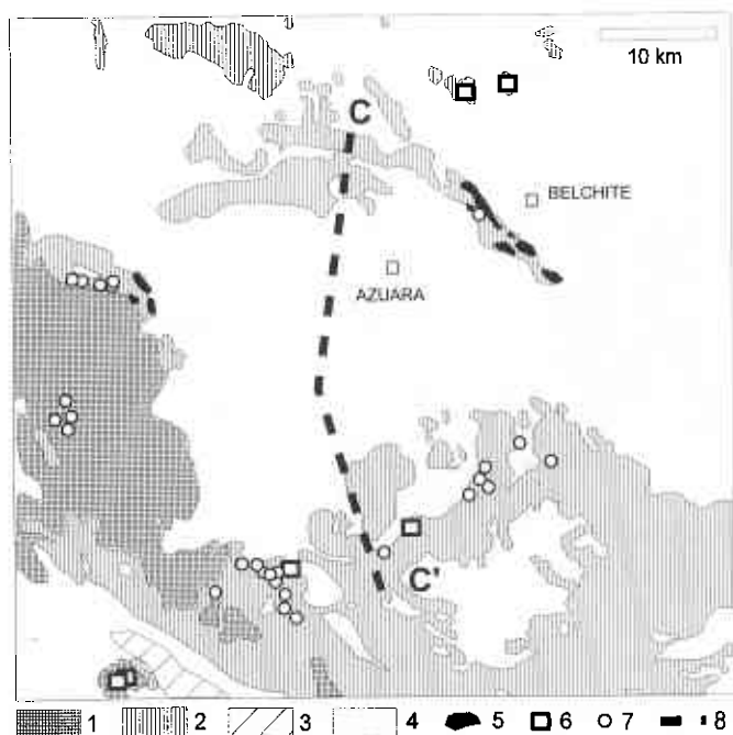
Fig. 5. Location map for the megabreccia (5), monomictic movement breccias (6), dislocated megablocks (7), and the gravity profile in Fig. 6 (8). Geology same as in Fig. 4.
