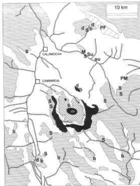
Fig. 11. Location map for impact features in the Rubielos de la Cérída structure. Geology same as in Fig. 9. PF = Pelarda Fm. ejecta, PM = Puerto Mínguez ejecta, b = basal (suevite) breccia, d = breccia dikes, M = impact melt rocks, Su = suevite, su = suevite-like impact breccia, s = shock metamorphism.
