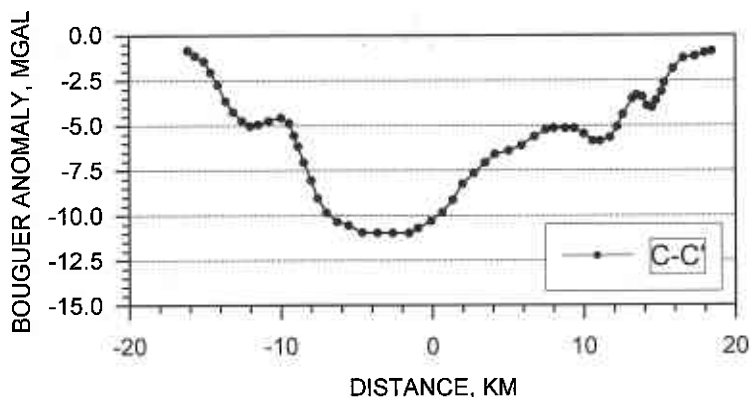
Fig. 6. Gravity profile (Bouguer residual anomalies) across the Azuara structure. Location for the profile in Fig. 5.
