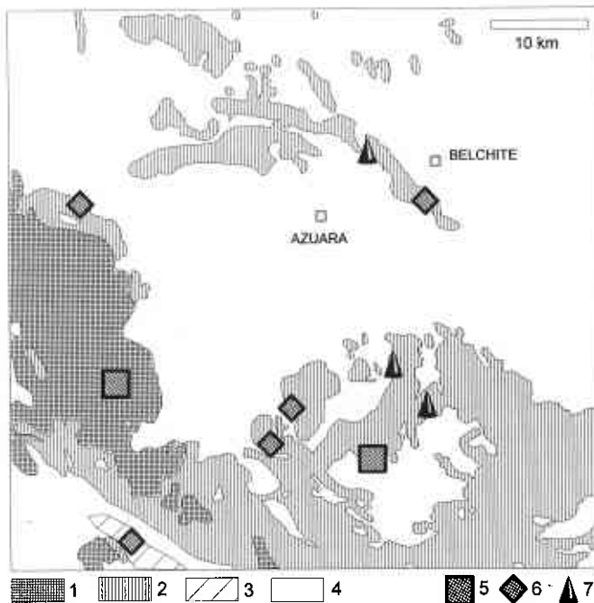
Fig. 7. Location map for strongly shocked rocks (5), moderately shocked rocks (6), and shatter cones (7). Geology same as in Fig. 4.
