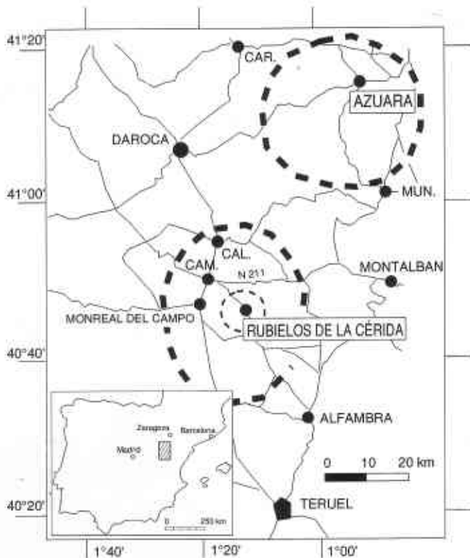
Fig. 1. Location map for the Azuara and Rubielos de la Cérída impact structures. CAL = Calamocha, CAM = Caminreal, CAR = Cariñena, MUN = Muniesa.
