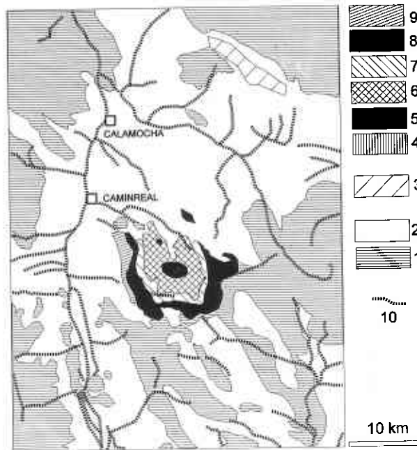
Fig. 9. Geological sketch map for the Rubielos de la Cérica impact structure, simplified and modified from ITGE (1991) and IGME (1986). 1 = Palaeozoicum, Mesozoicum and Lower Tertiary, 2 = Upper Tertiary and Quaternary, 3 = Pelarda Fm. ejecta; central uplift: 4 = Muschelkalk, 5 = Keuper, 6 = Rhaetian and Liassic, 7 = Dogger, 8 = Malmian, 9 = Cretaceous; 10 = drainage pattern.
