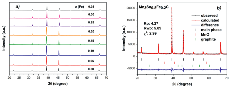
Figure 7.2: a) XRD patterns of Mn_3Sn_{1-x}Fe_xC compounds obtained at 298 K, b) Rietveld refinement of x = 0.20 at 298 K.
