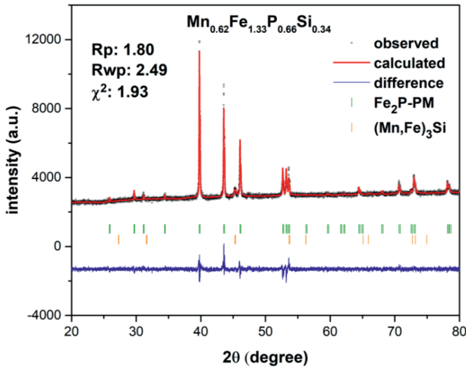
Figure 4.3: Observed and calculated XRD patterns of \text{Mn}_{0.62}\text{Fe}_{1.33}\text{P}_{0.66}\text{Si}_{0.34} .
