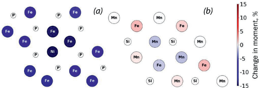
Figure 4.10: Change of the local magnetic moment upon 2 at.% Ni doping in the (a) 3f site and (b) 3g site. Note that Ni prefers the 3f site.
