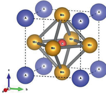
Figure 1.4: Unit cell of the Mn_3AC antiperovskite carbide, where A is a metal or semiconductor.
