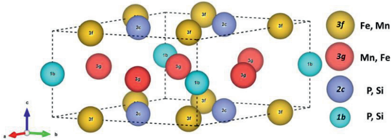
Figure 1.3: Unit cell of the hexagonal (\text{Mn,Fe})_2(\text{P,Si}) structure with specified crystallographic sites.
