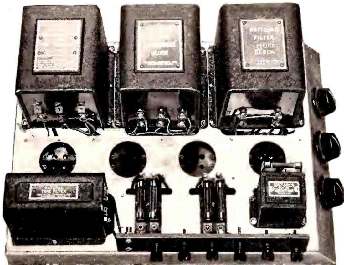
FIG. 2 RADIO BROADCAST Photograph Top view of the completed unit. The condenser block is placed between the power transformer and the choke coils in order to reduce any possibility of the choke coils picking up stray magnetic flux from the transformer
