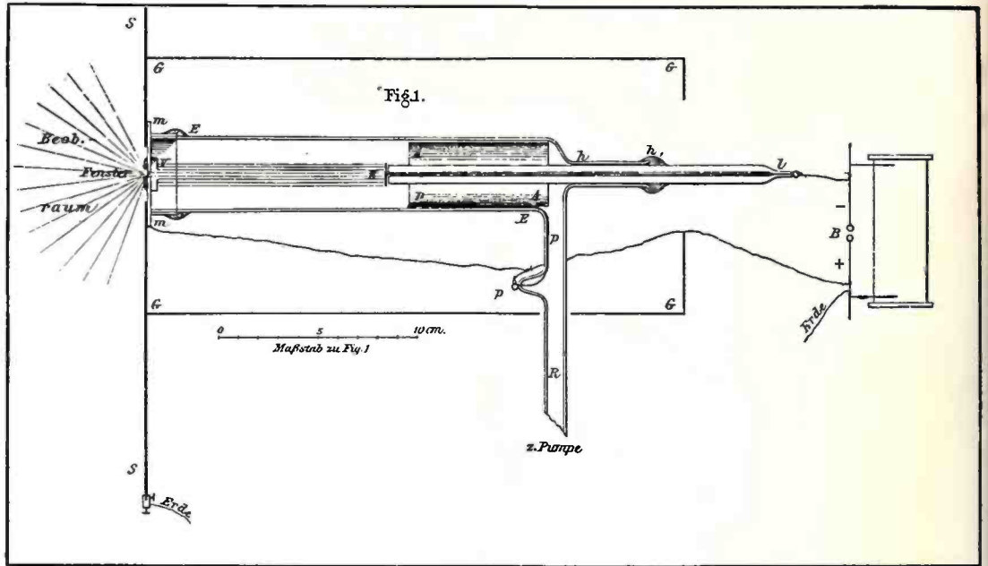
LENARD'S CATHODE RAY TUBE
