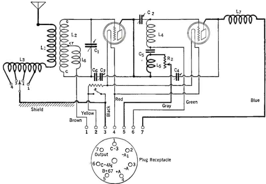
THE CIRCUIT OF THE TWO-TUBE TUNER UNIT
