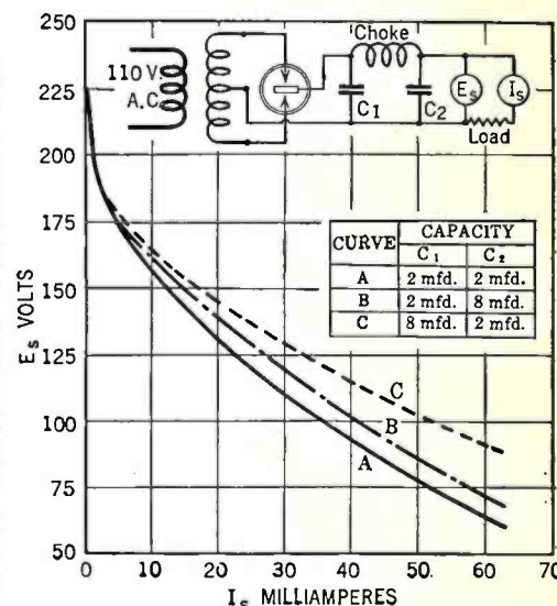
The curves shown are for a single section filter using the Raytheon tube as a rectifier. A multi-section filter would, however, give the same type of curves.
