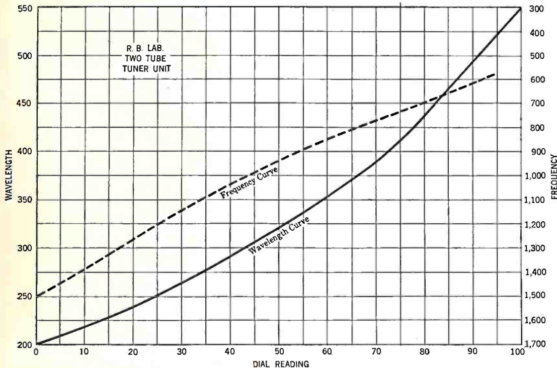
AN APPROXIMATE TUNING CHART
