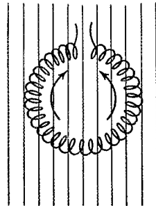
FIG. 2. Light vertical lines represent a magnetic field cutting the toroid. Arrows show the resulting (and opposing) voltages in the two halves of the coil.
