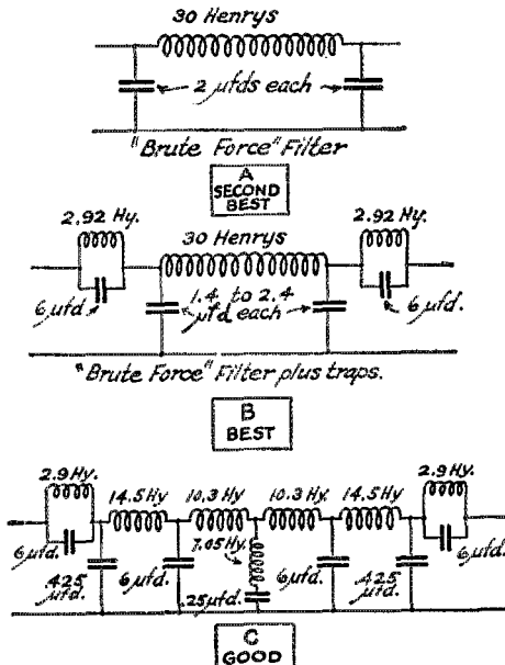
FIG. 21 THREE GOOD FILTERS FOR RECTIFIED 60~A.C.
