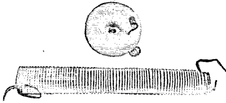
FIG. 1. AN EXPERIMENTAL TOROIDAL COIL IN WORKING CONDITION AND UNROLLED.
