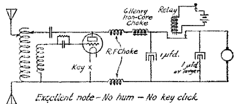
FIG 3 THE FINAL CIRCUIT
