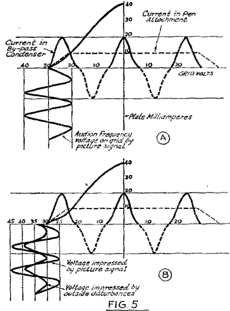
FIG. 5 The method of eliminating interference by means of grid bias adjustments.
