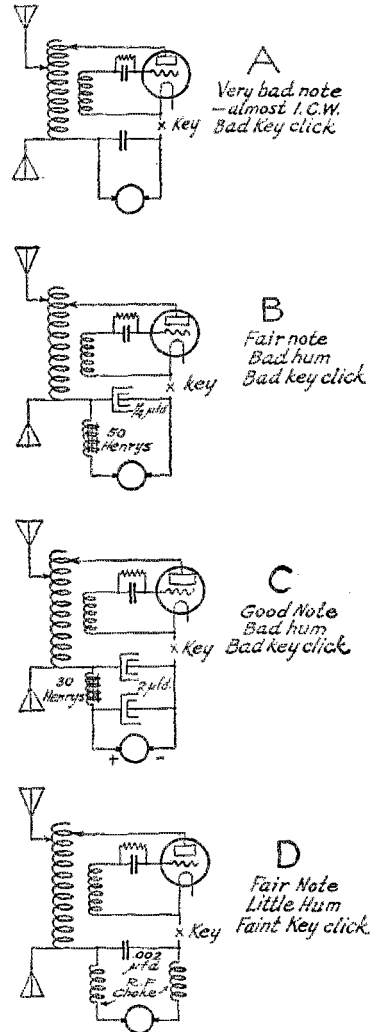
FIG. 1 THE SERIES FEED TEST CIRCUIT
