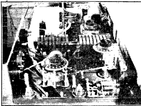
FIG. 4. THE TRANSMITTER. NOTE THE VERY LOW-LOSS CONSTRUCTION AND THE HEAVY LEADS.
