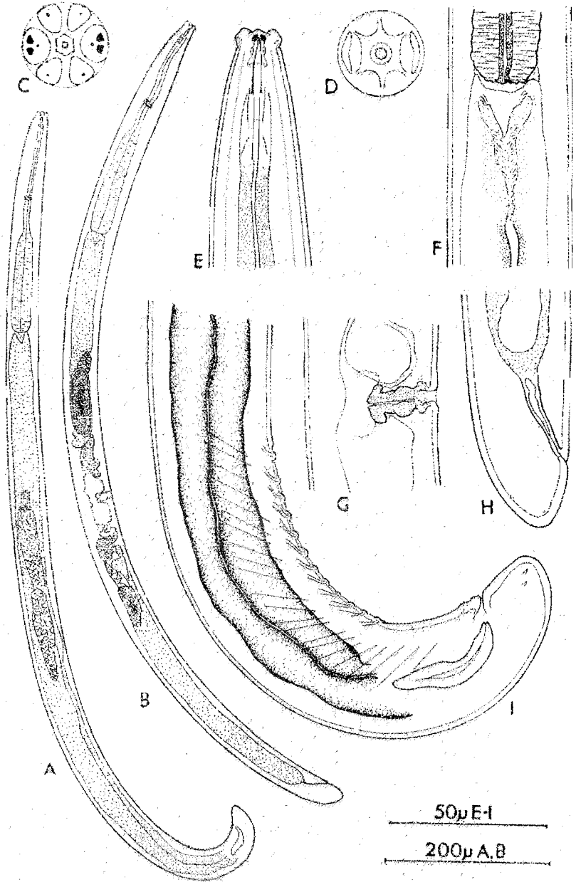
FIG. 9 A-I.— Crassolabium australe n. gen. et sp. A. Entire male. B. Entire female. C. En face view of lips. D. En face view at level of amphids. E. Anterior-intestinal region. F. Oesophago-intestinal junction. G. Lateral view of vulval region. H. Lateral view of female tail. I. Lateral view of male tail.
