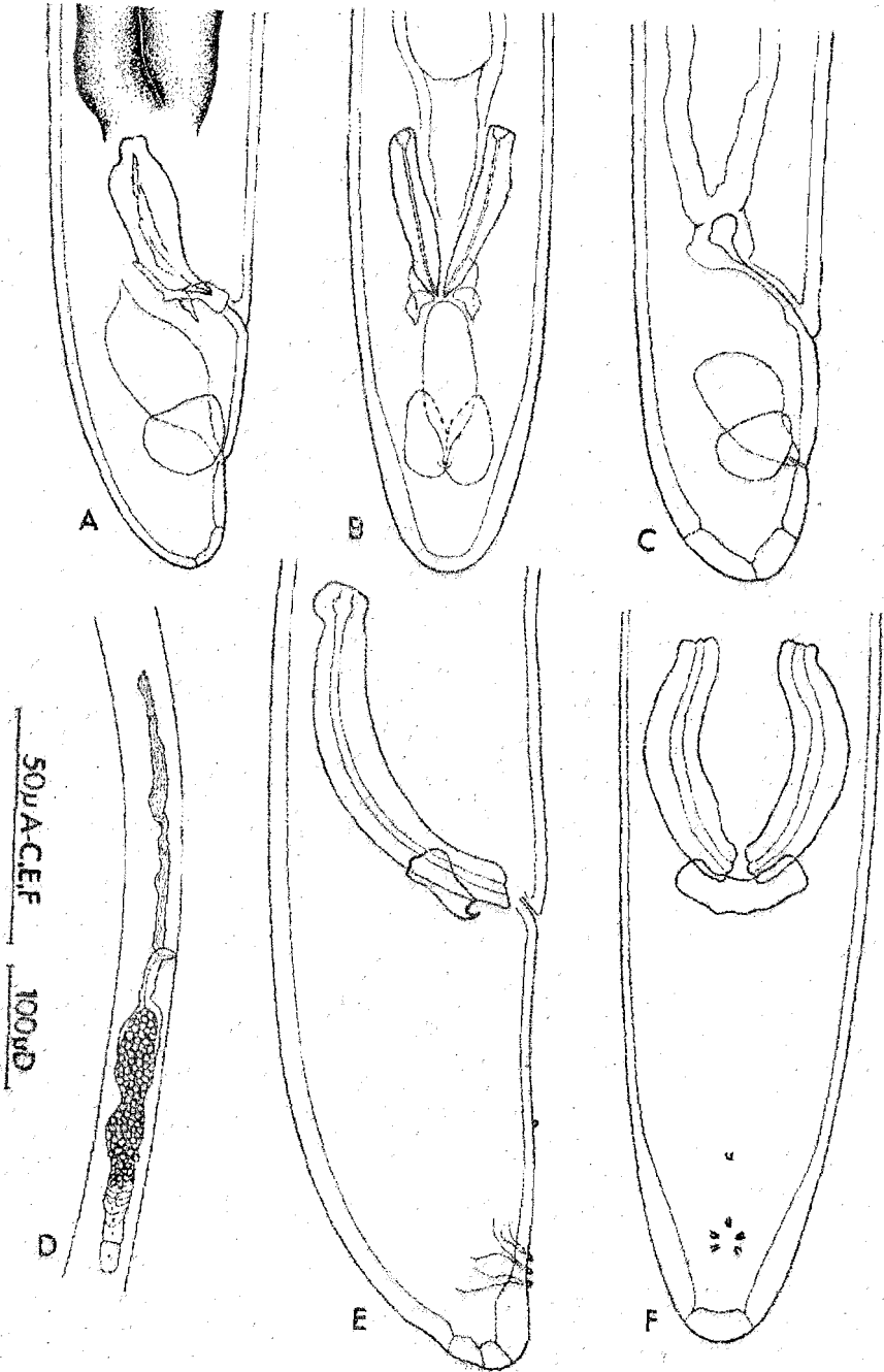
FIG. 4.— Trissonchulus litoralis n. sp. A. Male tail in lateral view. B. Male tail in ventral view. C. Female tail in lateral view. D. Female reproductive organs. Trissonchulus quinquepapillatus n. sp. E. Male tail in lateral view. F. Male tail in ventral view.
