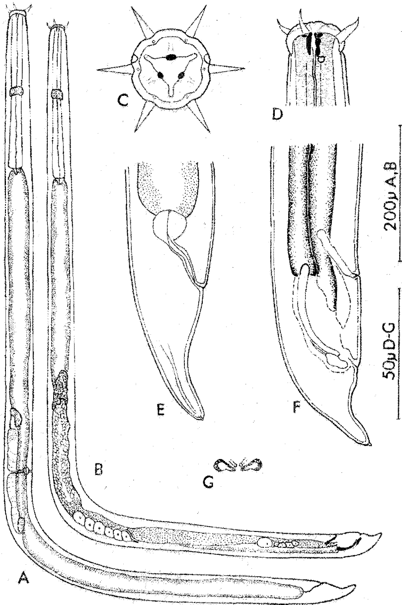
FIG. 4 A-G— Raamowhitia orca n. gen. et sp. A. Entire female. B. Entire male. C. In face view of head. D. Head region. E. Female tail. F. Lateral view of male tail region. G. Ventral view of distal end of spicules and gubernaculum.
