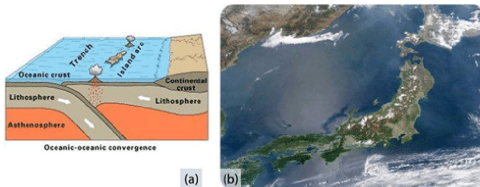
(a) Subduction of an ocean plate beneath an ocean plate results in a volcanic island arc, an ocean trench and many earthquakes. (b) Japan is an arc-shaped island arc composed of volcanoes off the Asian mainland, as seen in this satellite image.
