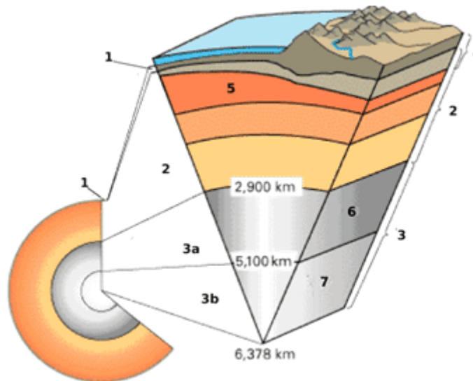
A cross section of Earth showing the following compositional layers: (1) crust (2) mantle (3a) outer core (3b) inner core and physical properties layers (4) lithosphere (5) asthenosphere (6) outer core (7) inner core.
