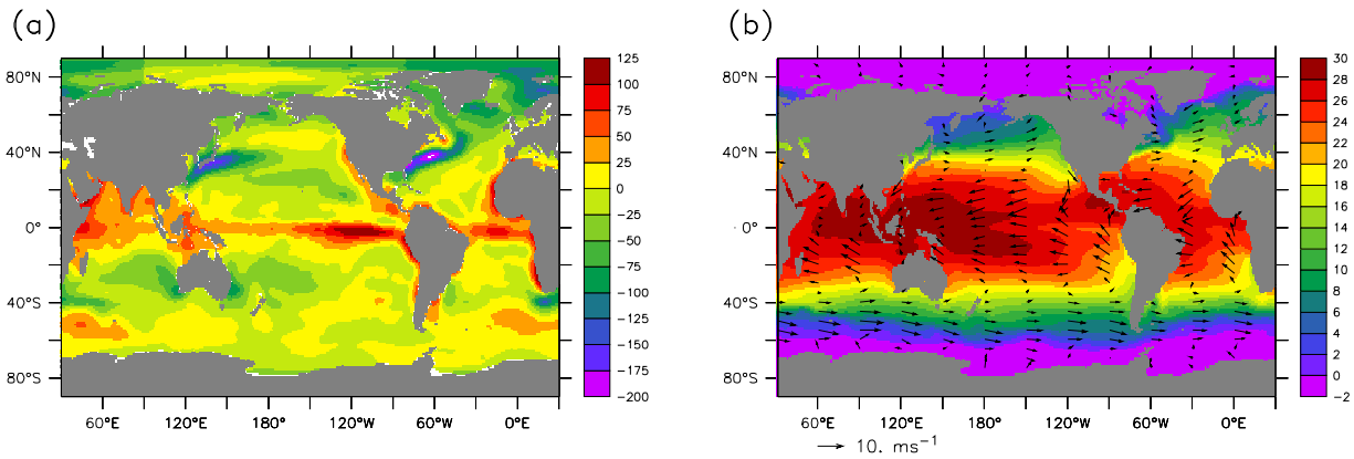
Figure 2. Mean climatologies of (a) net surface heat flux in units \text{Wm}^{-2} and, (b) sea surface temperature in units degrees Celsius, and surface winds in units \text{ms}^{-1} . Climatologies provided by da Silva et al. (1994). A positive net surface heat flux acts to warm the ocean.
