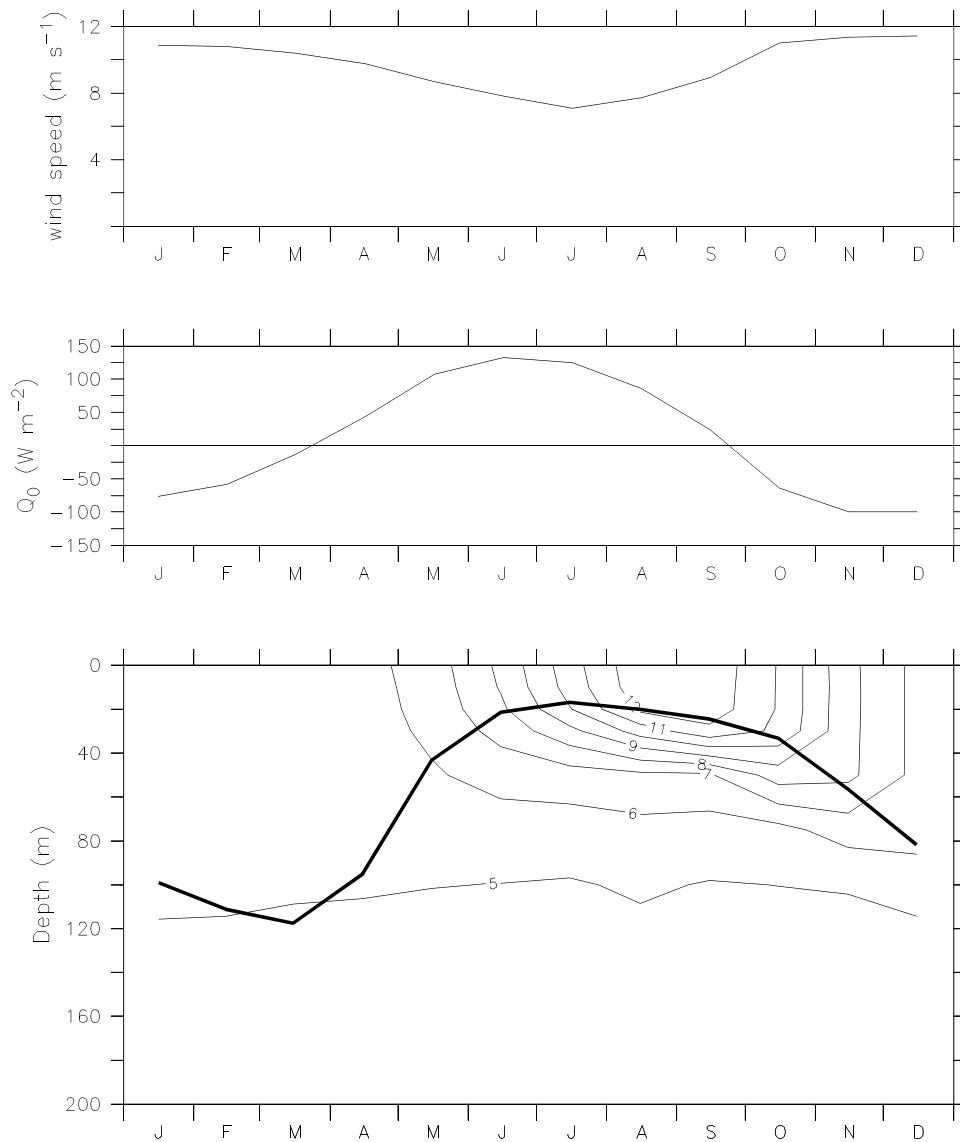
Figure 4. Seasonal climatologies at the ocean weather station PAPA in the north Pacific. (top panel) Wind speed, (middle panel) net surface heat flux, and (bottom panel) upper ocean temperature. The thick line represents the base of the ocean mixed layer defined as the depth where the temperature is 0.5^\circ\text{C} cooler than the surface temperature. Wind speed and net surface heat flux climatologies are from da Silva et al. (1994).
