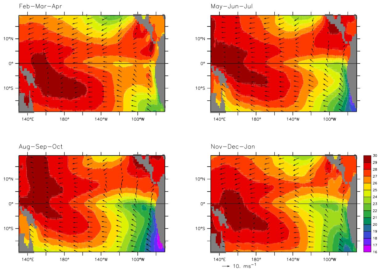
Figure 5. Tropical Pacific sea surface temperature and wind for the climatological (a) February-March-April, (b) May-June-July, (c) August-September-October, and (d) November-December-January. Winds are from da Silva et al. (1994). SSTs are from Reynolds and Smith (1994).
