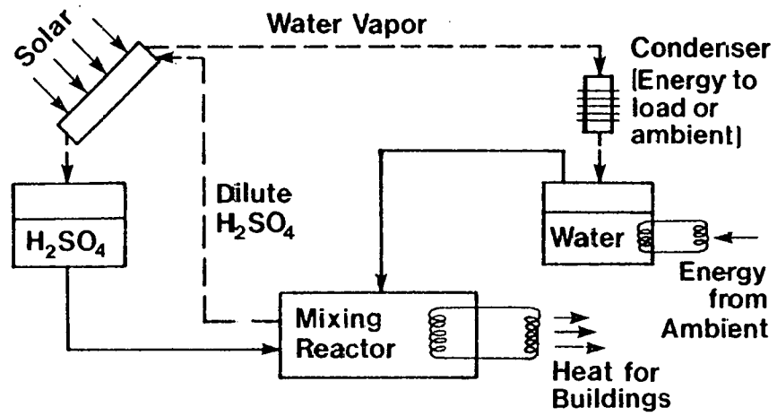
Figure 3-7. CHEMICAL HEAT PUMP STORAGE FOR SULFURIC ACID CONCENTRATION/ DILUTION WITH THE CHARGING CYCLE REPRESENTED BY DASHED LINES (---) AND THE DISCHARGING CYCLE BY SOLID LINES (-)
