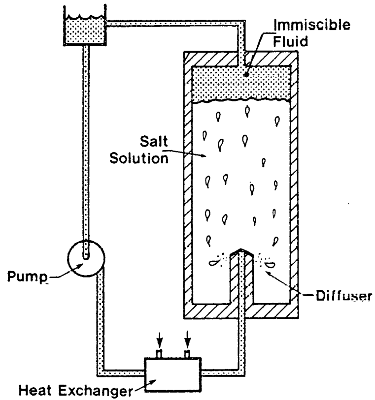
Figure 4-7. DIRECT CONTACT SYSTEM FOR HEAT TRANSFER BETWEEN THE LATENT HEAT STORAGE MEDIUM AND AN IMMISCIBLE FLUID [ 36 ]
