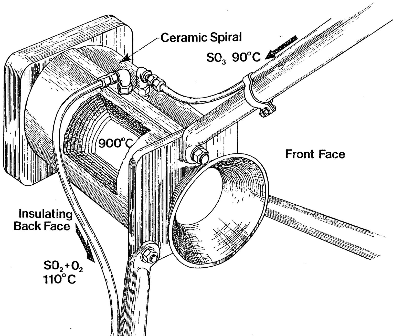
Figure 4-9. CAVIT/ CONVERTER-HEAT EXCHANGER FOR \text{SO}_3 DECOMPOSITION [41]
