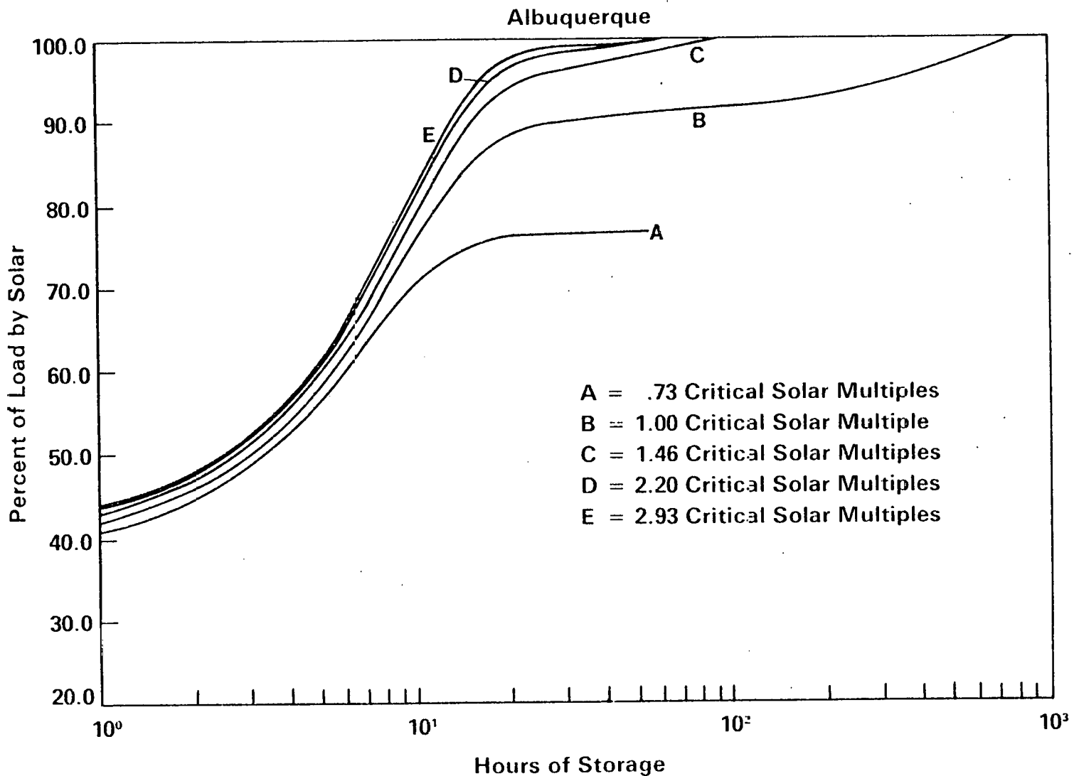
Figure 2-7. EFFECT OF STORAGE DURATION ON PERCENT ENERGY PROVIDED BY SOLAR FOR VARIOUS COLLECTOR ARRAY AREAS IN ALBUQUERQUE [7]
