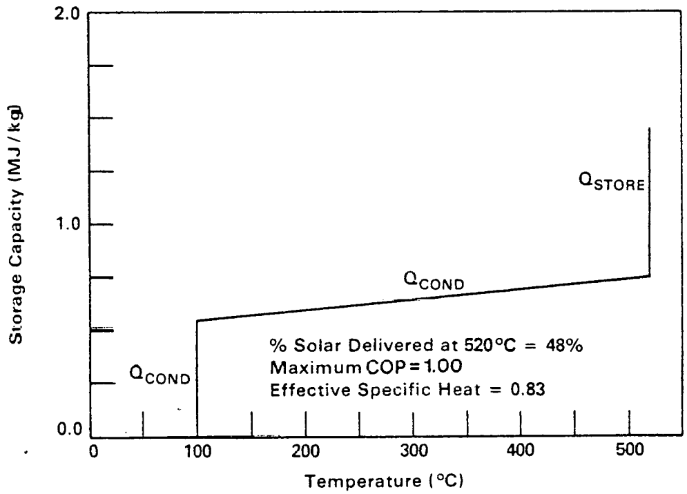
Figure 5-4. ENERGY RELEASED AS A FUNCTION OF TEMPERATURE FOR CALCIUM OXIDE/HYDROXIDE WITH MATERIALS STORED AT HIGH TEMPERATURES
