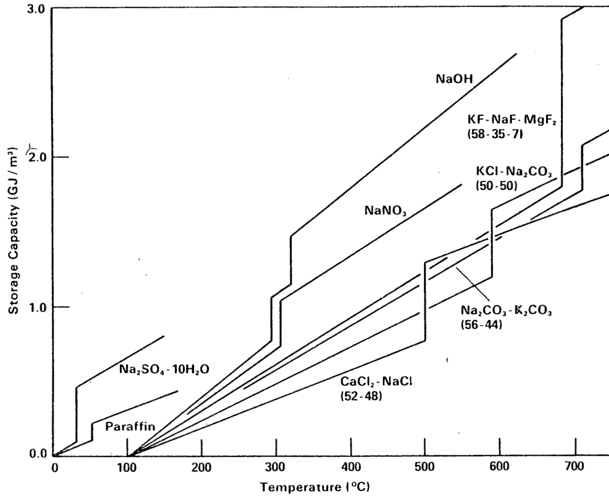
Figure 3-5. STORAGE CAPACITY PER UNIT VOLUME AS A FUNCTION OF TEMPERATURE FOR SELECTED LATENT HEAT STORAGE MATERIALS. THE MOLAR COMPOSITION OF MIXTURES ARE SHOWN IN PARENTHESIS
