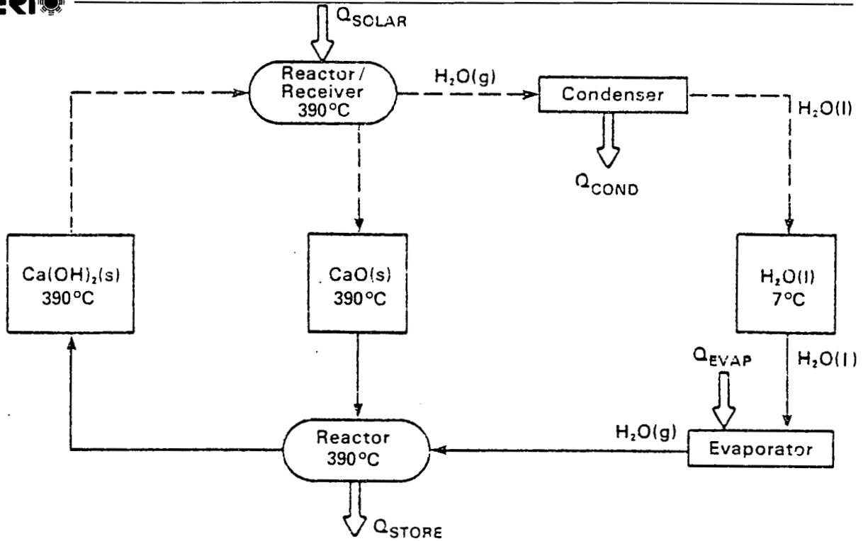
Figure 5-7. THERMAL ENERGY STORAGE SYSTEM BASED ON CALCIUM OXIDE/HYDROXIDE WITH SOLIDS STORED AT 390^{\circ}C AND WATER CONDENSED, STORED, AND VAPORIZED USING ATMOSPHERIC TEMPERATURES. THE CHARGING CYCLE IS SHOWN BY DASHED LINES AND THE DISCHARGING CYCLE IS SHOWN BY SOLID LINES
