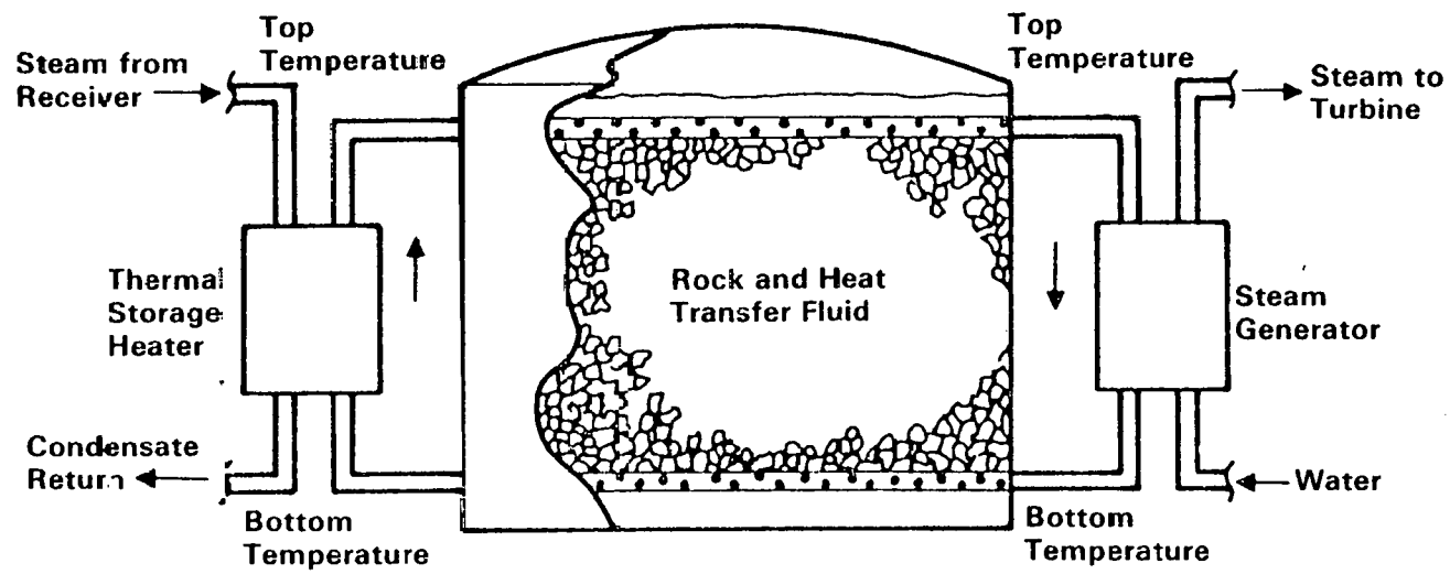
Figure 4-1. DUAL MEDIUM THERMAL STORAGE CONCEPT [17]
