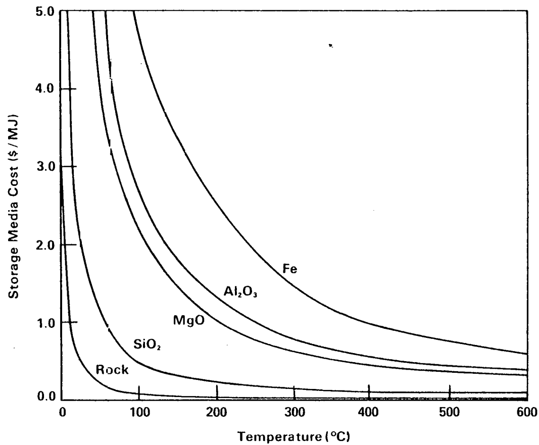
Figure 3-4. STORAGE MEDIA COSTS IN DOLLARS PER UNIT ENERGY STORED AS A FUNCTION OF TEMPERATURE FOR SELECTED SOLID SENSIBLE HEAT STORAGE MEDIA
