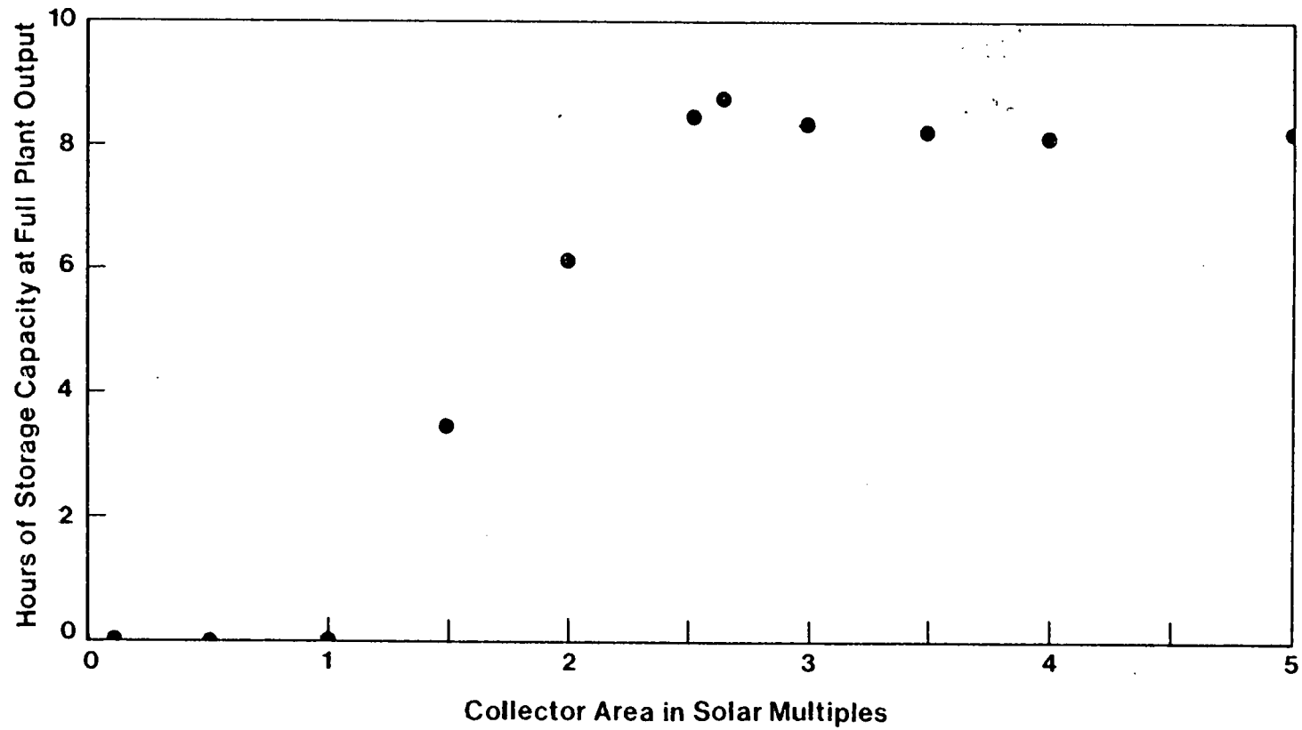
Figure 2-6. STORAGE CAPACITY FOR THE HYBRID ELECTRIC POWER PLANTS OF FIGURE 2-5 AS A FUNCTION OF THE COLLECTOR MIRROR AREA IN SOLAR MULTIPLES. [7]
