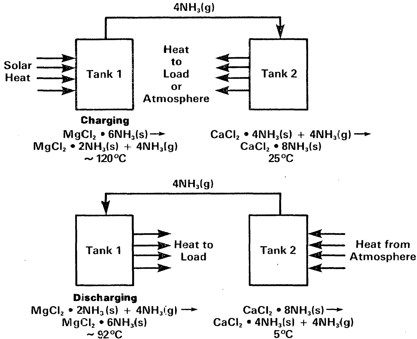
Figure 3-8. CHEMICAL HEAT PUMP STORAGE BY AMMONIATED SALT PAIRS FOR HEATING APPLICATIONS WITH THE UPPER DIAGRAM FOR CHARGING STORAGE AND THE LOWER FOR DISCHARGING
