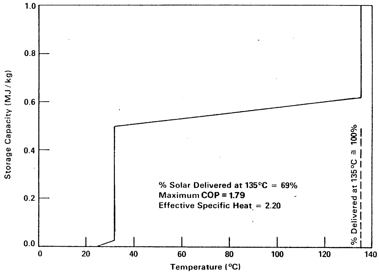
Figure 5-14. ENERGY RELEASED AS A FUNCTION OF TEMPERATURE FOR AMMONIATED SALTS IN THE CHEMICAL HEAT PUMP MODE WITH ALL MATERIALS STORED AT 25°C
