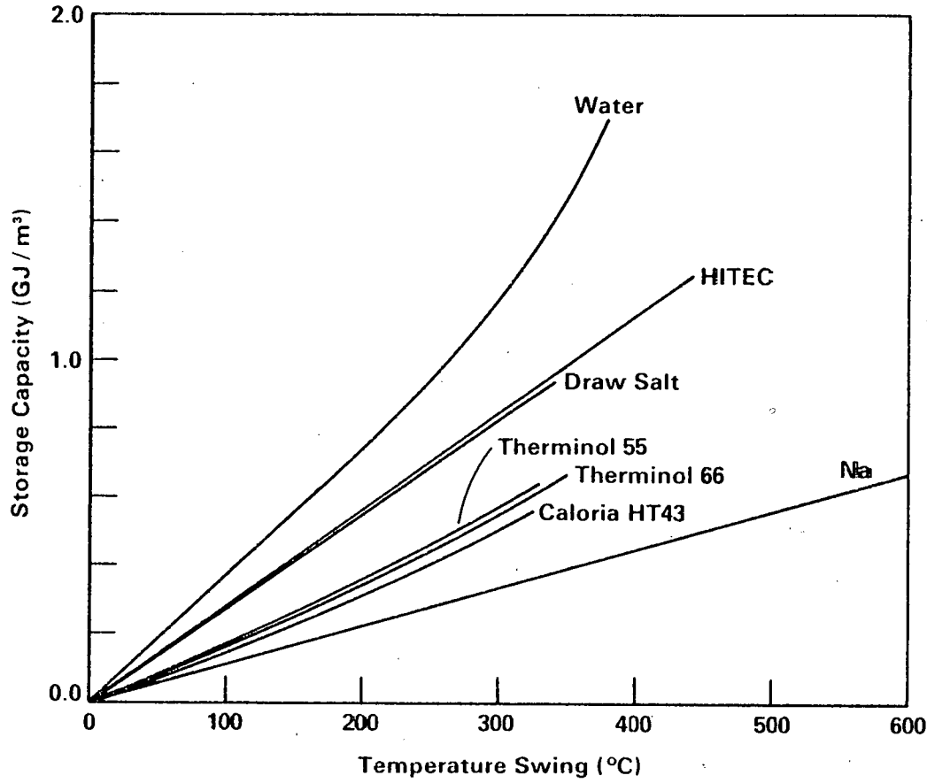
Figure 3-1. STORAGE CAPACITY PER UNIT VOLUME AS A FUNCTION OF TEMPERATURE SWING FOR SELECTED LIQUID SENSIBLE HEAT STORAGE MEDIA
