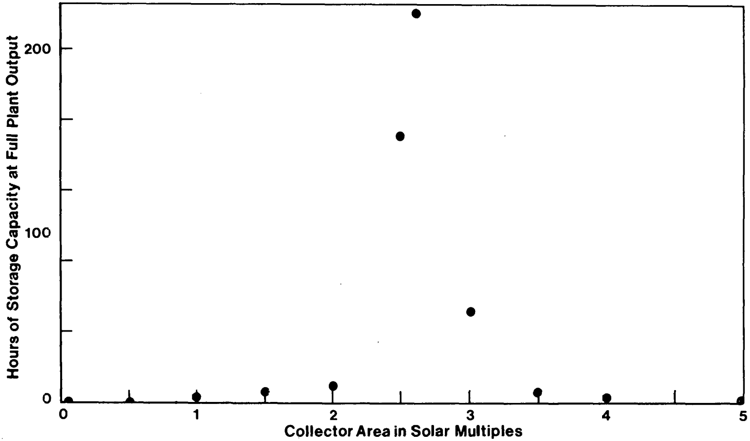
Figure 2-4. STORAGE CAPACITY FOR THE AUTONOMOUS ELECTRIC POWER PLANT OF FIGURE 2-3 AS A FUNCTION OF THE COLLECTOR MIRROR AREA IN SOLAR MULTIPLES [7]
