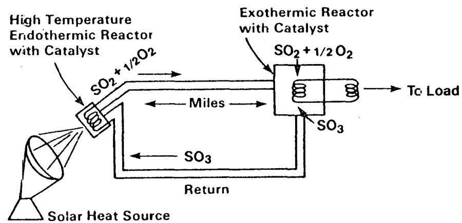
Figure 3-11. TRANSMISSION OF THERMAL ENERGY BY THE THERMOCHEMICAL PIPELINE SULFUR TRIOXIDE REACTION
