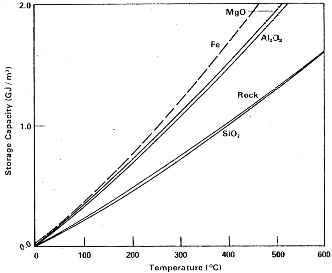
Figure 3-3. STORAGE CAPACITY PER UNIT VOLUME AS A FUNCTION OF TEMPERATURE FOR SELECTED SOLID SENSIBLE HEAT STORAGE MEDIA
