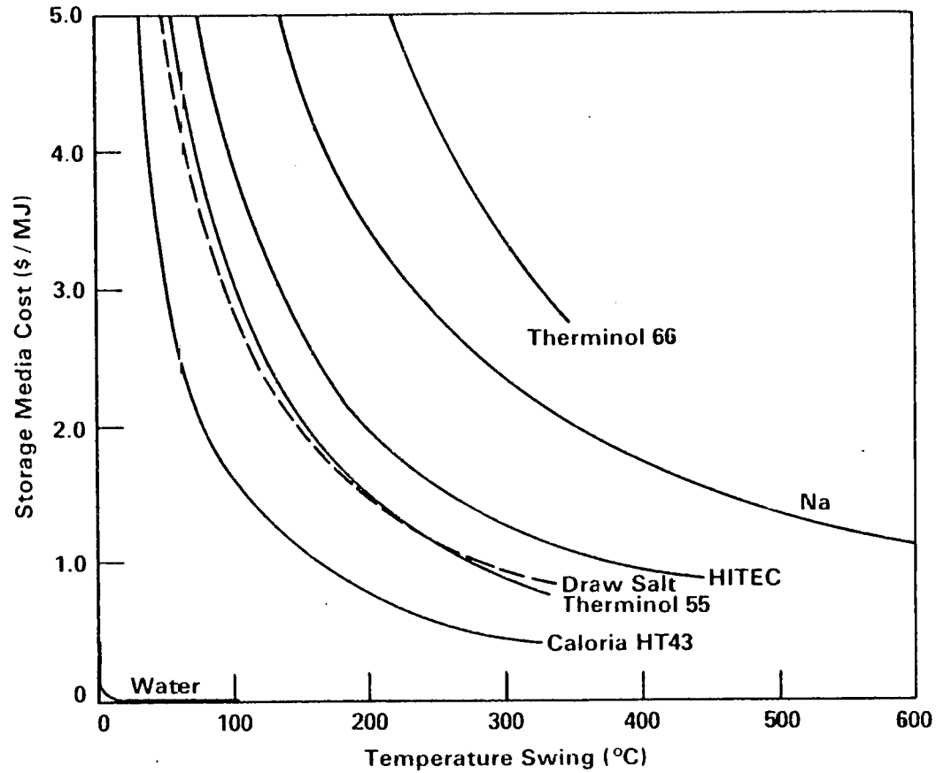
Figure 3-2. STORAGE MEDIA COSTS IN DOLLARS PER UNIT ENERGY STORED AS A FUNCTION OF TEMPERATURE SWING FOR SELECTED LIQUID SENSIBLE HEAT STORAGE MEDIA
