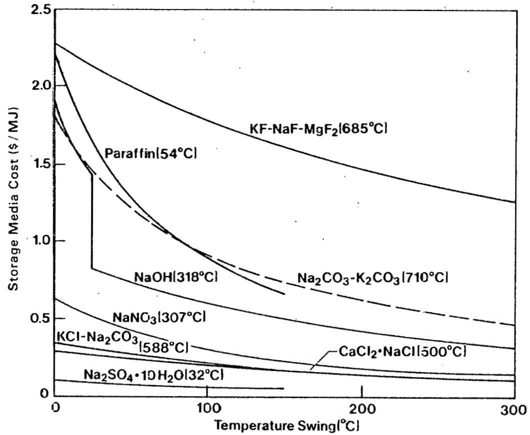
Figure 3-6. STORAGE MEDIA COSTS IN DOLLARS PER UNIT ENERGY STORED AS A FUNCTION OF TEMPERATURE SWING FOR SELECTED LATENT HEAT STORAGE MATERIALS. THE FUSION TEMPERATURE IS IN PARENTHESES
