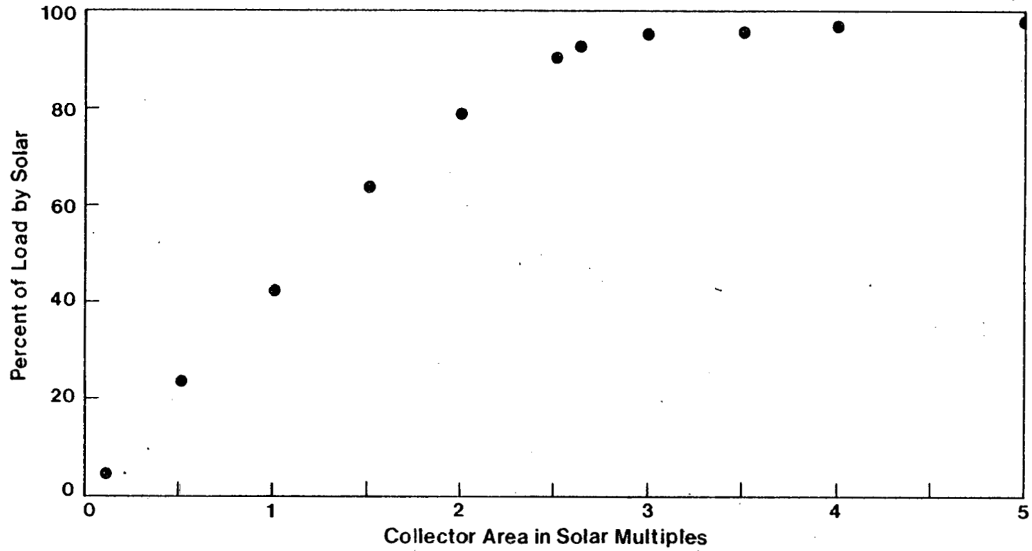
Figure 2-5. PERCENTAGE OF A HYBRID ELECTRIC POWER PLANT LOAD SUPPLIED BY SOLAR AS A FUNCTION OF COLLECTOR MIRROR AREA IN SOLAR MULTIPLES [7]
