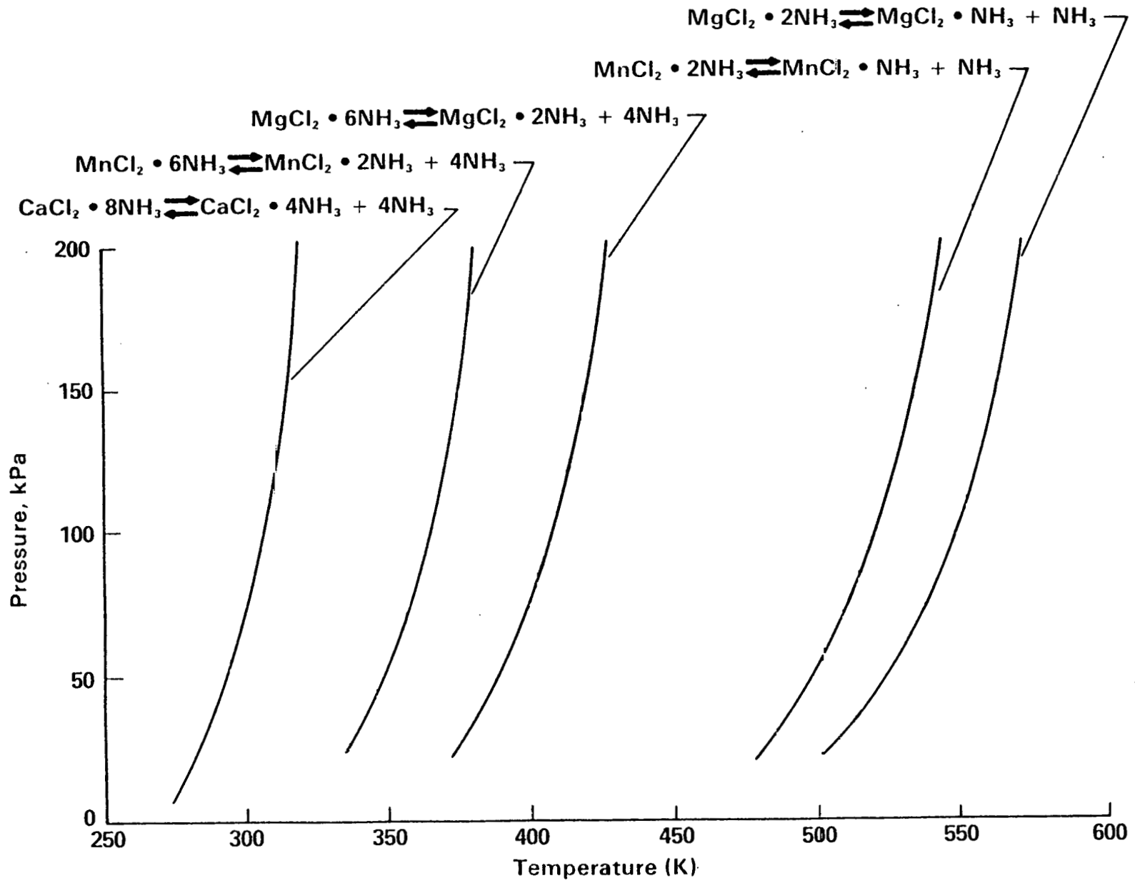
Figure 3-9. EQUILIBRIUM PRESSURES AS A FUNCTION OF TEMPERATURE FOR A VARIETY OF AMMONIATED SALTS [31]
