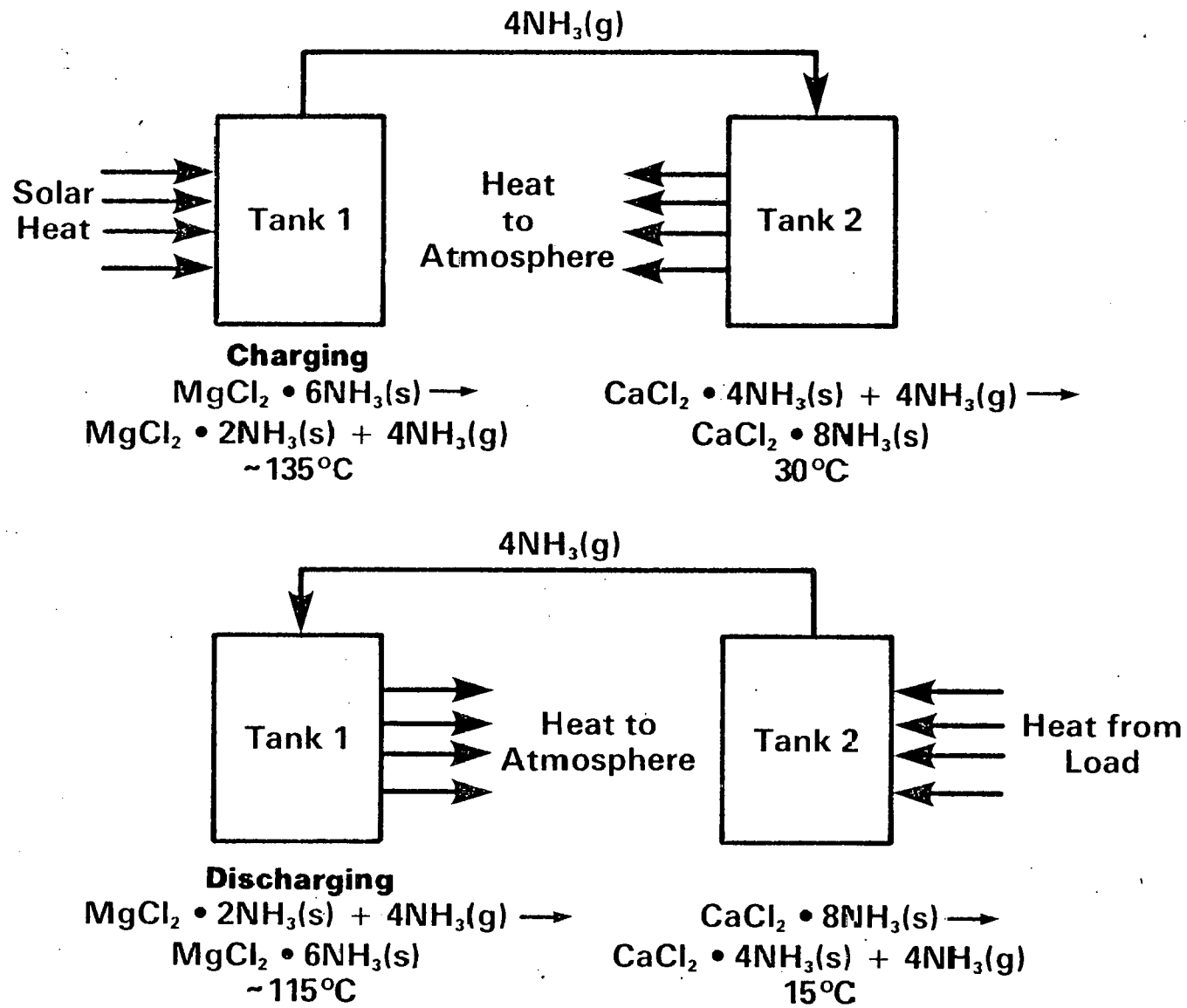
Figure 3-10. CHEMICAL HEAT PUMP STORAGE BY AMMONIATED SALT PAIRS FOR COOLING APPLICATIONS WITH THE UPPER DIAGRAM FOR CHARGING STORAGE AND THE LOWER FOR DISCHARGING.
