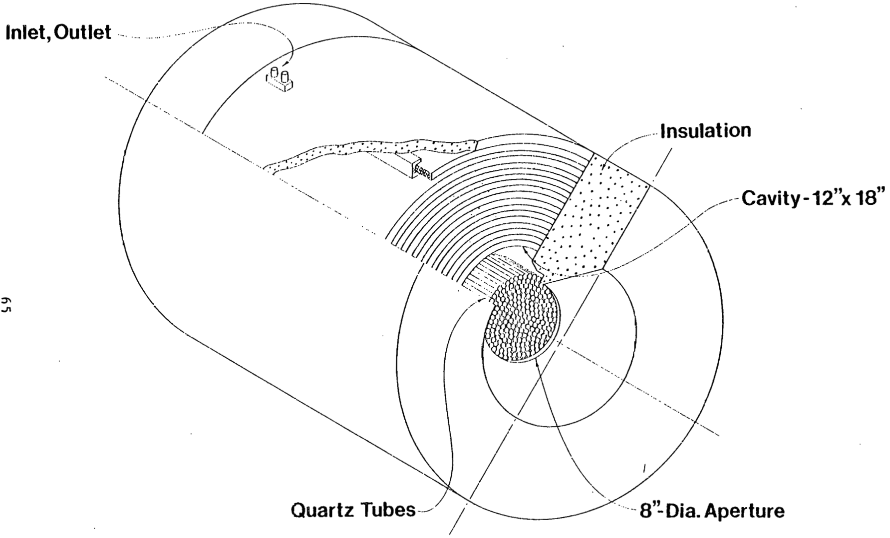
Figure 4-10. DETAILS OF CONVERTER-HEAT EXCHANGER CAVITY FOR SO 3 DECOMPOSITION [41]
