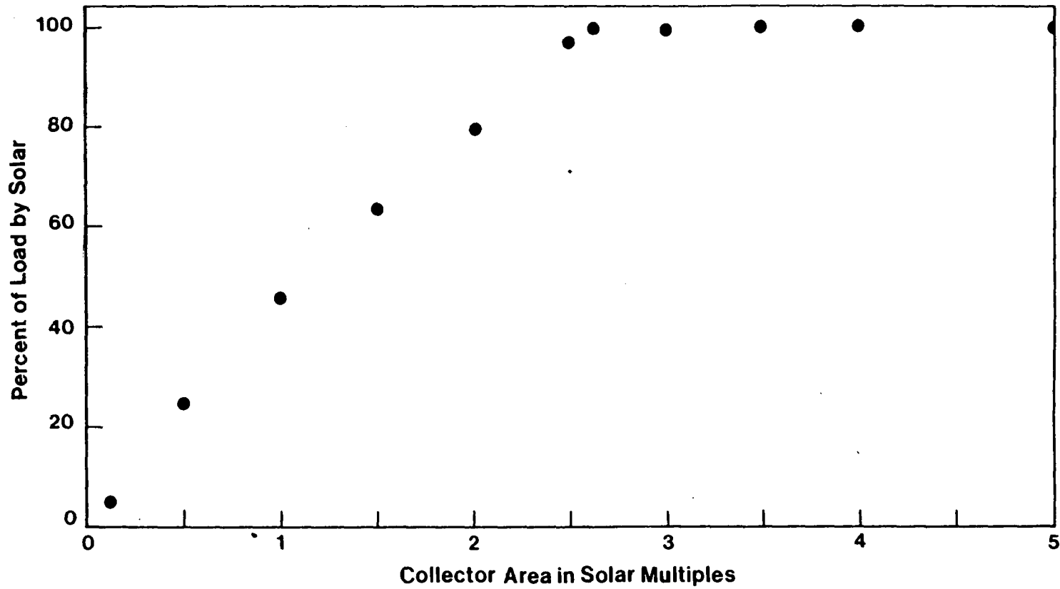
Figure 2-3. PERCENTAGE OF AN AUTONOMOUS ELECTRIC POWER PLANT LOAD SUPPLIED BY SOLAR AS A FUNCTION OF THE COLLECTOR MIRROR AREA IN SOLAR MULTIPLES. A MINIMUM COLLECTOR AREA OF 2.63 SOLAR MULTIPLES IS REQUIRED FOR AUTONOMOUS OPERATION [7]
