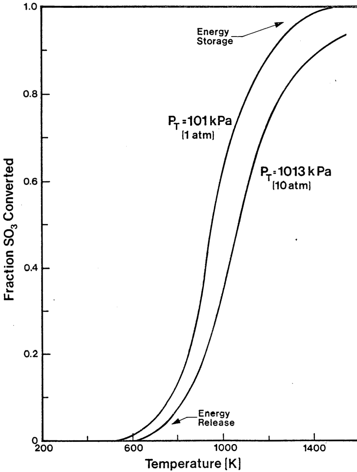
Figure 5-1. EQUILIBRIUM CONVERSION OF SO 3 AS A FUNCTION OF TEMPERATURE [23]
