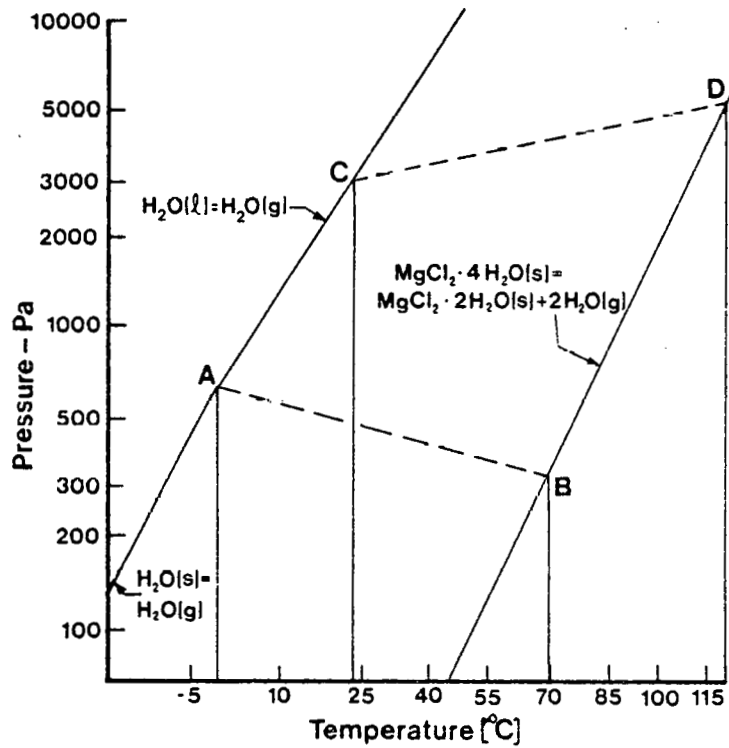
Figure 4-8. EQUILIBRIUM PRESSURE-TEMPERATURE DIAGRAM FOR HYDRATES OF MAGNESIUM CHLORIDE AND WATER [40]
