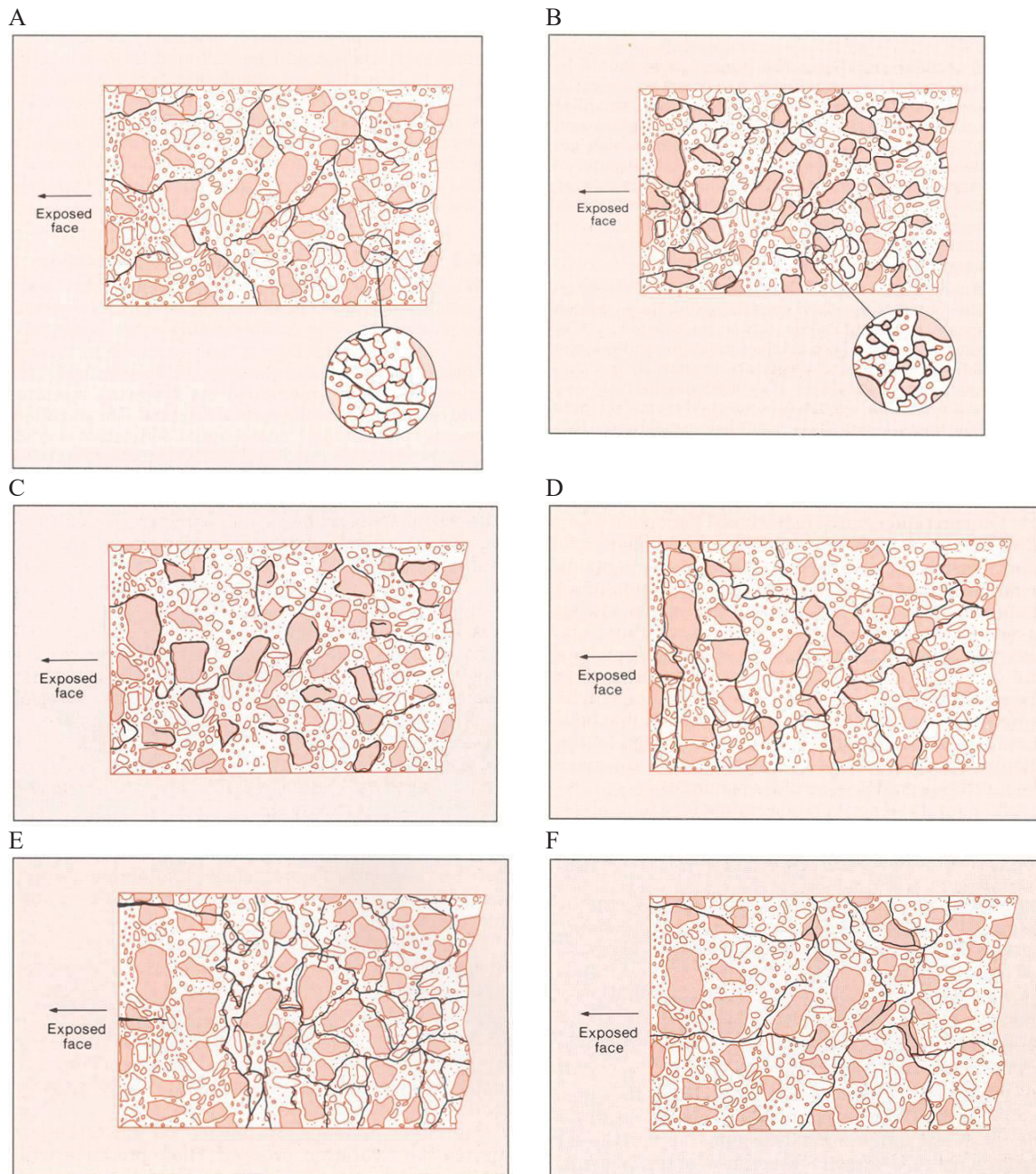
Figure C2. From BCA (1992) (Note: This was taken directly from the BCA publication and should be for internal use / discussion only at this stage, i.e. until copyright issues be resolved) (A). Internal crack pattern which can be induced by drying shrinkage. (B). Internal crack pattern which can be caused by internal sulfate attack for delayed ettringite formation (DEF), or from sulfates derived from the aggregates. (C). Internal crack pattern which can be induced by shrinkage of the coarse aggregate. (D). Internal crack pattern which can be induced by frost attack. (E). Internal crack pattern which can be caused by ASR: reactive silica in the sand fraction. (F). Internal crack pattern which can be caused by ASR: reactive silica in the coarse aggregate.
