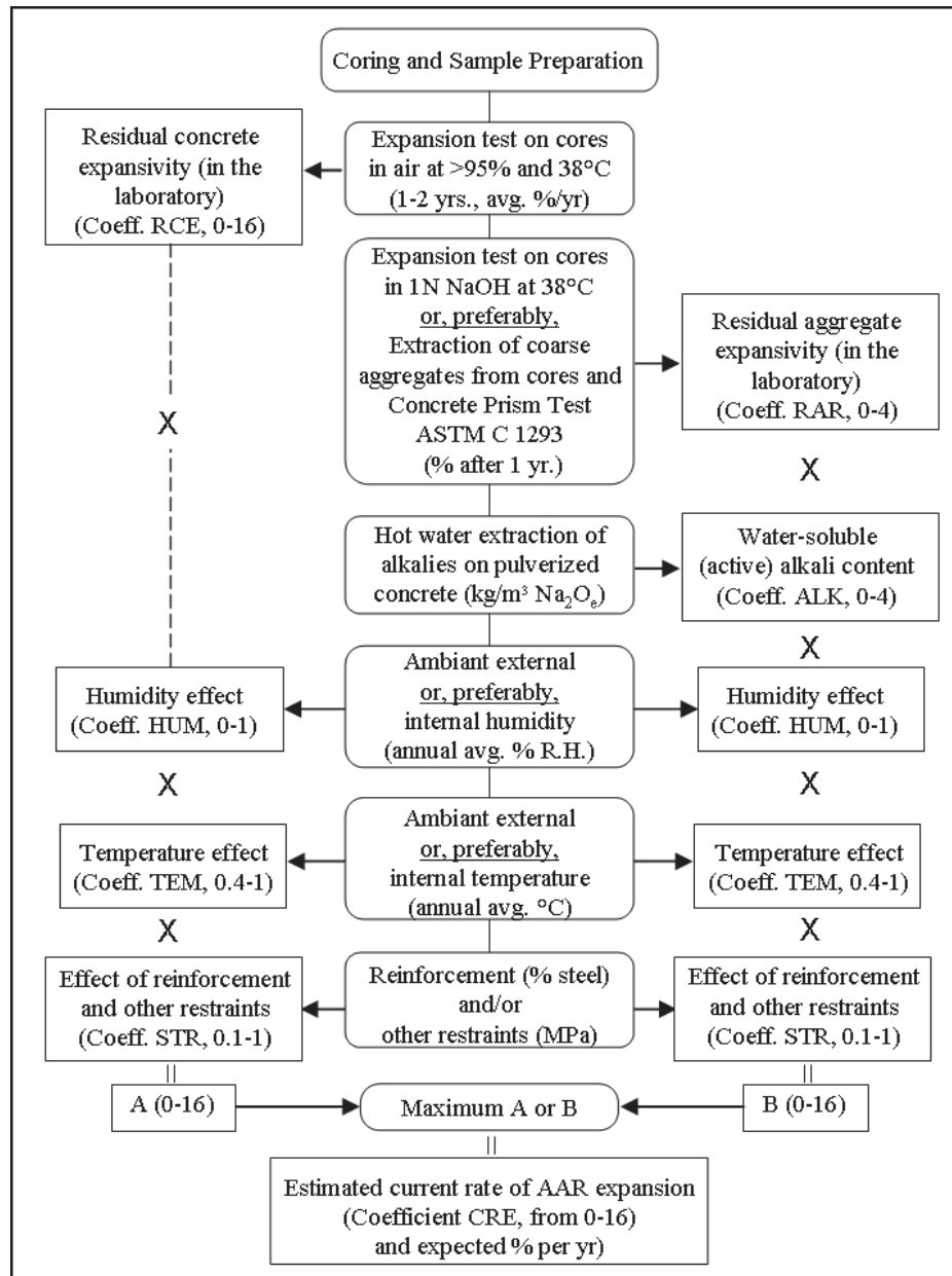
Figure 11. Laboratory assessment of the current rate of ASR expansion in concrete members in service either already affected by ASR or not.
