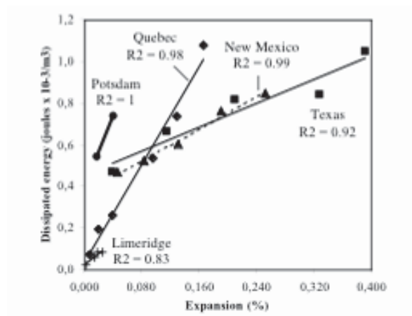
Figure E3. Linear relationships between the energy dissipated during the first load/unload cycle of the modified SDT and the expansion of concrete cylinders made with different coarse (Québec, New Mexico, Potsdam, Limeridge) or fine (Texas) aggregates susceptible to ASR. (After Smaoui et al. 2004a, 2004c).
