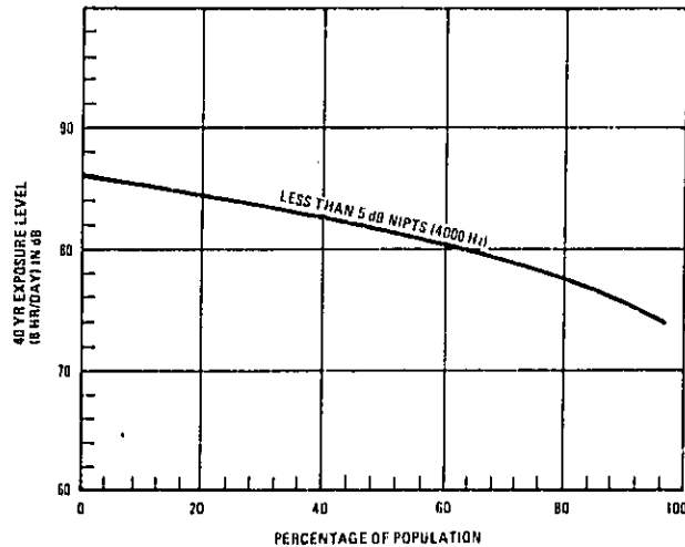
Figure 3. Percentage of Exposed Population That Will Incur No More Than 5 dB NIPTS Shown as a Function of Exposure Level. Population Ranked by Decreasing Ability to Hear at 4000 Hz. (See Appendix C for Rationale).
