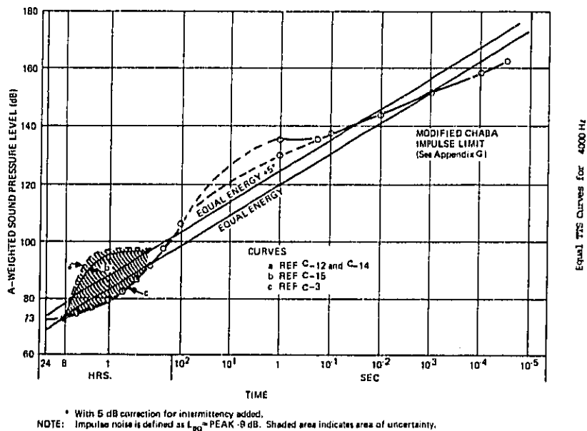
Figure C-6. Equal TTS Curves for 4000 Hz
