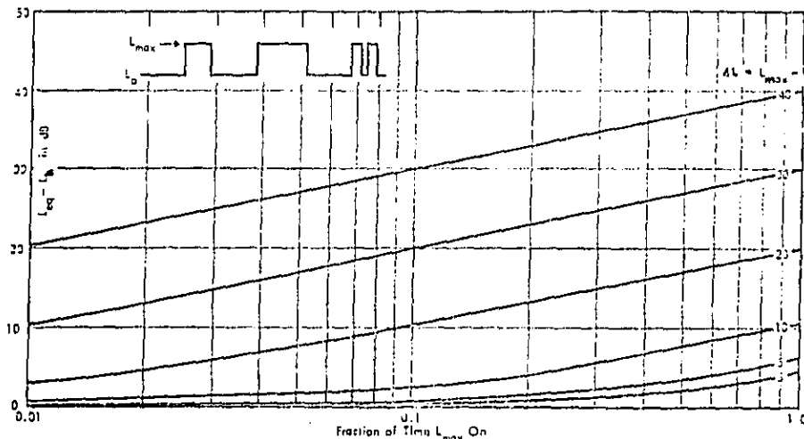
Figure A-1. L_{\text{eq}} for Intermittent L_{\max} Added to L_b A-25
