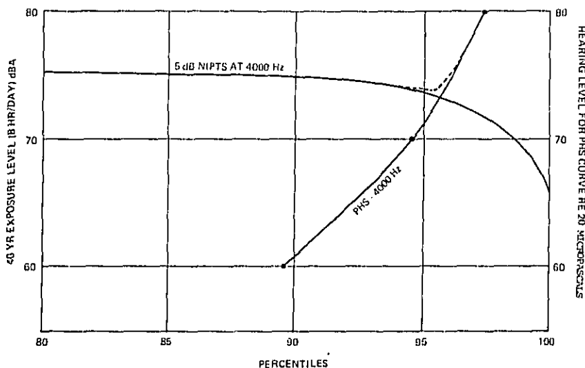
Figure C-3. Exposure Level and Hearing Level as a Function of Population Percentile, Showing the 5 dB NIPTS Curve Merging with the PHS 4000 Hz Curve
