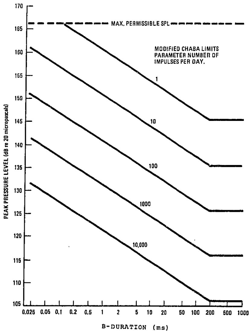
Figure 4. Set of Modified CHABA Limits for Daily Exposure to Impulse Noises Having B-Durations in the Range 25 Microseconds to 1 Second. (Parameter: number (N) of impulses per daily exposure. Criterion: NIPTS not to exceed 5 dB at 4 kHz in more than 10% of people.)
