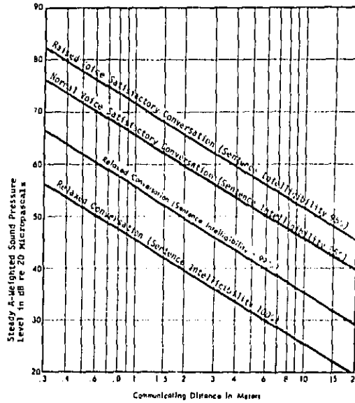
Figure D-2. Maximum Distances Outdoors Over Which Conversation is Considered to be Satisfactorily Intelligible in Steady Noise. D-1, D-2
