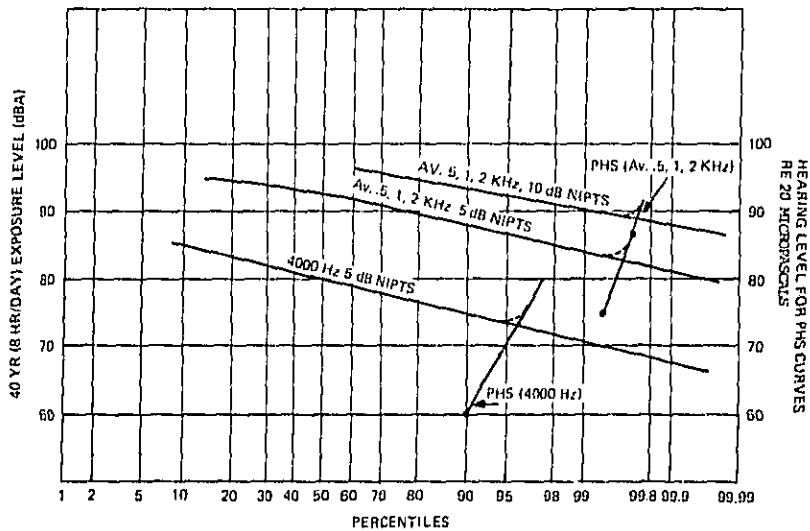
Figure C-4. Exposure Level and Hearing Level as a Function of Population Percent Showing Merging of Different NIPTS Curves with PHS Curves
