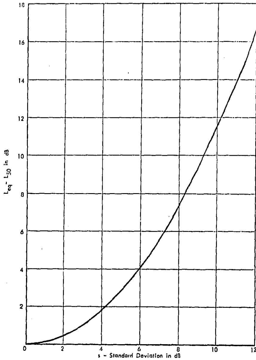
Figure A-4. Difference Between L_{eq} and L_{50} for a Normal Distribution Having Standard Deviation of s , A-25 (See Equation A-14).
