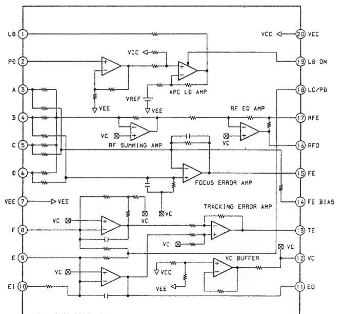
IC103 CXA1821M
