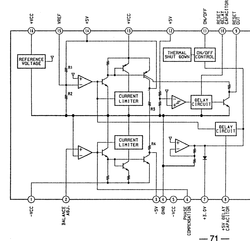
IC671 M5294P
