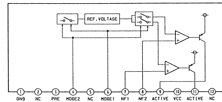
IC541 BA3960
