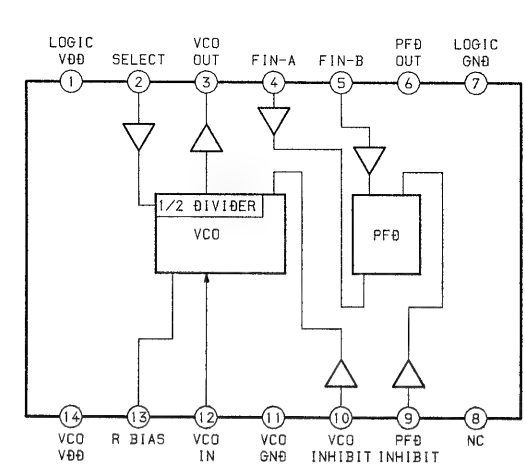
IC401 TLC2932IPW-E20
