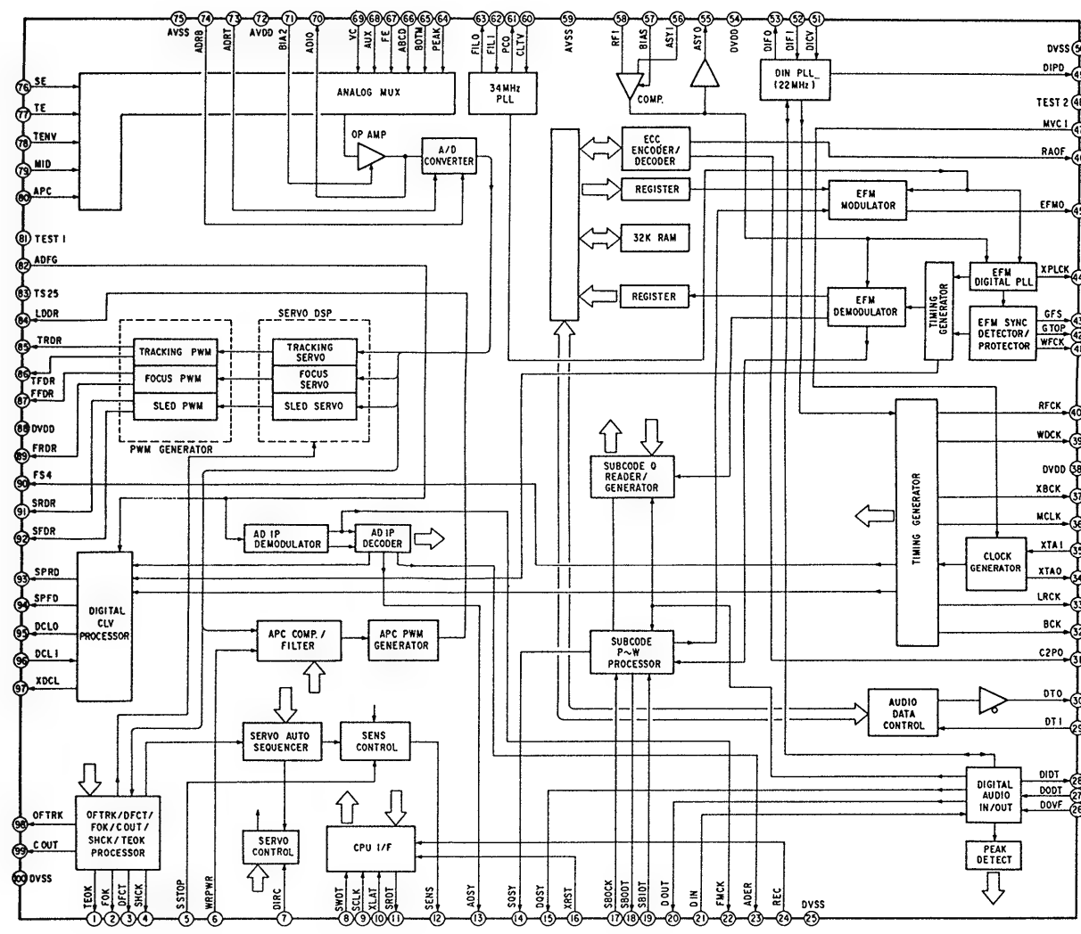
IC121 CXD2535BR
