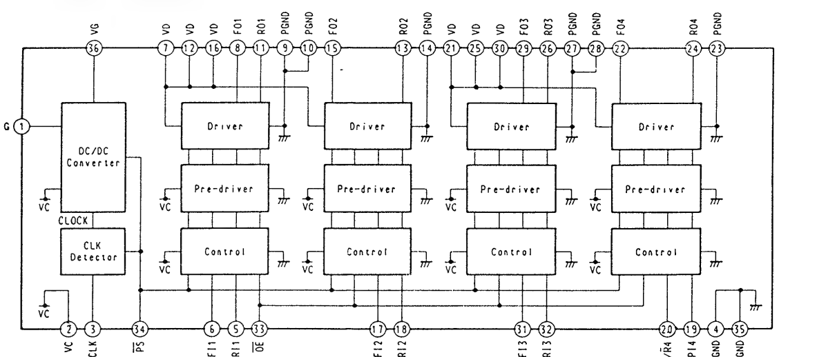
IC151 MPC17A38VMEL
