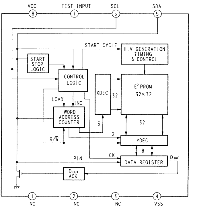
IC171 X24C01S
