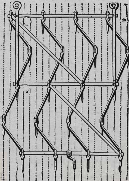
Central Draught 4-Beam Harrow.
