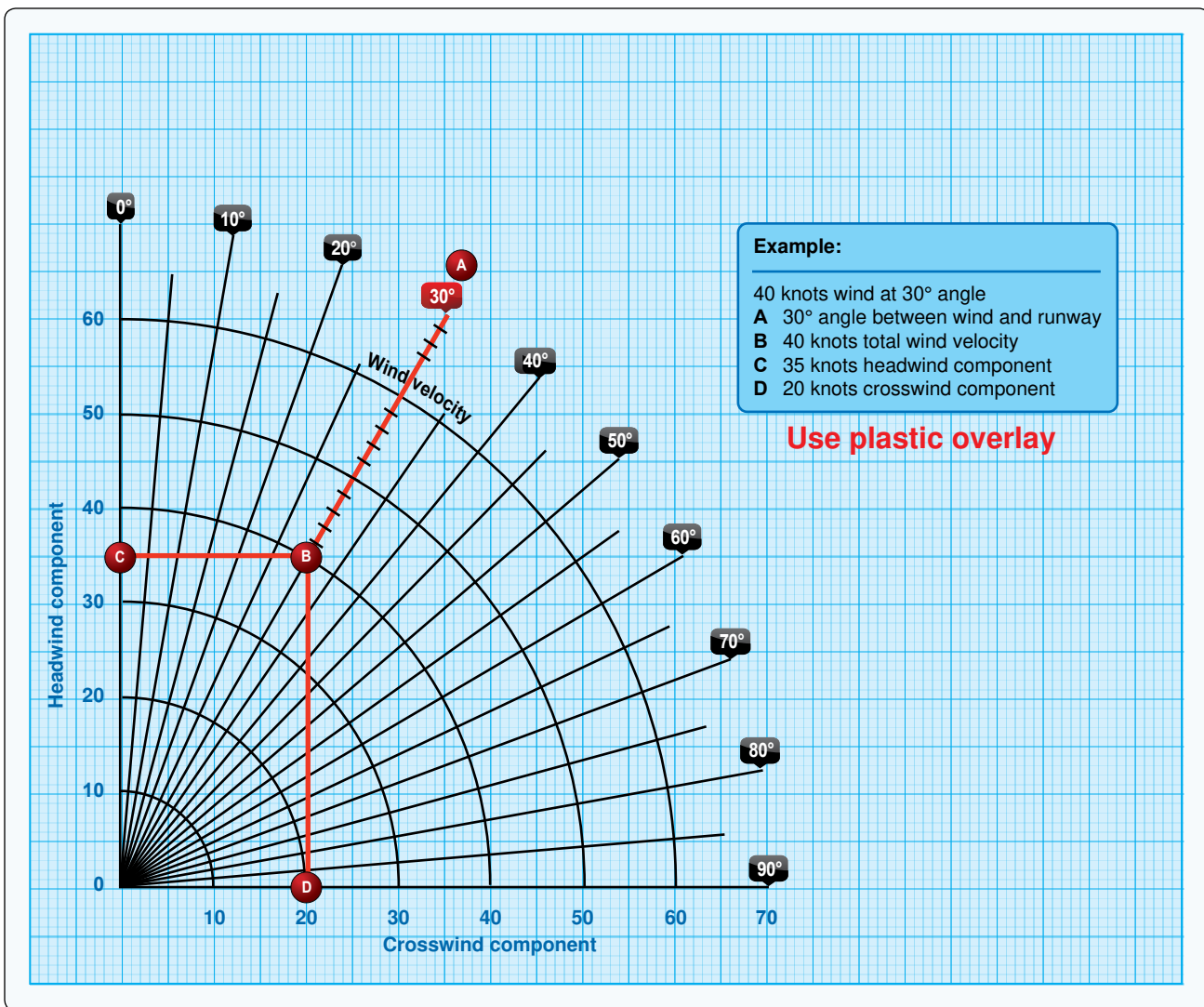
FIGURE 36.—Crosswind Component Graph.
