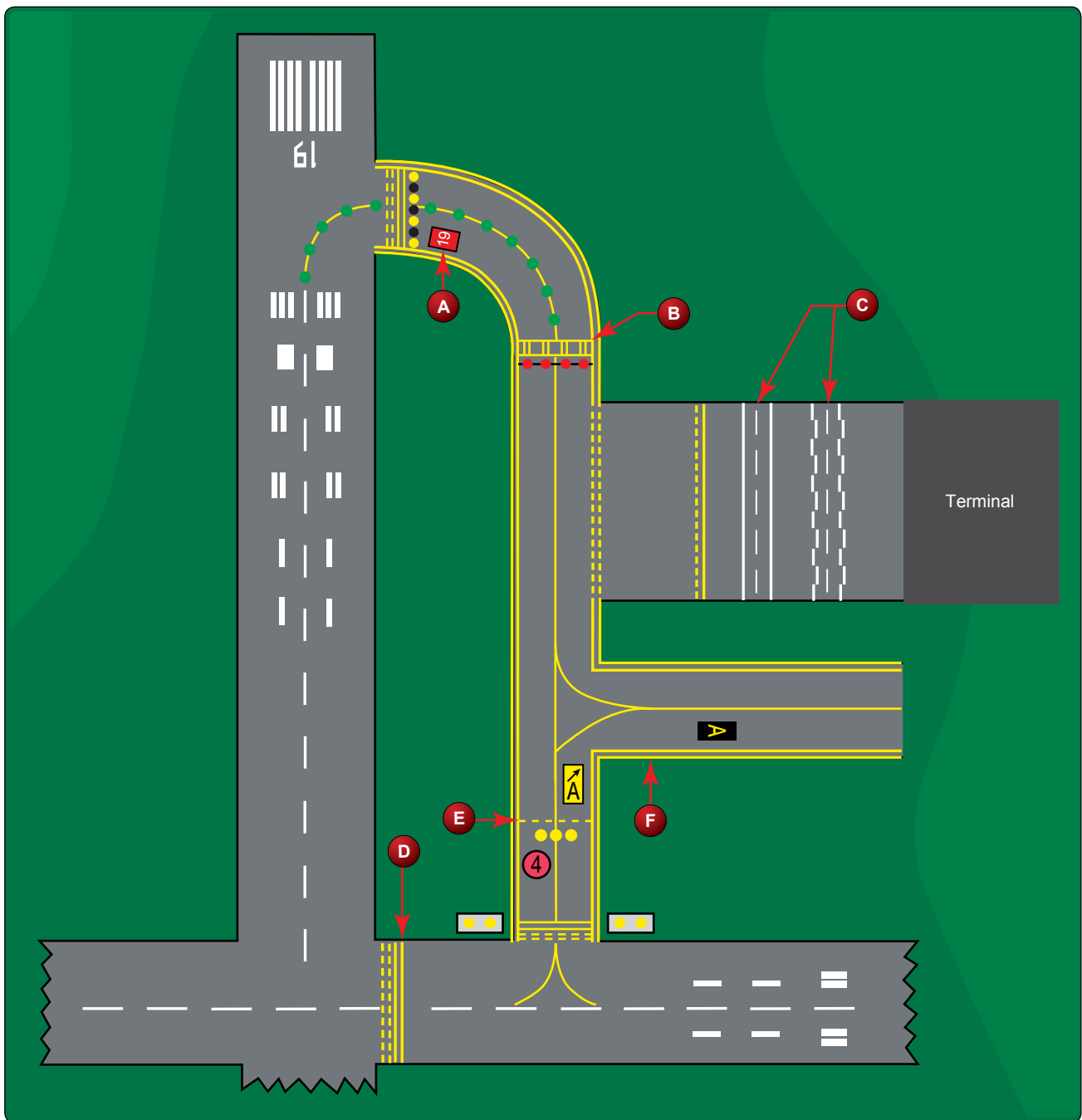
FIGURE 64.—Airport Markings.
