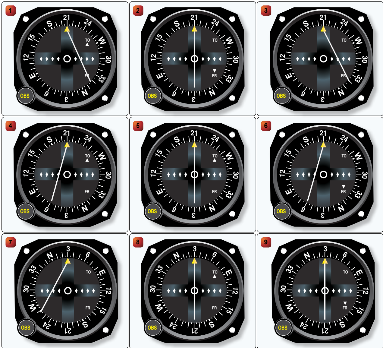
FIGURE 28.—VOR.
