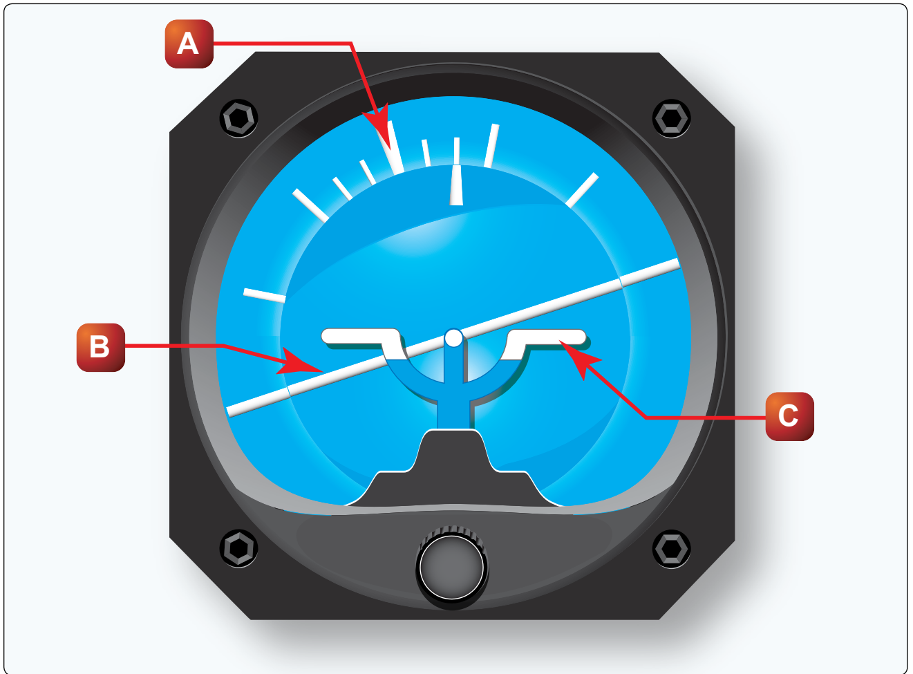
FIGURE 7.—Attitude Indicator.
