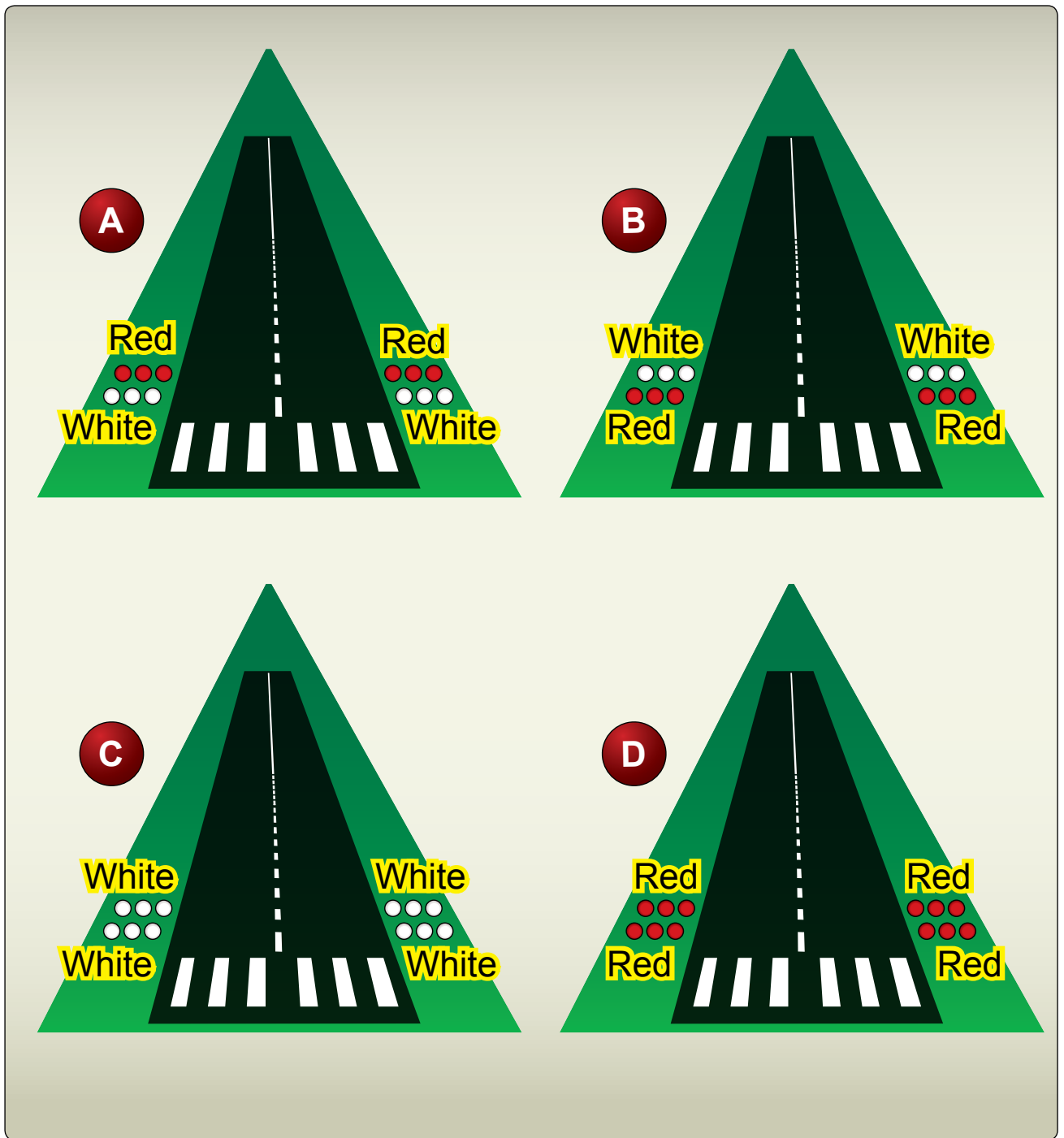
FIGURE 47.—VASI Illustrations.
