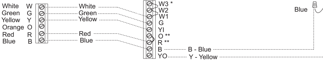
Comfort Control
