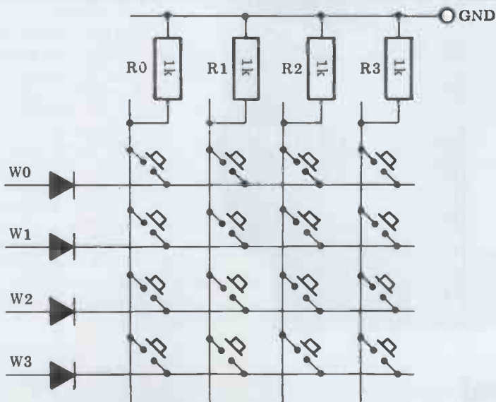
Fig 3 software polled Hex Keypad. D = IN914 or similar. W0 = channel 0 of output port = pin 1 of WRITE plug etc. R0 = channel 0 of input port = pin 1 of READ plug etc. Connect the ground on each resistor to pin 9 of the READ plug.
