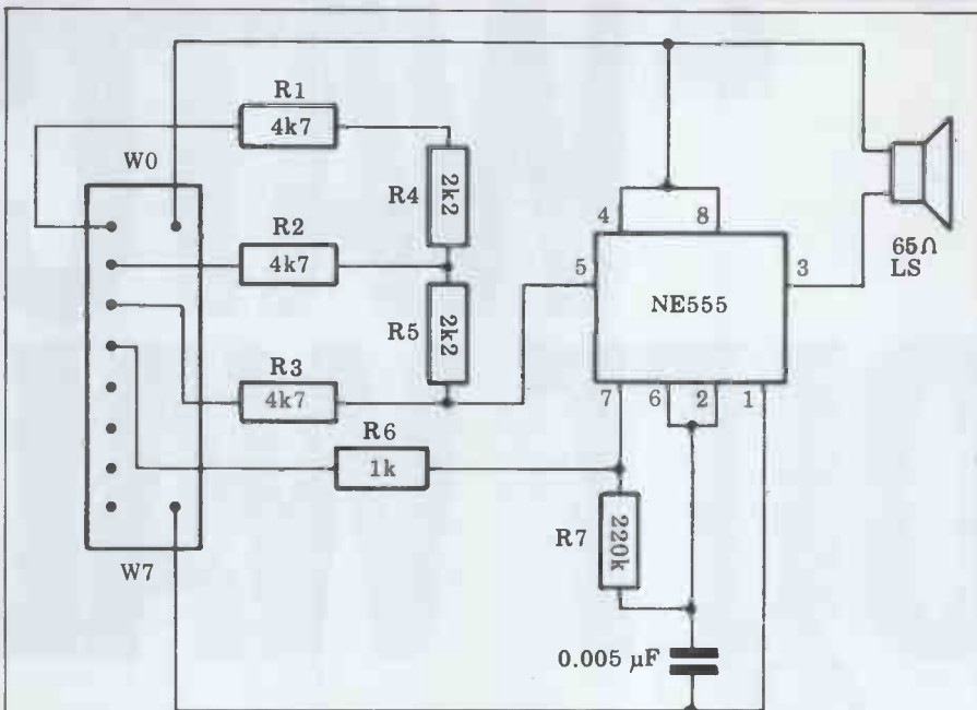
Fig 2 Hardwired audio generator. For accurate conversion, R1, R2 & R3 should be 4k 1% and R4 & R5 should be 2k 1%.
