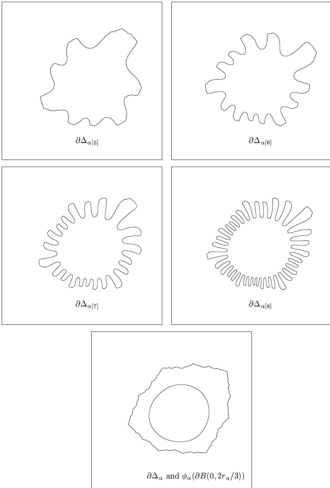
FIGURE 3. Some boundaries of Siegel disks for a sequence \alpha[n] .
