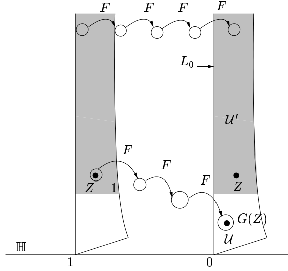
FIGURE 4. The regions \mathcal{U} , \mathcal{U}' and the map G : \mathcal{U}' \rightarrow \mathcal{U} .
