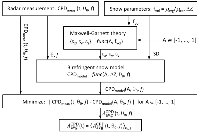
Figure 10. Processing chain used to estimate the average anisotropy of the snow pack, A_{\text{avg}}^{\text{CPD}} . The anisotropy can be estimated from the measured CPD, by minimizing the difference between modeled and measured data with respect to A if snow depth \Delta Z and the ice volume fraction f_{\text{vol}} are known. The anisotropy A_{\text{avg}}^{\text{CPD}}(t, \theta_0, f) was calculated independently for all incidence angles, \theta_0 , and frequencies, f , and the results were averaged to obtain A_{\text{avg}}^{\text{CPD}}(t) .
