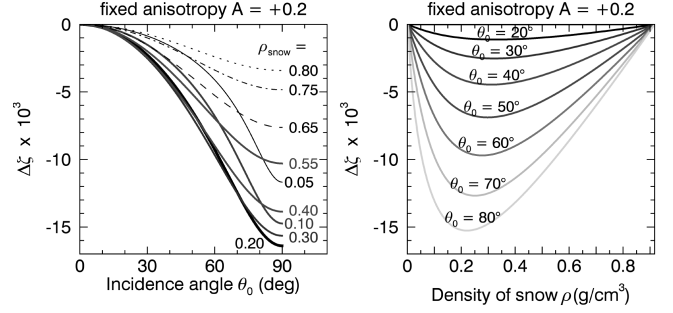
Figure 3. The specific path length difference \Delta\zeta , expected between vertically and horizontally polarized microwaves according to (Eq. 22), is plotted for snow with horizontally aligned oblate ice grains ( A = +0.2 ) over incidence angle (left), and snow density (right).
