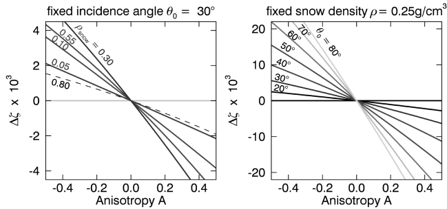
Figure 4. The specific path length difference \Delta\zeta , according to (Eq. 22), plotted over anisotropy for different snow densities but fixed incidence angle, \theta_0 = 30^\circ , (left) and for different incidence angles but fixed snow density, \rho = 0.25 \text{ g cm}^{-3} , (right).
