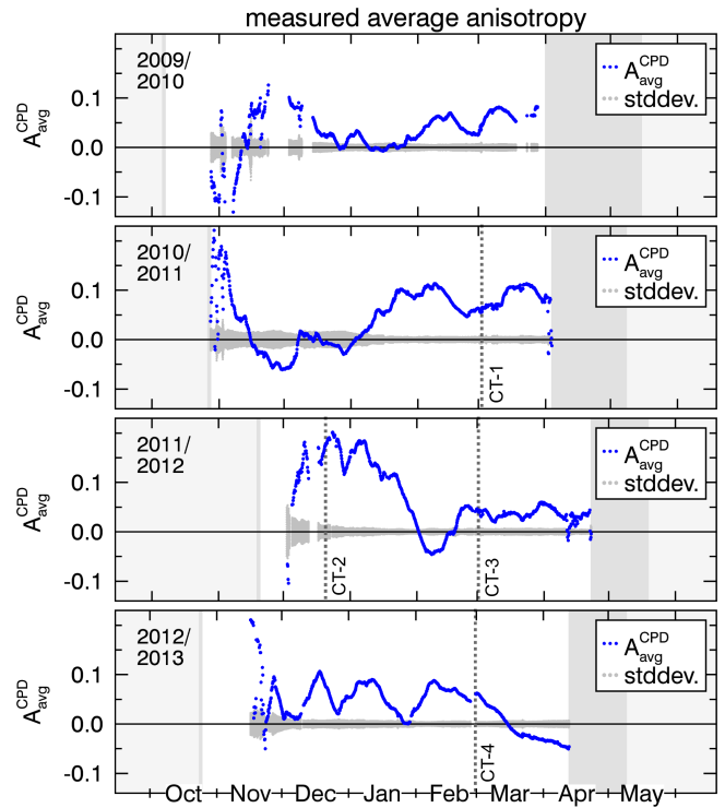
Figure 11. Average anisotropy of the snow pack, A_{\text{avg}}^{\text{CPD}} , determined during dry snow conditions for the winter seasons from 2009–2013. The anisotropy was derived from the CPD measured by the SnowScat instrument. The standard deviation of A_{\text{avg}}^{\text{CPD}} , calculated from measurements at different frequencies and incidence angles, is shown as the time-varying gray bar below the anisotropy. The dark-gray shading in April/May indicates the period of snow melt, the light-gray shadings (Oct./Nov., May/June) indicate snow free conditions. The four dashed vertical lines show the times when the anisotropy was measured by computer tomography (CT-1, -2, -3, and -4).
