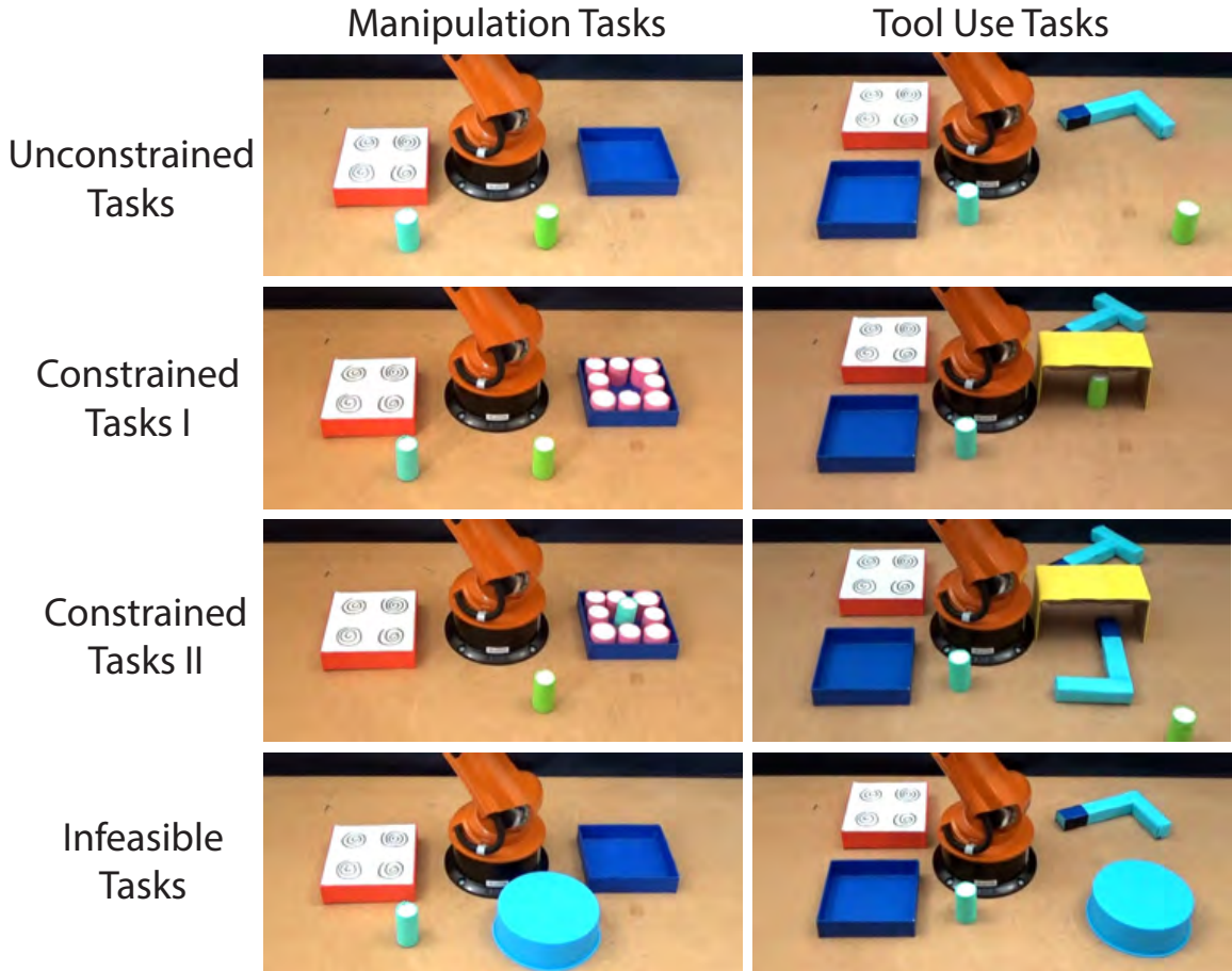
Figure 4.4: Eight tasks in our evaluations with a Kuka youBot arm.
