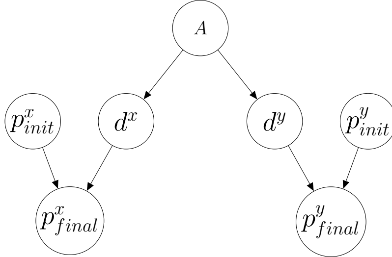
Figure 5.4: The learned structure of the SCM.
