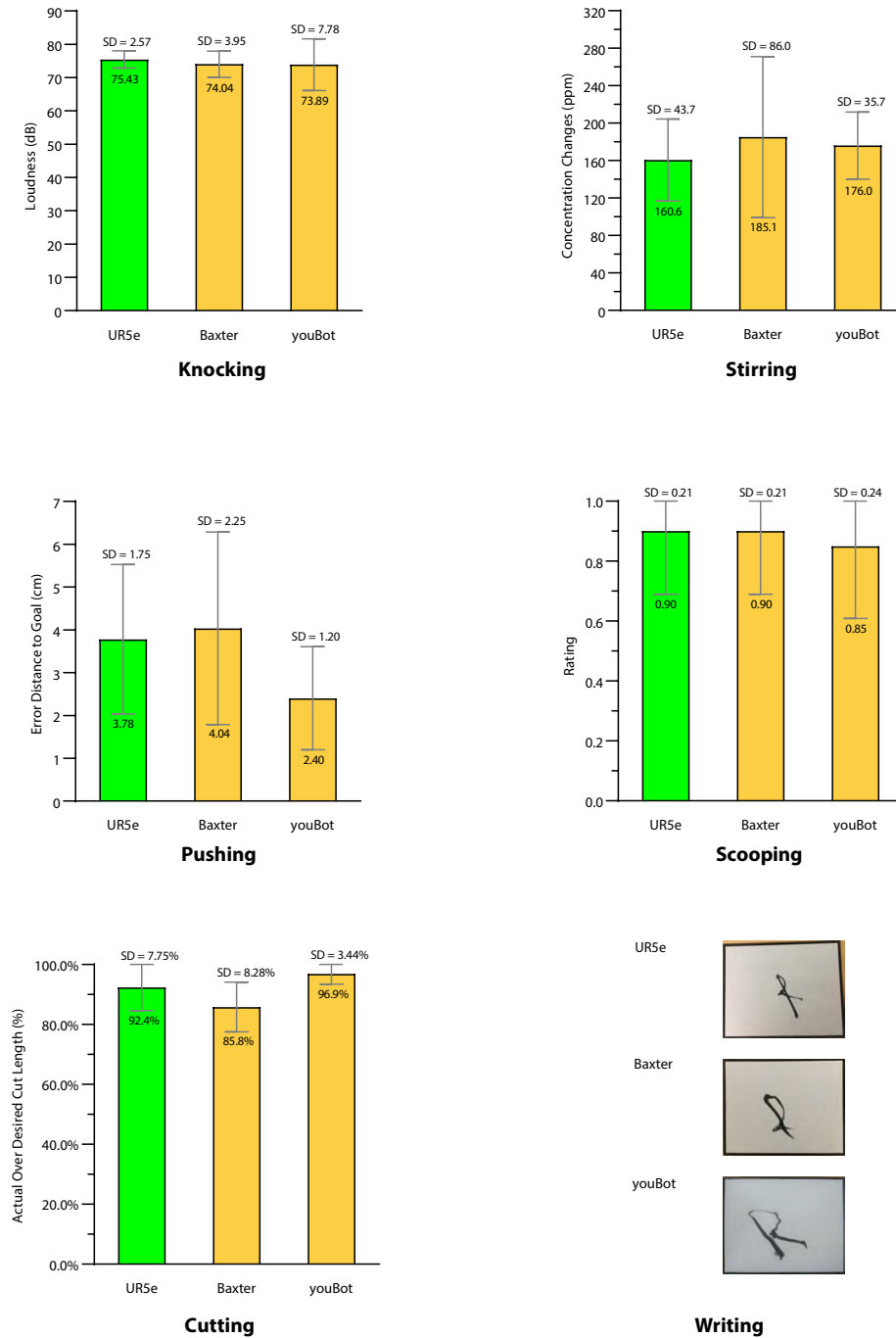
Figure 3.11: Results of tool use generalization across robot platforms (Star 3). The bar graphs include results of the UR5e (green), Baxter (yellow), and youBot (yellow) using the source tool/manipulandum combinations for knocking, stirring, pushing, scooping, and cutting. The pictures at the bottom right demonstrate different robots writing “R” with trained scale and orientation.
