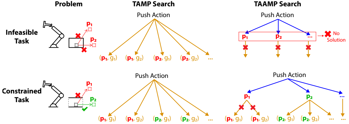
Figure 4.2: Diagram of the search for action parameters in TAMP and in TAAMP for the action push . (Top) In an infeasible task in which a block cannot be pushed from under an immovable container, TAMP attempts to search for a feasible combination including affordance-centric parameters (e.g., goal poses of the block p ) and robot-related parameters (e.g., grasping pose g ). Affordance planning detects that none of the p 's are feasible in a generic sense and does not attempt to search for robot-related parameters such as grasping poses. (Bottom) In a constrained task where the block is located inside a tunnel, TAMP needs to consider a large space, including p 's that are either feasible or infeasible, and searches for feasible combinations to instantiate the action push . Affordance planning detects the p 's that are feasible and performs motion planning only within feasible p states.
