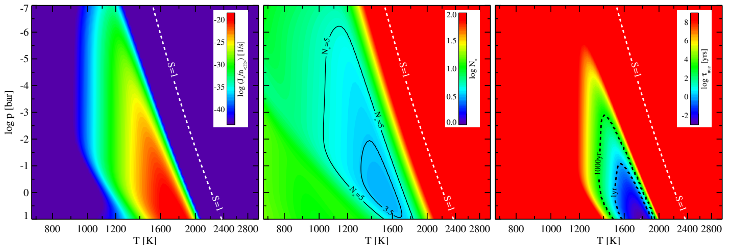
Fig. 13. Left: The nucleation rate of tungsten per hydrogen nucleus J_{\star}/n_{(H)} [1/s] as function of gas pressure and temperature. Centre: The size of the critical cluster N_{\star} , Right: The nucleation timescale \tau_{\text{nuc}} [yrs] according to Eq. (25). The white dashed contour line marks saturation S = 1 , the gas is supersaturated to the left of this line.
