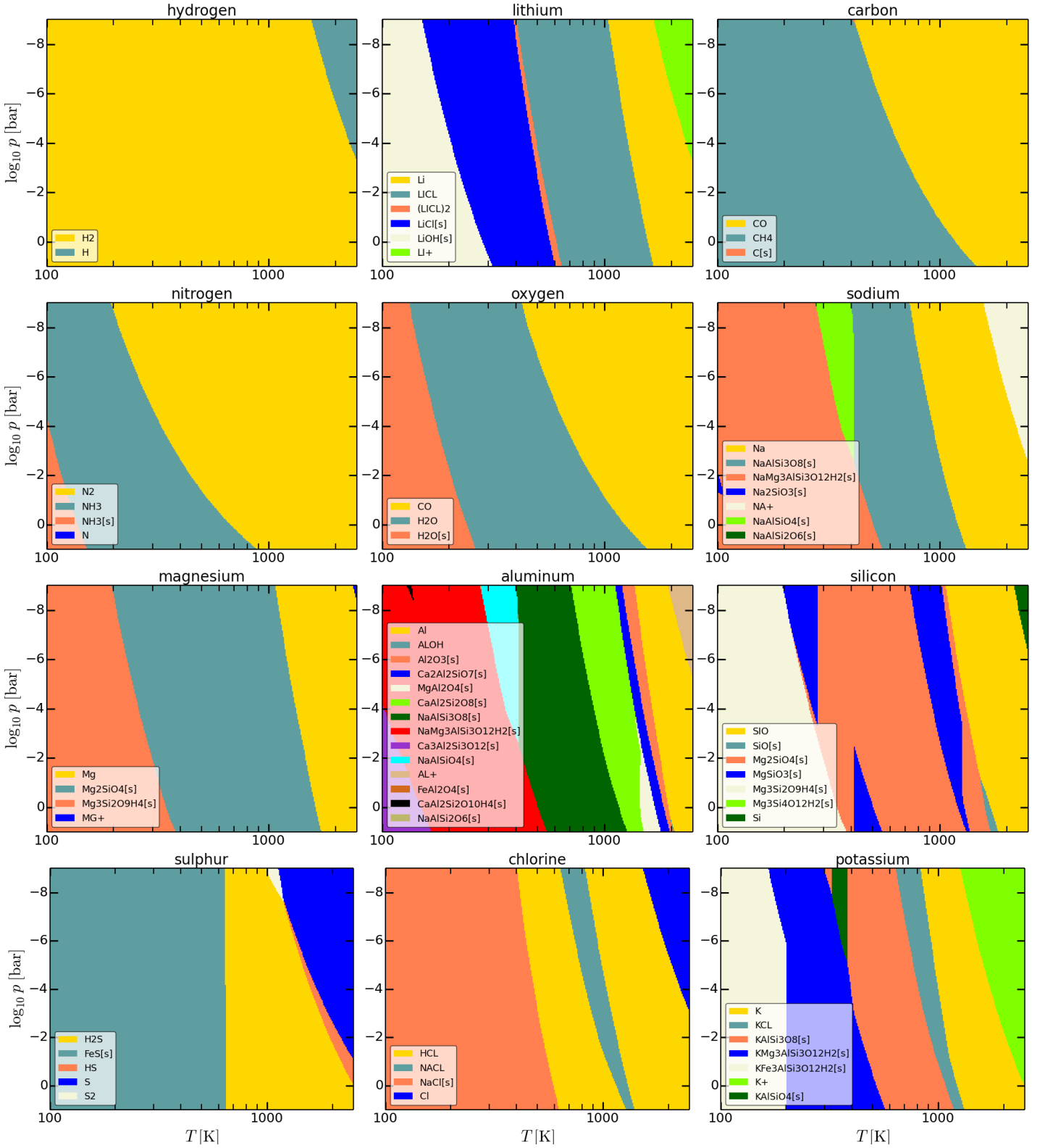
Fig. 10. Gas phase/condensed species which contain most of the elements in the (p, T) -plane. Solid species are marked by '[s]' and liquid species by '[l]'. At low temperatures, the elements Mg, Si, Na, Al and K are mostly present in form of phyllosilicates.
