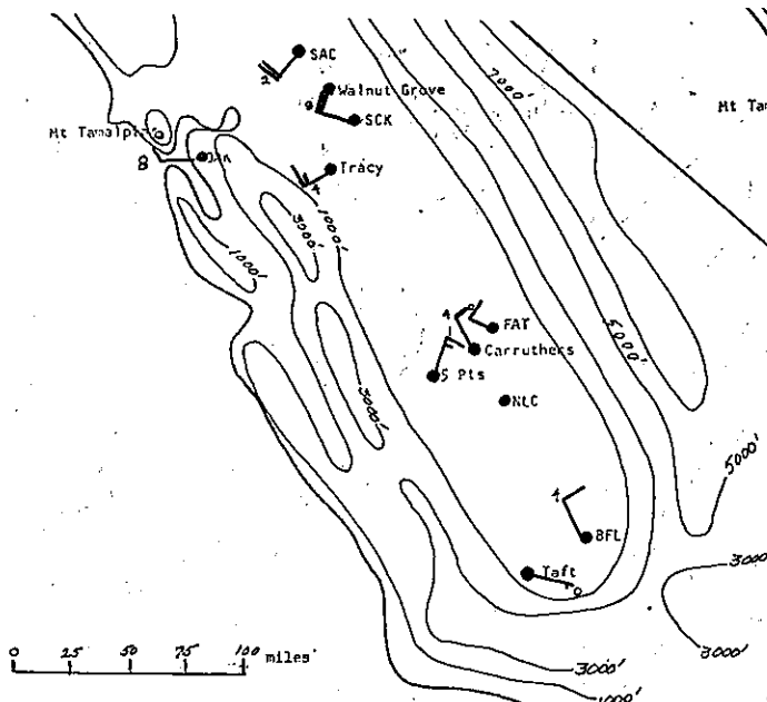
FIGURE 12A. WINDS AT 293 M. ABOVE GROUND FOR 1715 PST AUGUST 2, 1971. FULL BARS REPRESENTS 5 MPS. NUMBERS INDICATE DIRECTION TO TENS OF DEGREES.
