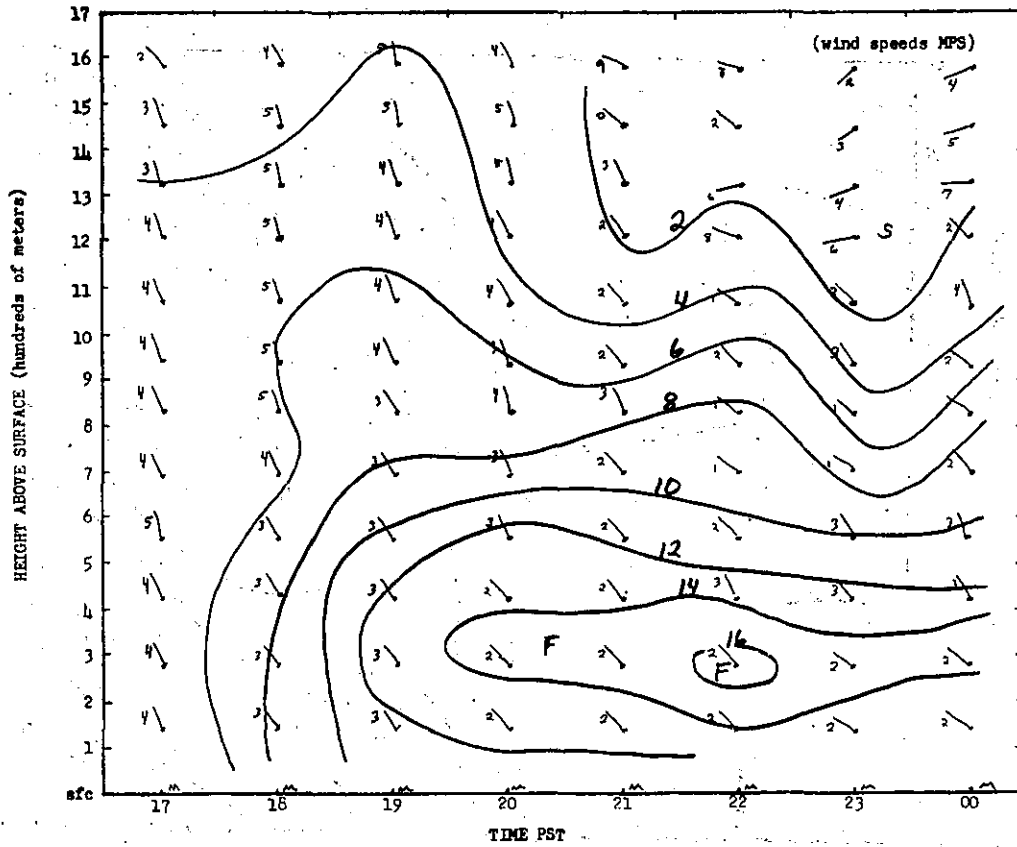
FIGURE 10E. TIME SECTION FOR CARRUTHERS, AUGUST 2, 1971.
