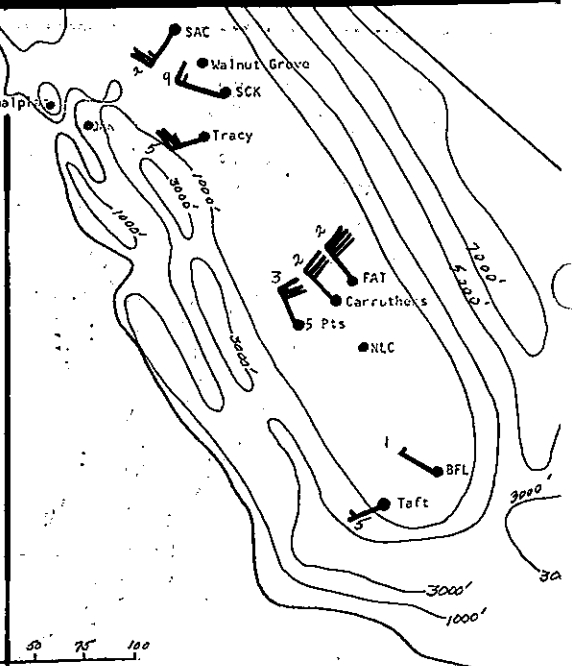
FIGURE 12D. WINDS AT 293 M. ABOVE GROUND FOR 2015 PST AUGUST 2,
