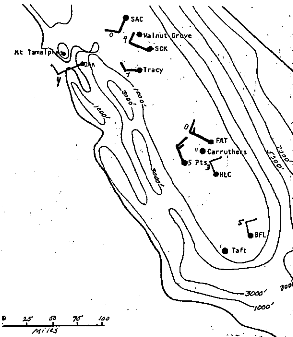
FIGURE 17A. SURFACE WINDS AT 2115 PST AUGUST 2, 1971. FULL BARB REPRESENTS 5 MPS. NUMBERS INDICATE DIRECTION TO TENS OF DEGREES.
