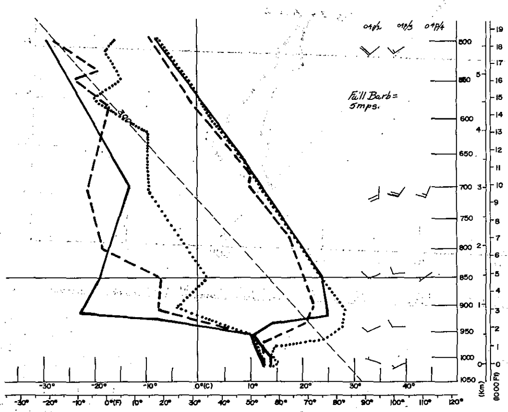
FIGURE 7A. OAKLAND, CALIFORNIA, SOUNDINGS FOR 0400 AUGUST 2 (DOTTED LINES), AUGUST 3 (SOLID LINES), AUGUST 4 (DASHED LINES), 1971.
