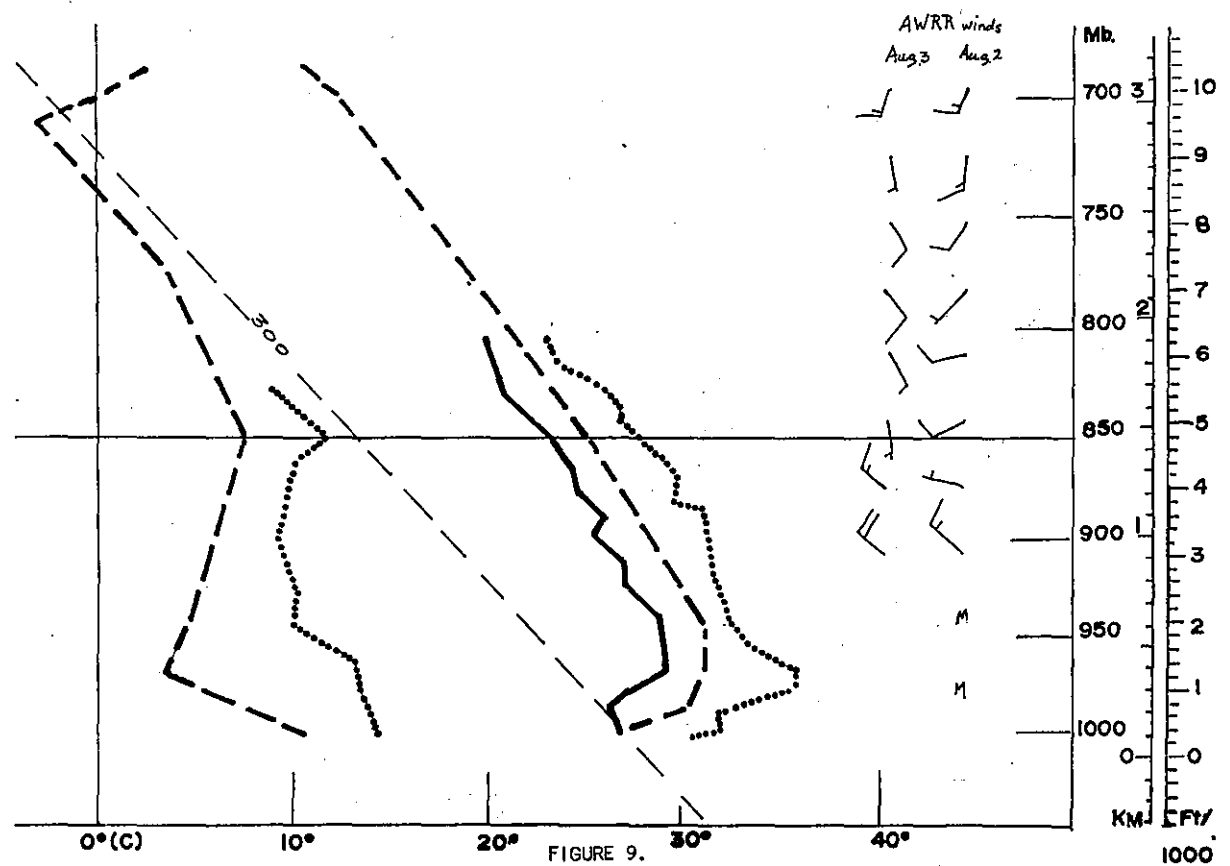
FIGURE 9. RAOB SOUNDINGS FROM AWRR FRESNO, 2155 AUGUST 2 (DOTTED LINES); 2115 AUGUST 3 (SOLID LINE) AND SOUNDING AT LEMOORE NAS, 2250 AUGUST 2 (DASHED LINES), 1971.
