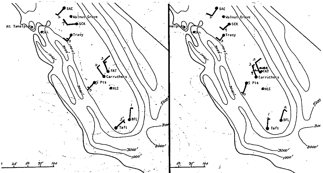
FIGURE 17I. WINDS 1085 M. ABOVE GROUND LEVEL AT 2115 PST AUGUST 2, 1971. FIGURE 17J. WINDS 1213 M. ABOVE GROUND LEVEL AT 2115 PST AUGUST 2, 1971.
