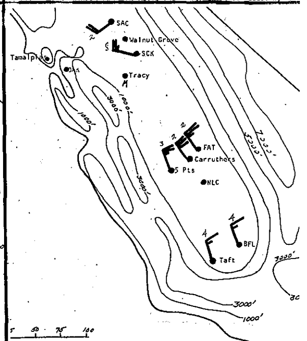
FIGURE 12H. WINDS AT 293 M. ABOVE GROUND FOR 0015 PST AUGUST 3, 1971.
