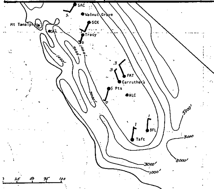
FIGURE 17K. WINDS 1341 M. ABOVE GROUND LEVEL AT 2115 PST AUGUST 2, 1971.
