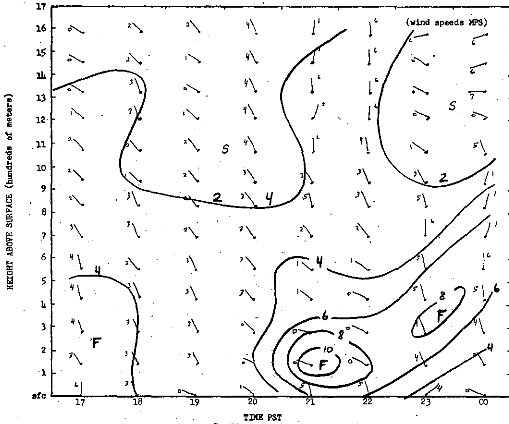
FIGURE 106. TIME SECTION FOR BAKERSFIELD, AUGUST 2, 1971.
