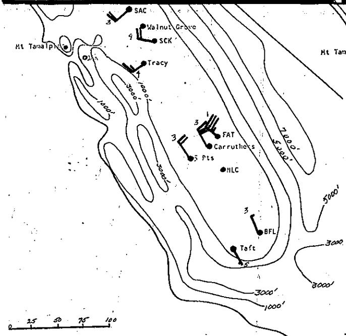
FIGURE 12C. WINDS AT 293 M. ABOVE GROUND FOR 1915 PST AUGUST 2, 1971
