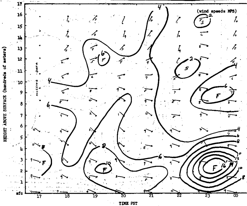
FIGURE 10B. TIME SECTION FOR STOCKTON, AUGUST 2, 1971.
