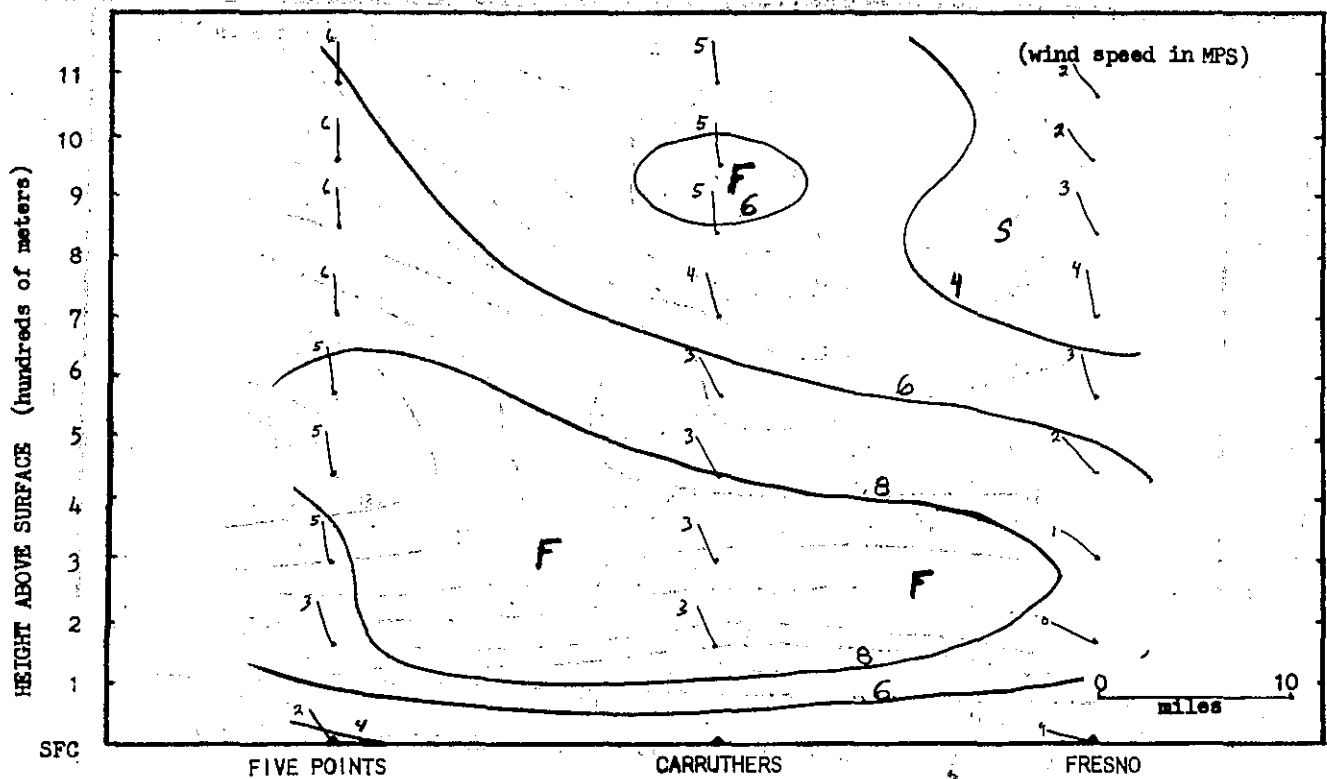
FIGURE 16B. CROSS SECTION FROM FIVE POINTS TO FRESNO FOR 1815 PST AUGUST 2, 1971.
