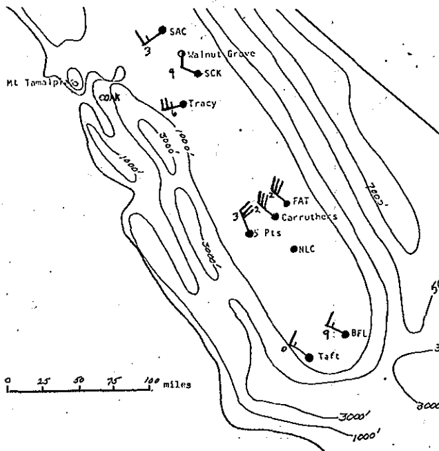
FIGURE 12E. WINDS AT 293 M. ABOVE GROUND FOR 2115 PST AUGUST 2, 1971.
