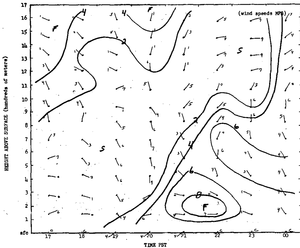
FIGURE 104. TIME SECTION FOR TAFT, AUGUST 2, 1971.
