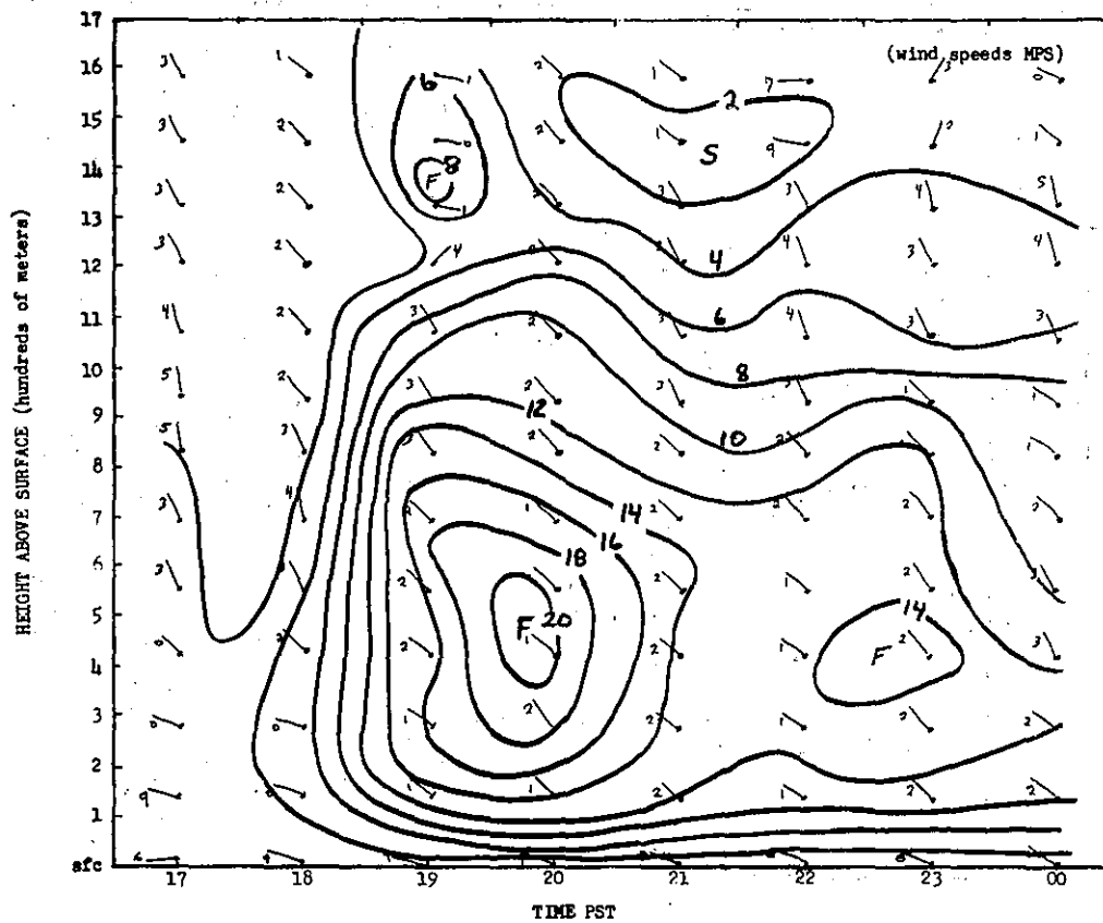
FIGURE 10D. TIME SECTION FOR FRESNO, AUGUST 2, 1971.
