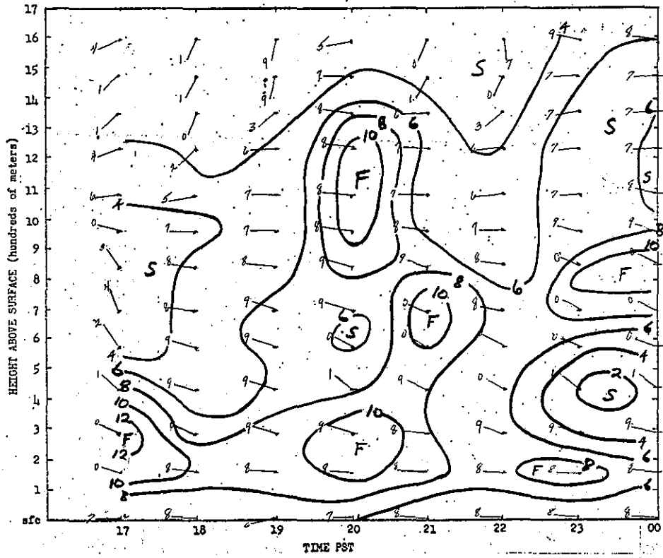
FIGURE 18C. TIME SECTION FOR STOCKTON, AUGUST 3, 1971.
