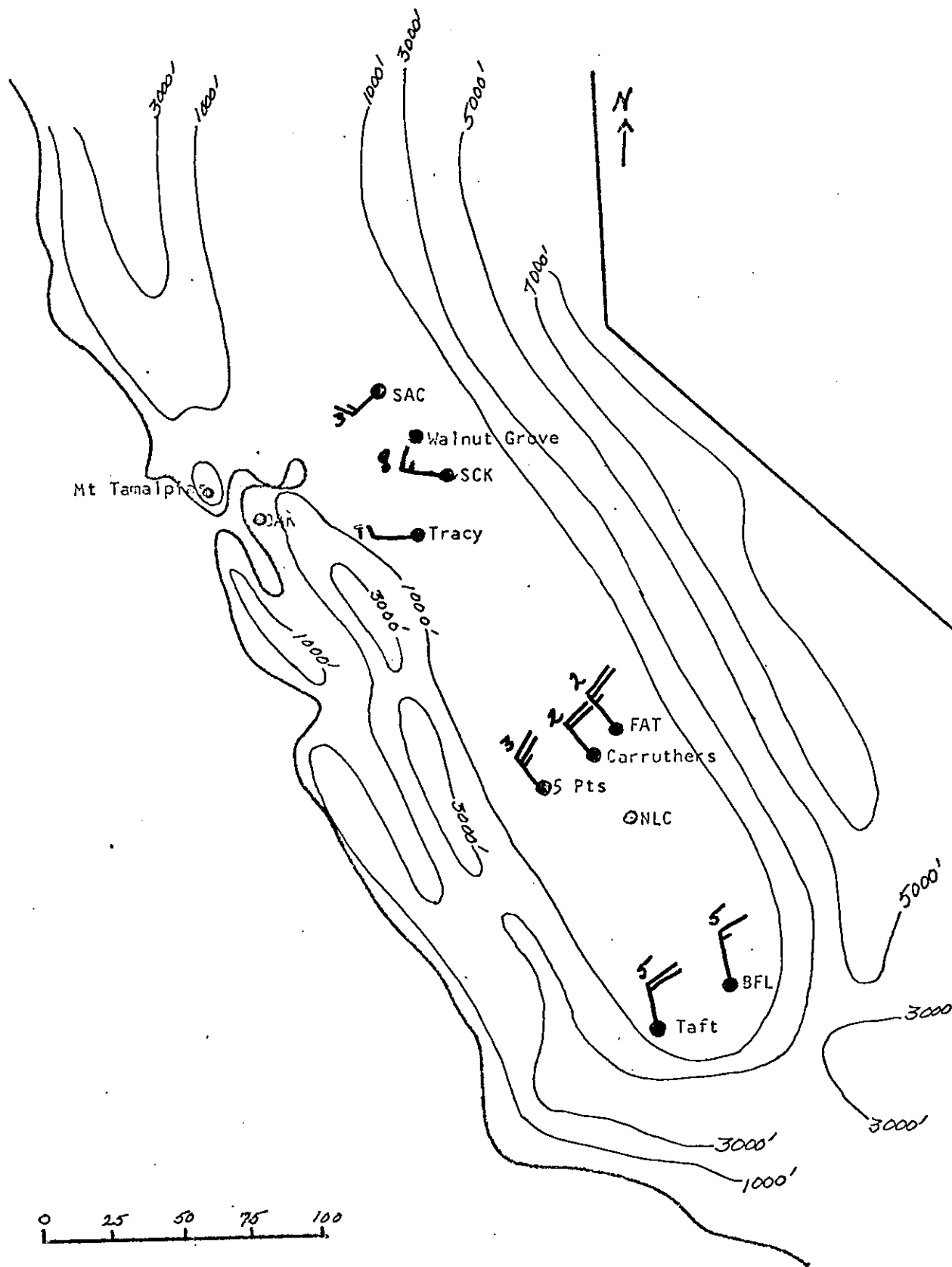
FIGURE 21. WIND FLOW OVER SAN JOAQUIN VALLEY AT 293 M., 2115 PST AUGUST 3, 1971. FULL BARB REPRESENTS 5 MPS. NUMBERS INDICATE DIRECTION TO TENS OF DEGREES.
