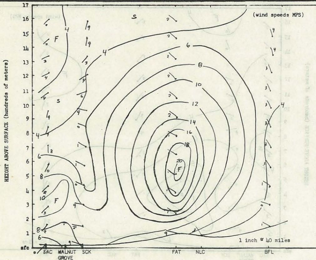
FIGURE 11D. LONGITUDINAL SECTION, SACRAMENTO-BAKERSFIELD, FOR 2015 PST AUGUST 2, 1971.
