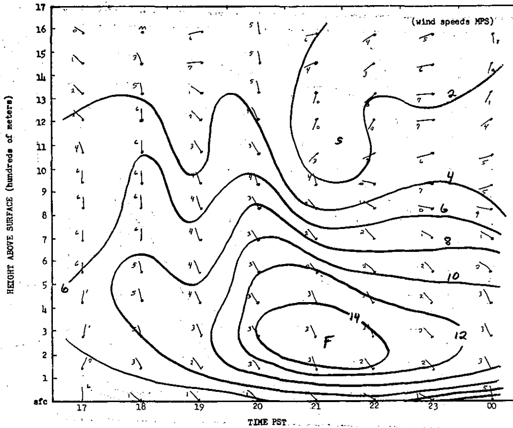
FIGURE 10F. TIME SECTION FOR FIVE POINTS, AUGUST 2, 1971.
