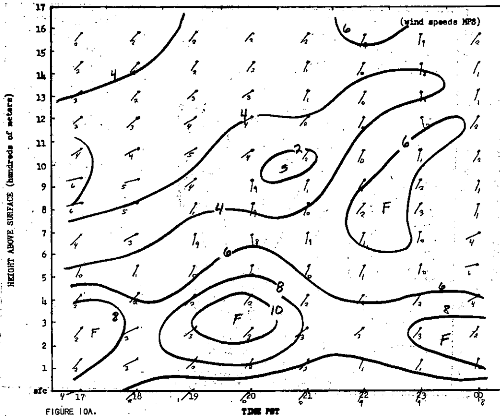
FIGURE 10A. TIME SECTION FOR SACRAMENTO, AUGUST 2, 1971. LINES ARE ISOPLETHS OF WIND SPEED (MPS). WINDS BLOW TOWARD DOT, DIRECTION IN TENS OF DEGREES. (EXAMPLE: 9 REPRESENTS 090, 190 OR 290 DEGREES; F IS FAST; S IS SLOW.)
