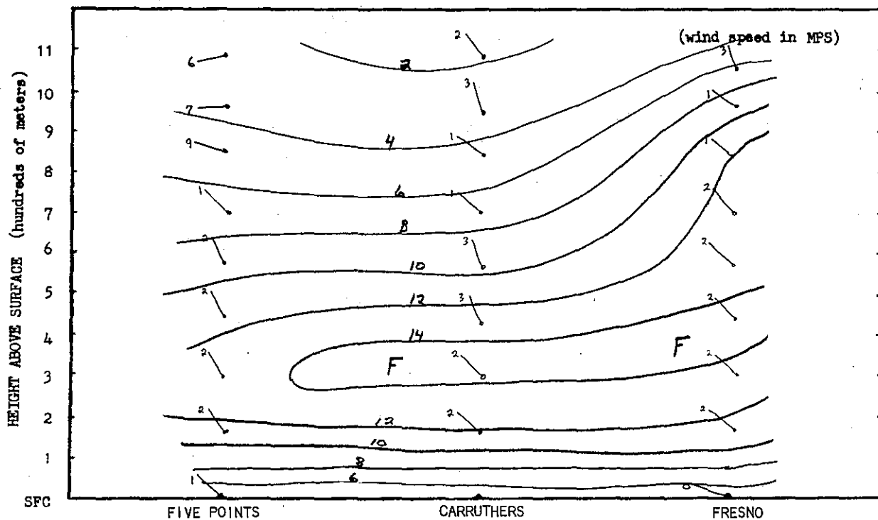
FIGURE 16G. CROSS SECTION FROM FIVE POINTS TO FRESNO FOR 2315 PST AUGUST 2, 1971.
