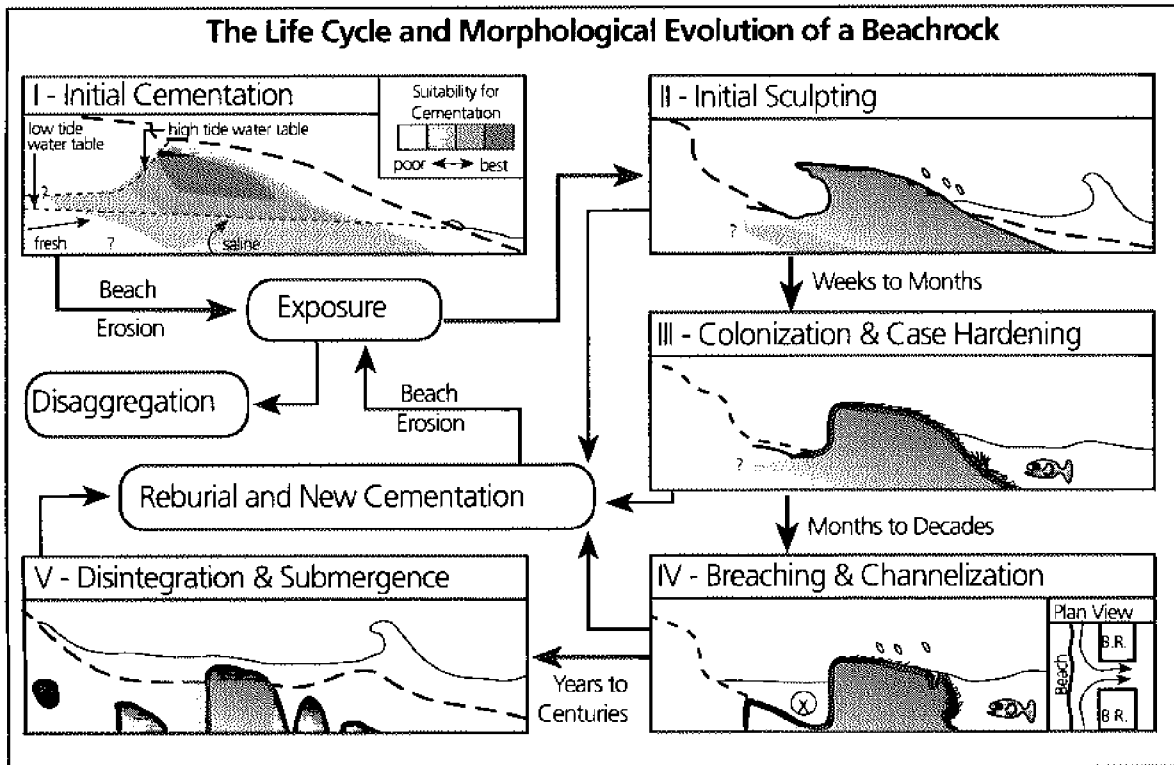
Fig. 1. Conceptual model of the stages of beachrock development. Although this model only illustrates the evolution of a single beachrock unit, it does allow for multiple episodes of beachrock formation.
