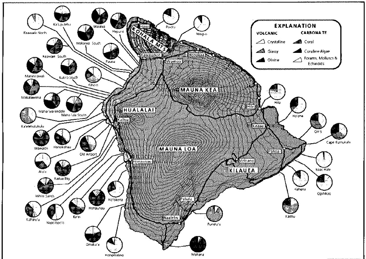
Fig. 1. Pie diagrams displaying the composition of beaches around the Big Island of Hawaii. Note the predominance of volcanic constituents along the eastern, windward portions of the island. Along the western, leeward coast carbonate constituents become abundant. Coral is the main carbonate constituent; however, coralline algae increases in abundance to the north where reefs apparently are more mature.
