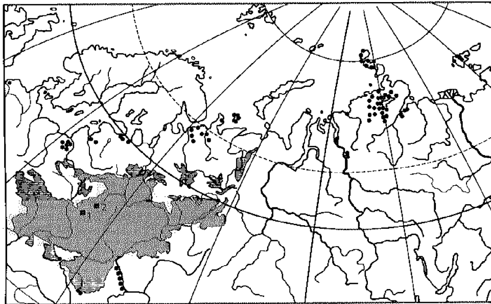
Fig. 1. Map showing the localities of collected shell samples (circles), studied loess-palaeosol sections (squares: 1 - Arapovich, 2 - Likhvin) and distribution of loesses on East-European Plain (gray area).
