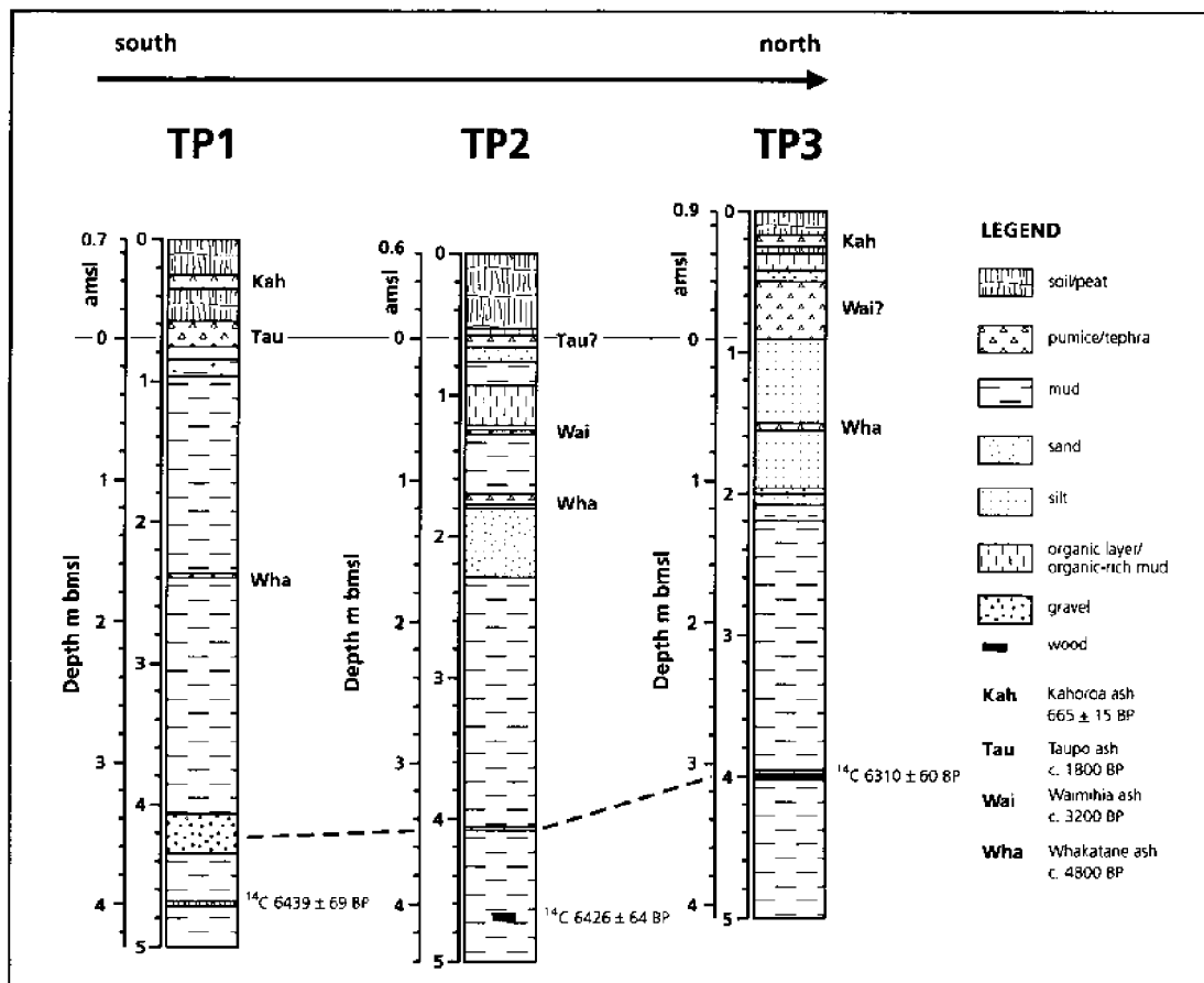
Fig. 2. Stratigraphy of cores TP1, TP2 and TP3. See Figure 1 for core locations.
