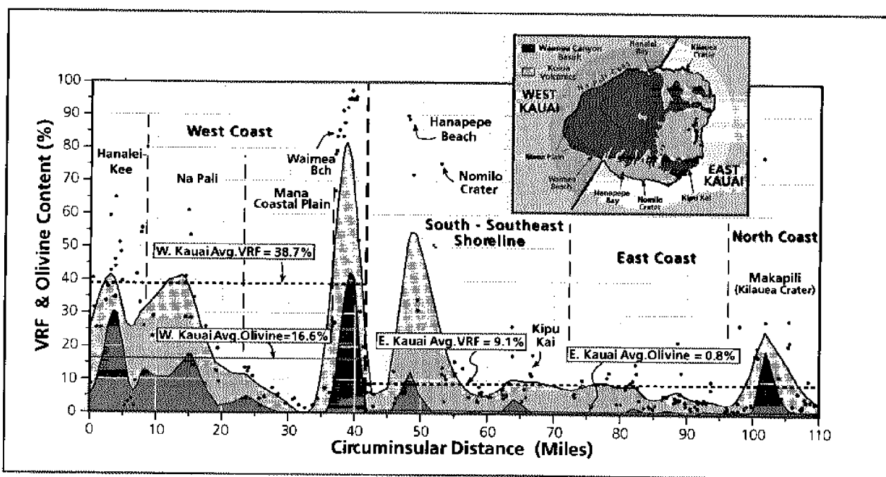
Fig. 3. Circuminsular plot of the volume of volcanic lithic materials in beaches around the Island of Kauai. The plot starts at the eastern side of Hanalei Bay and wraps around the island. Data points for total volcanic rock fragments (VRFs) (including olivine) are displayed. Data-distance smoothing curves are displayed for both total VRFs (light shading) and olivine (dark shading). The variability of VRFs and olivine within beach sediments around the island reflects the composition of the island's volcanic rocks.
