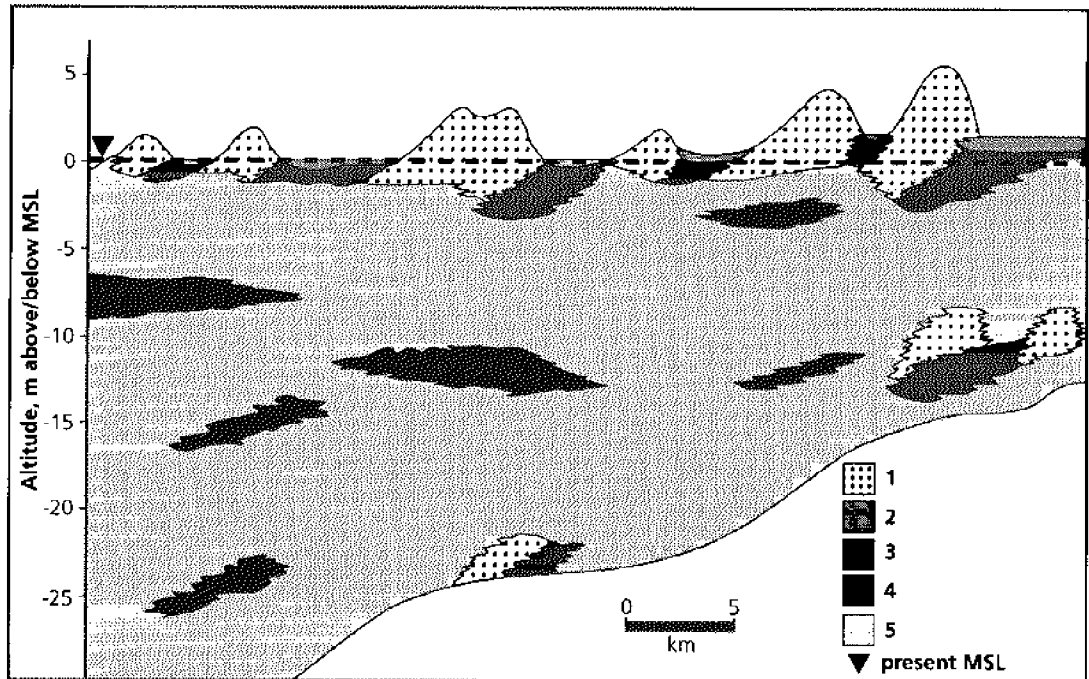
Fig. 2. Schematic geological profile of the Holocene sediments in the Kuban River delta: (1) sandy shells of coastal barriers; (2) lagoon silts and gyttia; (3) lagoon peats; (4) deltaic silts and sandy silts with peat layers; (5) deltaic shell sands and loams; (6) present mean sea-level.
