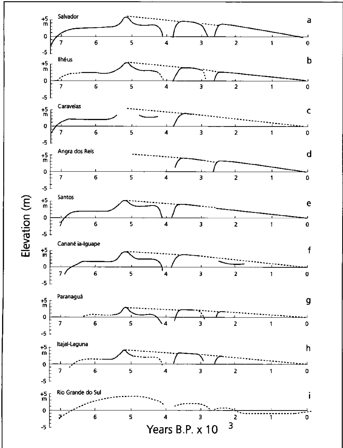
Fig. 2. The Brazilian sea level curves for the last 7000 years (after Suguio et al., 1985 and Villwock and Tomazelli, 1989, in Tomazelli, 1990). See Figure 1 for location.
