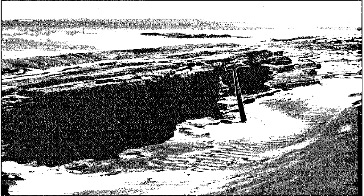
Fig. 3. Beachrock in Stage II of its development. This beachrock is weakly cemented and the outer surface has the same color as the unconsolidated sand. Longshore flow of seawater impounded on the foreshore during high tide is eroding the landward margin of the unit, increasing its relief and fostering the development of an overhang. This overhang subsequently failed, resulting in a nearly vertical landward edge. Barrio Rio Grande de Aguada, Puerto Rico.
