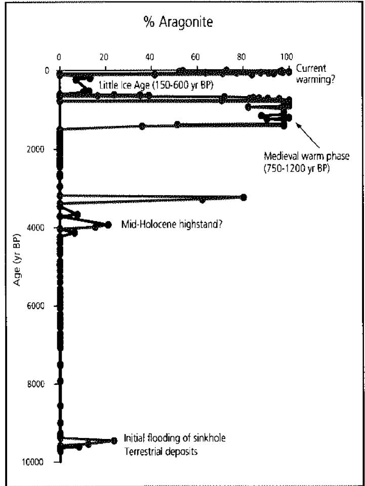
Fig. 3. Percentage of total carbonate present as aragonite versus sediment age.
