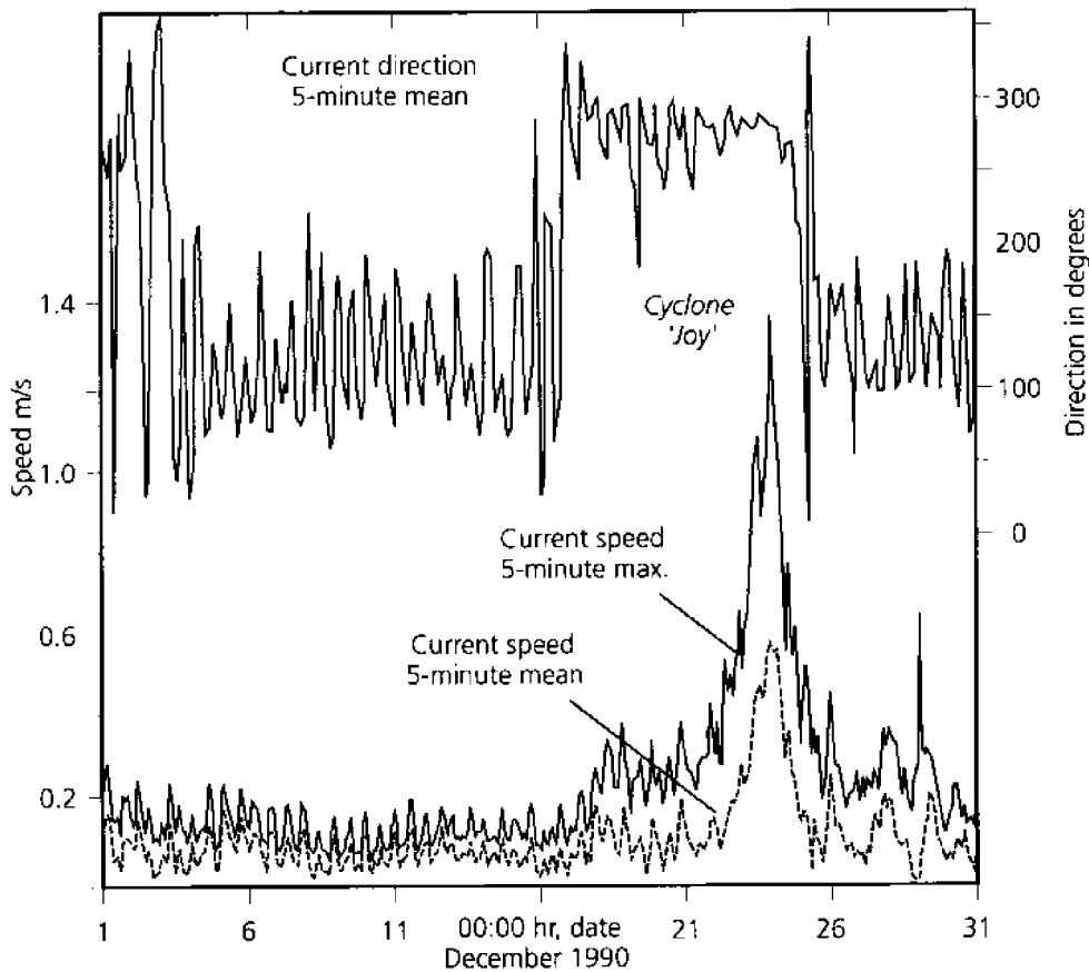
Fig. 1. Near-bed current speed and direction recorded in northern Trinity Bay, Cairns, in water depth of ~12 m, during the passage of Cyclone Joy, in late December 1990. Note that pre-cyclone current speeds rarely exceed 20 cm/s.
