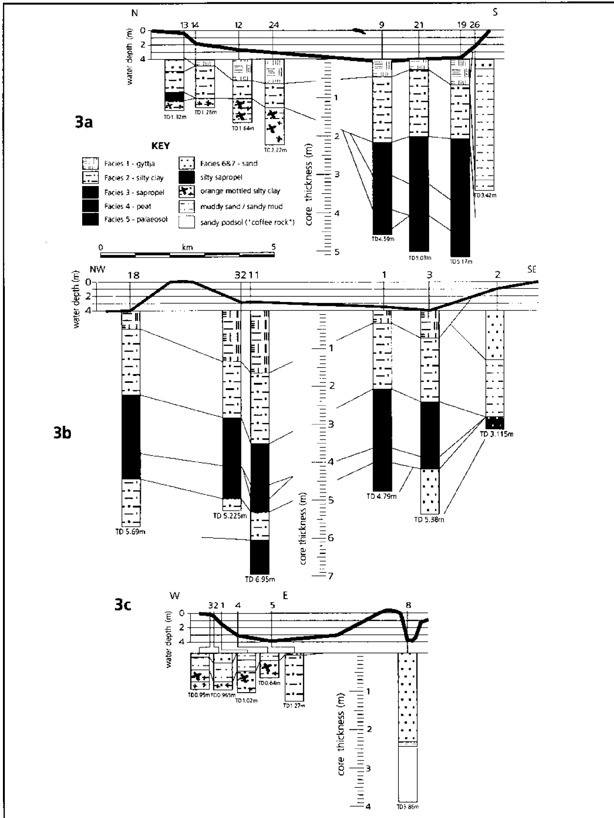
Fig. 3. Cross sections showing correlation of Quaternary facies in Myall (a,b) and Smiths (c) lakes.
