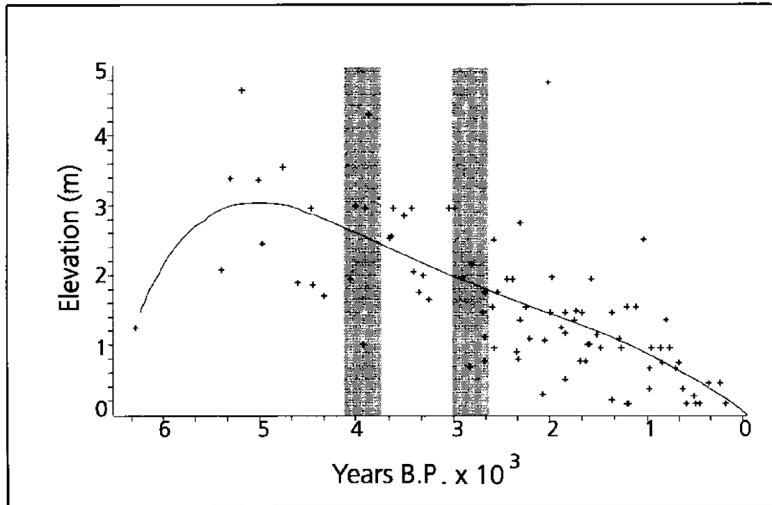
Fig. 3. Elevation of the published paleo-sea level indicators in Brazil derived from vermetid radiocarbon dates. Shaded areas indicate the time for the proposed secondary oscillations proposed by other authors (see Suguio et al. 1985). The line is a 4th order polynomial best fit. (Angulo & Lessa 1997)
