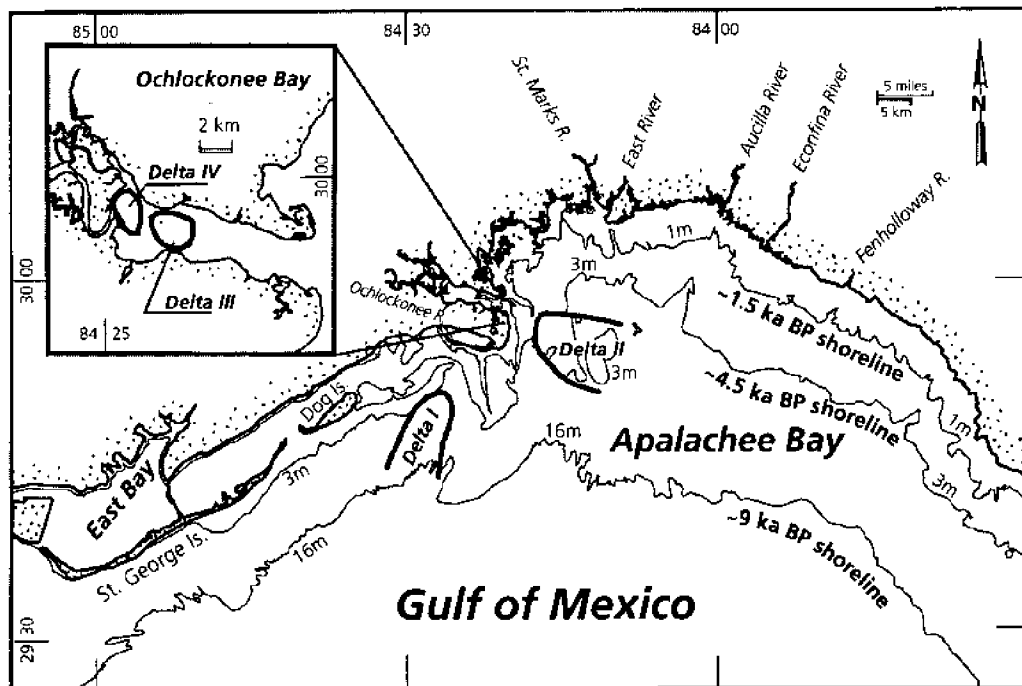
Fig. 2. A reconstruction of Holocene shoreline evolution and inferred history of the paleo-Ochlockonee River delta in response to sea-level rise in the study area. Sea-level data is based on Frazier (1974). The paleo-deltas were located and identified using seismic data from this study.
