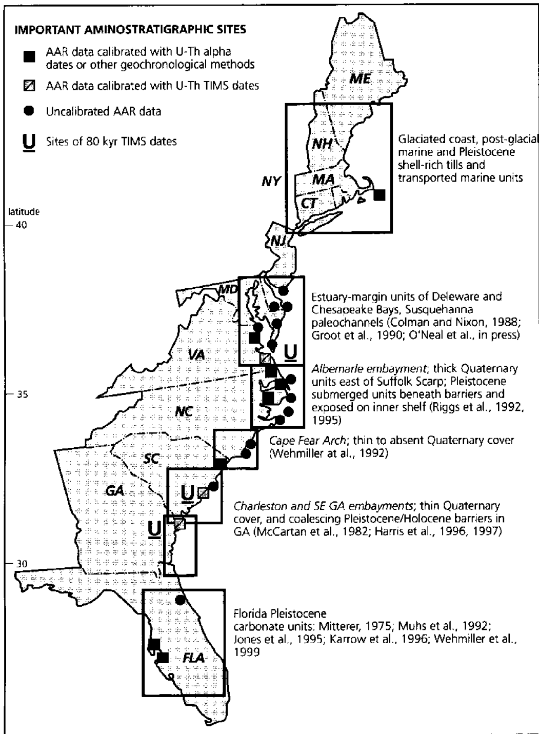
Fig. 1. Map of the US Atlantic coast, Maine to Florida, showing regions from which aminostratigraphic data have been obtained (see Wehmiller et al., 1988 for details regarding these regions). Areas south of the glacial limit (New Jersey to Florida) are the focus of this presentation. Delineated areas identify regions within which similar geomorphic processes appear to have functioned during the Quaternary. Selected references to aminostratigraphic data from each region are shown.
