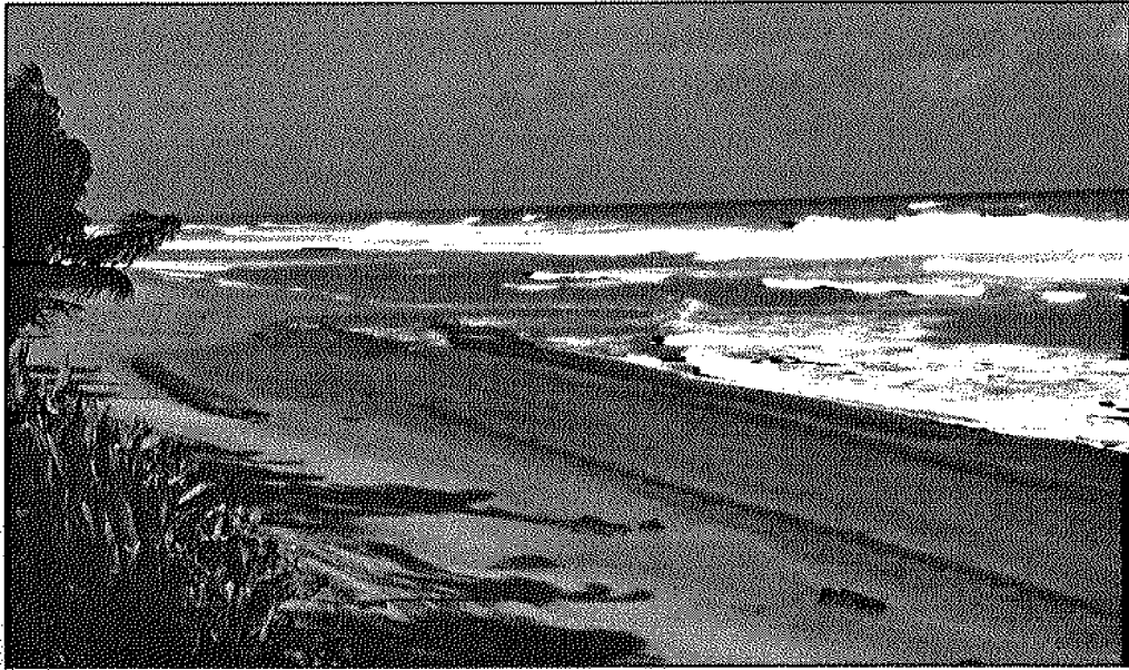
Fig. 5. Multiple unit beachrock exposure at Barrio Rio Grande de Aguada, Puerto Rico. Seawater impounded by the beachrock flows from right to left and discharges to the sea in a rip current where there is an eroded gap in the seaward beachrock unit. Maximum variability of beach volume and width occurs opposite this gap.
