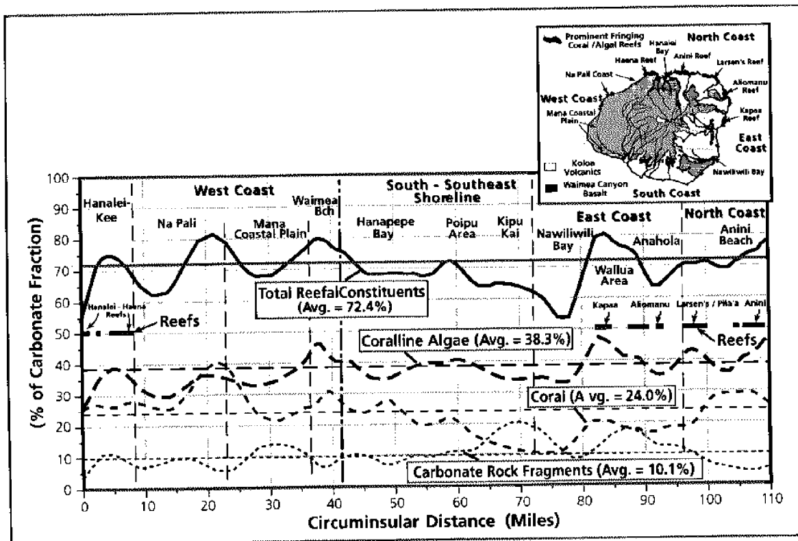
Fig. 4. Circuminsular plot of reefal carbonate constituents of Kauai's beach sediments. Note the location of the prominent fringing coral/algal reefs. The distribution of these carbonate grains does not appear to reflect the location of reef structures. Coralline algae is most abundant, indicative of the predominance of stony red algae in Kauai's reefs.
