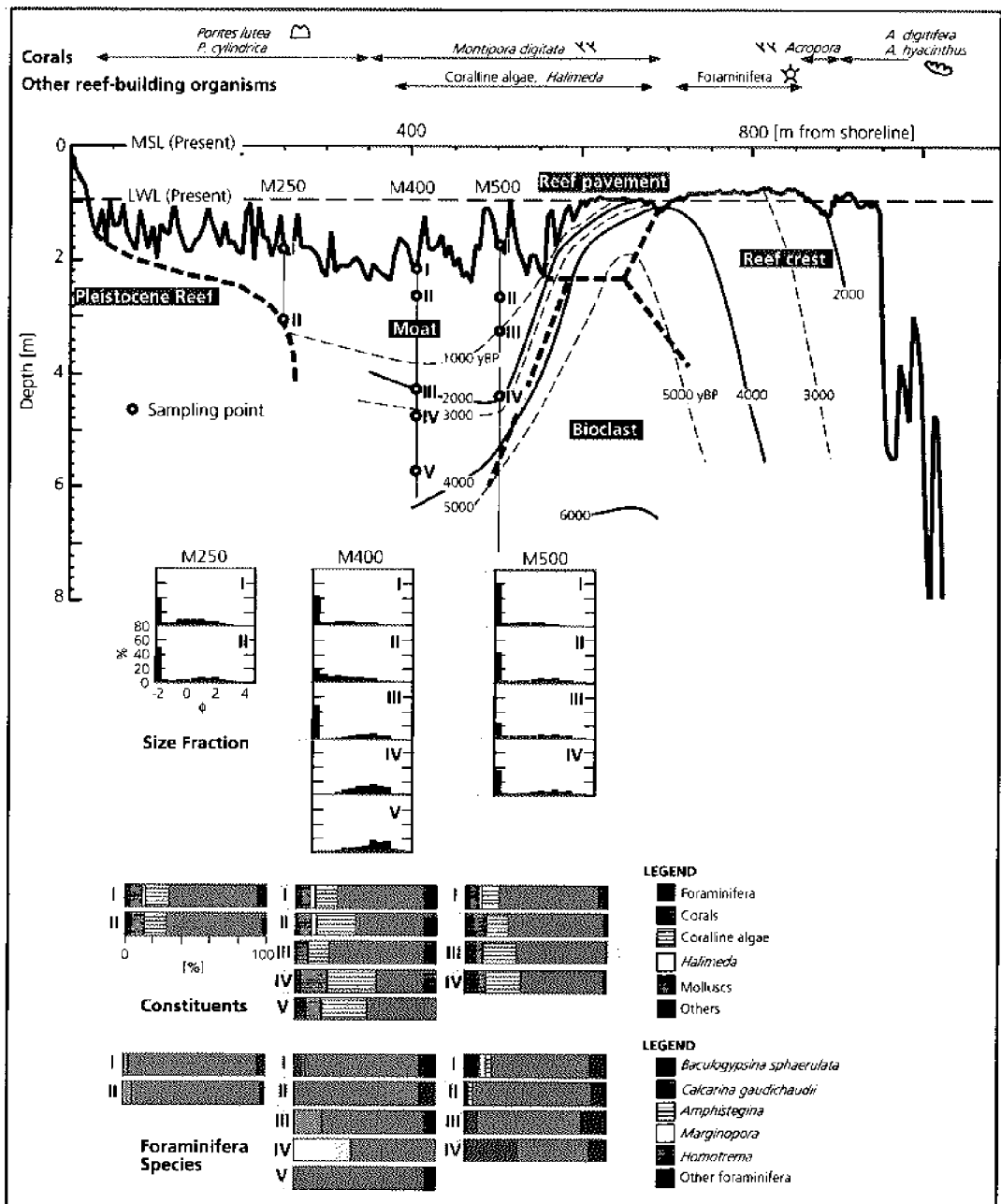
Fig. 2. The present distribution of reef-building organisms, the topographic profile, and internal facies of Kabira Reef flat. Isochronal lines based on the radiocarbon ages of coral and foraminifera specimens. Vertical lines show drill holes. The distribution of corals and the topographic profile are from Yamano et al. (1999a). Size fraction and constituents of the sediments, ratio of each foraminifera tests obtained from the moat cores (M250, M400 and M500). Adapted from Yamano et al. (submitted). The backreef structure (moat) was infilled after the establishment of the reef framework (reef crest). Corals and coral fragments coarser than 2.0 \phi is the major constituents of the backreef structure. Significant amount of shallow species of benthic foraminifera occurred after 2000 yr BP. Calcarina gaudichaudii occurred after 3500 yr BP, and Baculogypsina sphaerulata occurred after 2000 yr BP.
