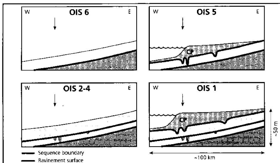
Fig. 1. Schematic dip-oriented section illustrating the evolution of the Rhine-Meuse system in the west-central Netherlands during the last glacio-eustatic cycles. Arrow indicates the position of the core. Sequence boundaries result from fluvial erosion due to sea-level fall; ravinement surfaces result from transgressive scour. Note the occurrence of both wave, tidal and fluvial ravinement surfaces. OIS = oxygen-isotope stage, CP = coastal prism.
