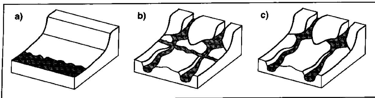
Fig 1. Schematic diagram showing general modes of sediment distribution observed in the study area. Gray areas designate unconsolidated sediment and white areas are bedrock. (a) Continuous rocky coastline where no streams have incised the topography and the dominant offshore wave direction is parallel to the coast. (b) Embayed coastline with pocket beaches and shore-normal, sediment-filled paleo-stream channels connected by shallow, shore-parallel ribbons of sediment in shallow water. The dominant offshore wave direction is shore-parallel. (c) Embayed coastline with pocket beaches and shore-normal, sediment-filled paleo-stream channels. The dominant offshore wave direction in this configuration is shore-normal.
