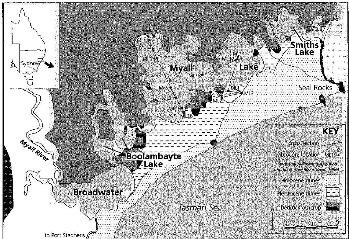
Fig.1. Myall Lakes system showing location of cores and cross sections.
