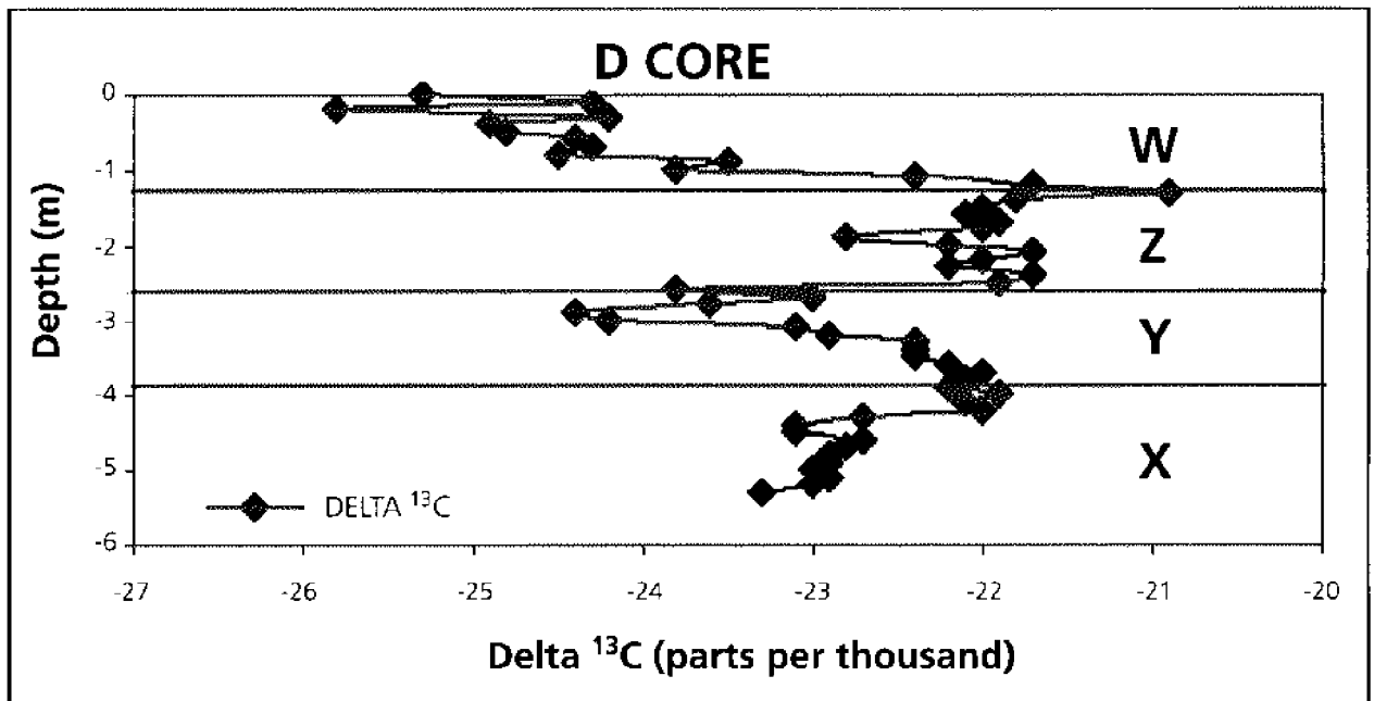
Fig. 2. Isotopic ratios of C to core D
