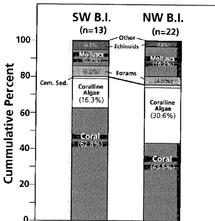
Fig. 2. Histograms of carbonate constituents of beaches along the leeward portion of the Big Island, south and north of Kailua, showing the predominance of coral clasts but also the increase in coralline algae and molluscan fragments northward.
