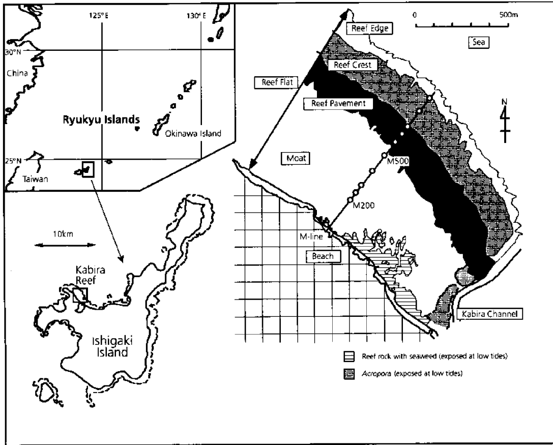
Fig. 1. Kabira Reef located at the northwestern coast of Ishigaki Island, the Ryukyu Islands, Southwest Japan (left). Geomorphological map of Kabira Reef and a transect (M-line) set perpendicular to the shore-line (right). Open circles show the drilling points.
