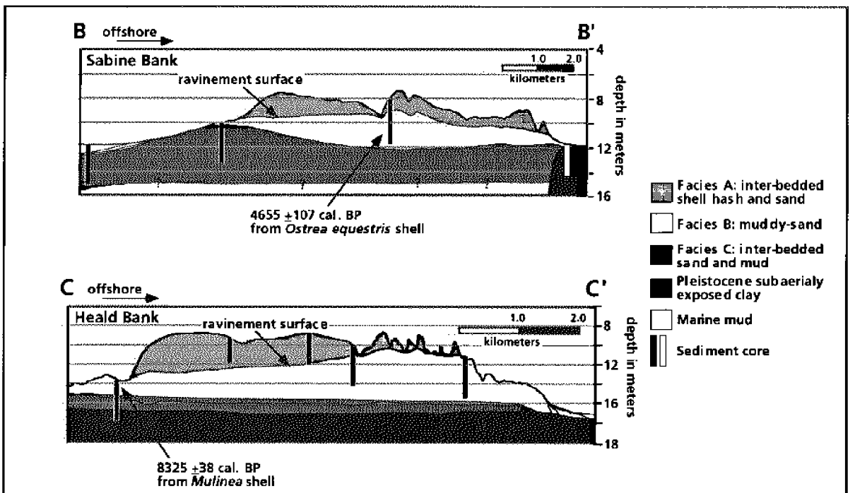
Fig. 3. Cross sections B-B' through Sabine Bank and C-C' through Heald Bank. The ~10 m (Sabine Bank) and ~14 m (Heald Bank) flooding surfaces are indicated by dashed lines.
