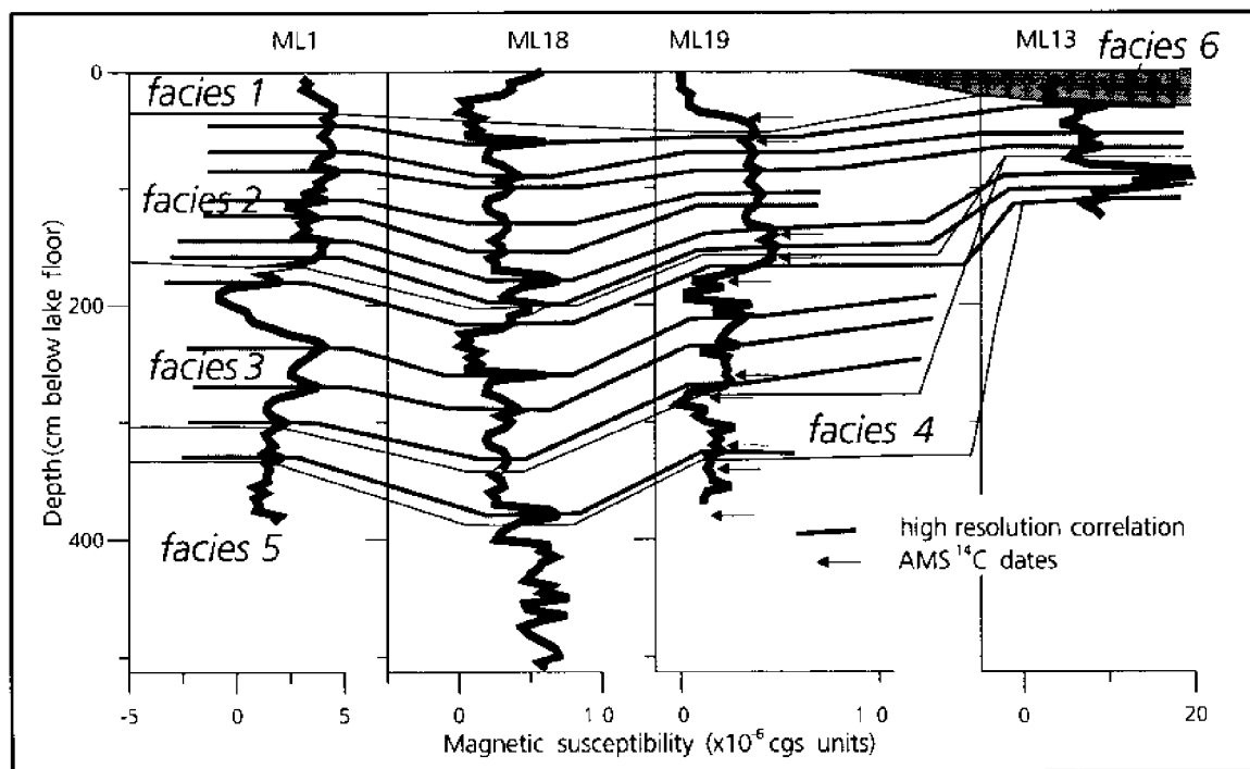
Fig. 7. Correlation of magnetic susceptibility profiles for Myall Lakes cores.
