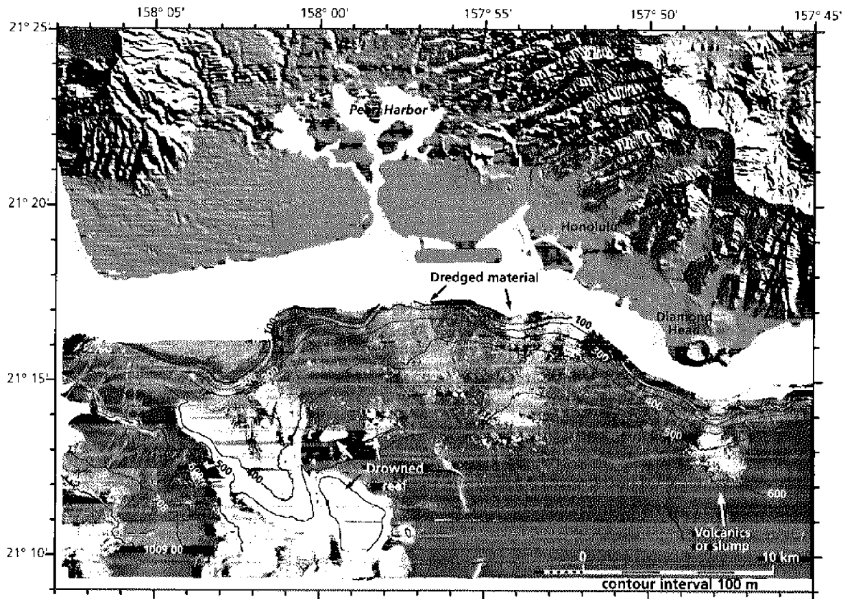
Fig. 2. Multibeam backscatter image from Mamala Bay. Note the high backscatter (bright tones) dredged-material deposits and drowned reef platforms. In contrast, natural sediment is characterized by low backscatter (dark tones).
