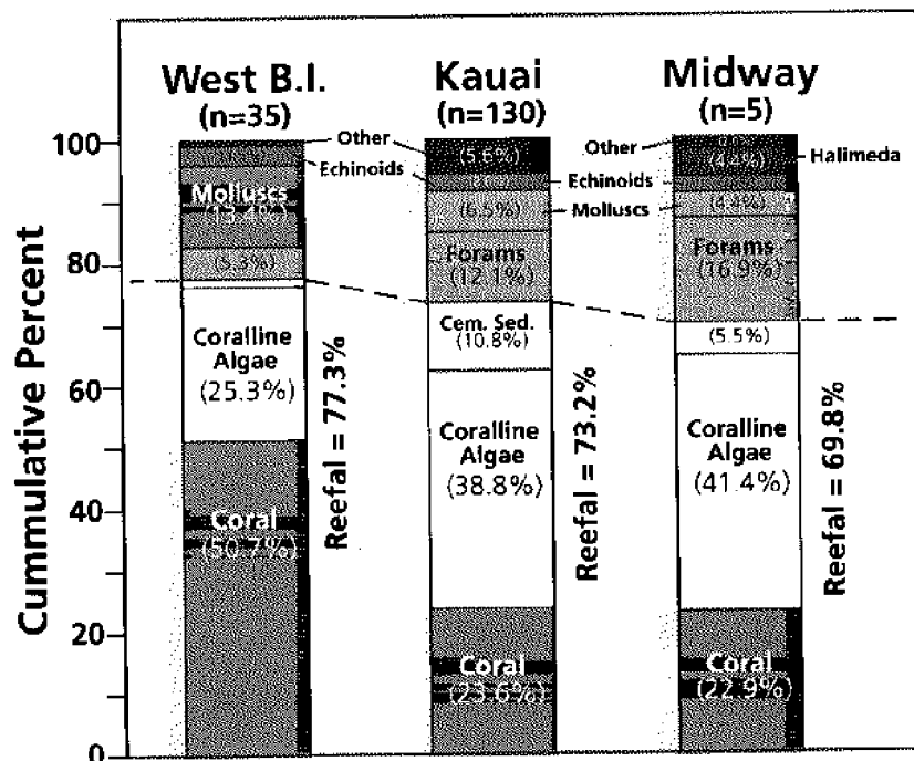
Fig. 5. Comparative histograms of carbonate constituents of beaches for the western portion of the Big Island, Island of Kauai and islands of Midway Atoll. Note the increase of coralline algae, cemented-sediment intraclasts and foraminifers in Kauai and Midway beach sediments, most probably indicative of the greater stability and maturity of their coral/algal reefs.
