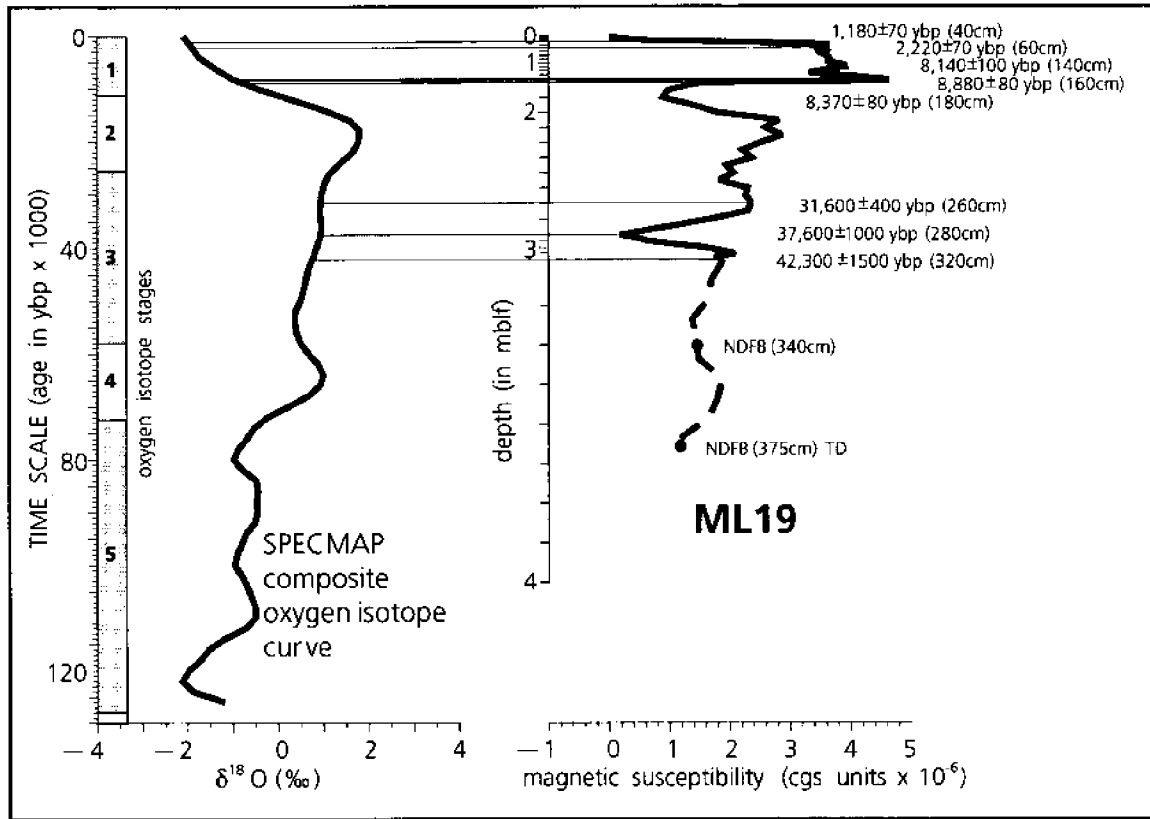
Fig. 6. Correlation between magnetic susceptibility in ML19
