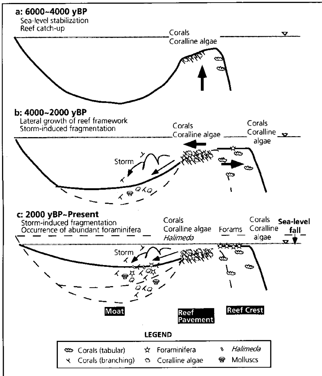
Fig. 3. The stage of sedimentation of Kabira Reef flat from 6000 yr BP to the present. The reef crest caught up with the sea-level at about 4000 yBP. Then, the reef framework expanded both oceanward and landward. The moat was infilled by coral fragments and coralline algae supplied by fragmentation due to typhoon events. Sea-level fall at about 2000 yr BP (Kawana 1989) caused the aerial exposure of the reef crest and caused the occurrence of shallow species of benthic foraminifera, thus resulting in the modification of the constituents of backreef facies (from Yamano et al. submitted).
