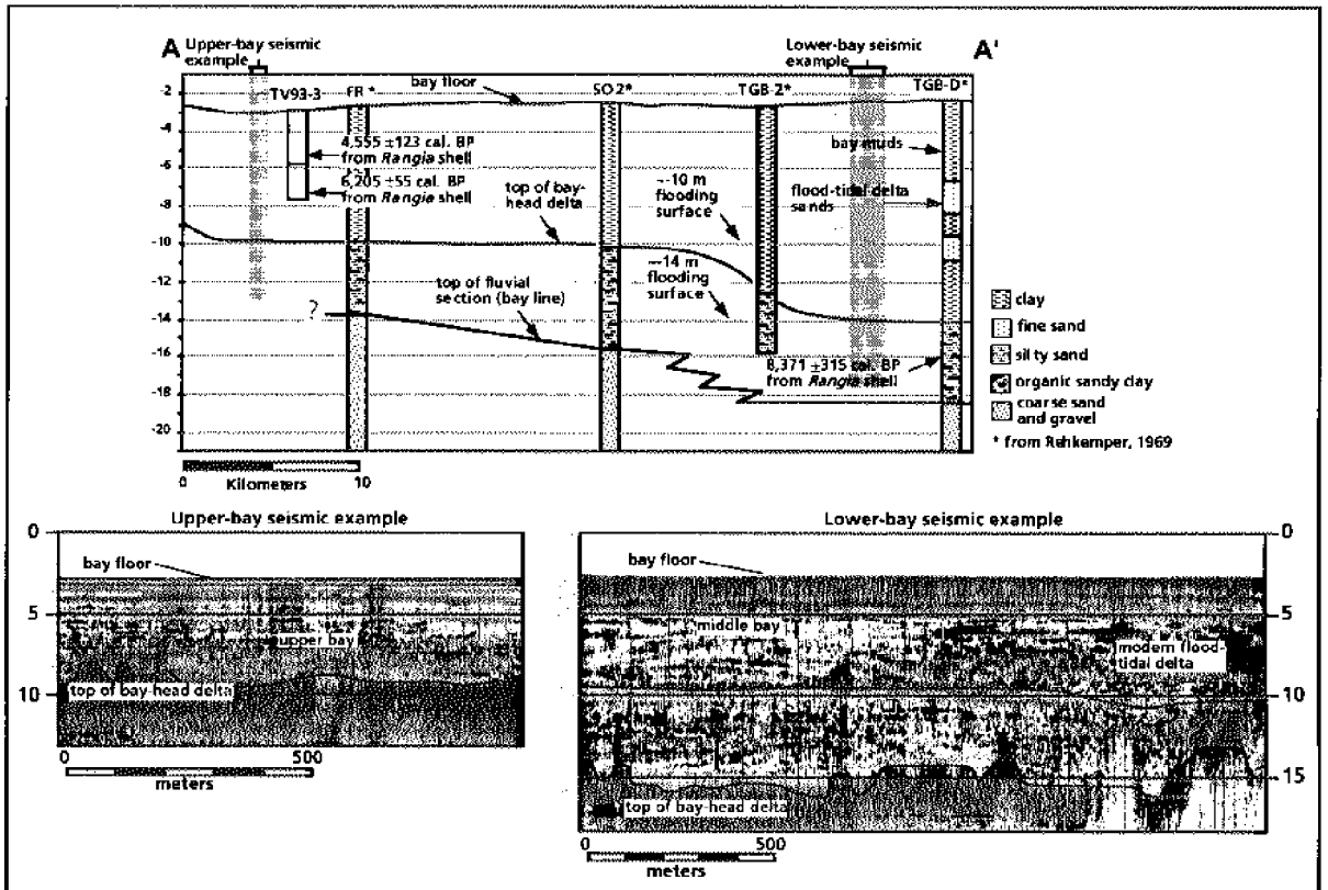
Fig. 2. Cross-section A-A' through Galveston bay based on seismic and lithologic data. Locations of two seismic examples are indicated in gray on the cross-section. Flooding surfaces are outlined on the representative seismic examples.
