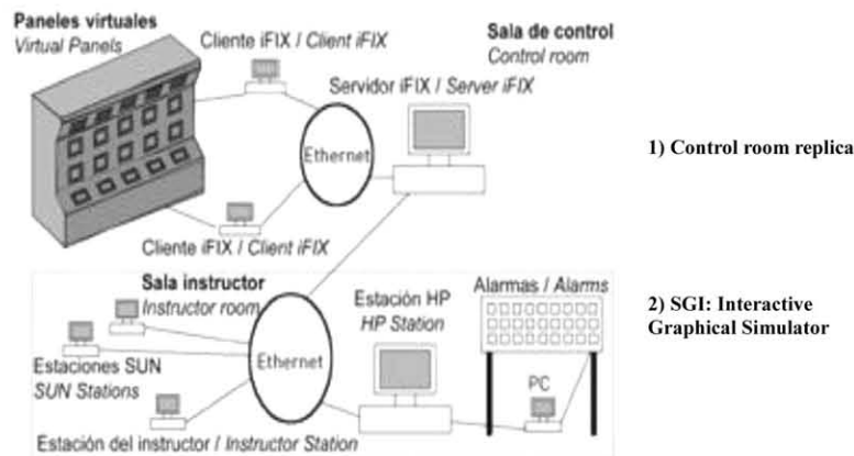
Fig. 1. José Cabrera Nuclear power plant General Simulator Arrangement.
