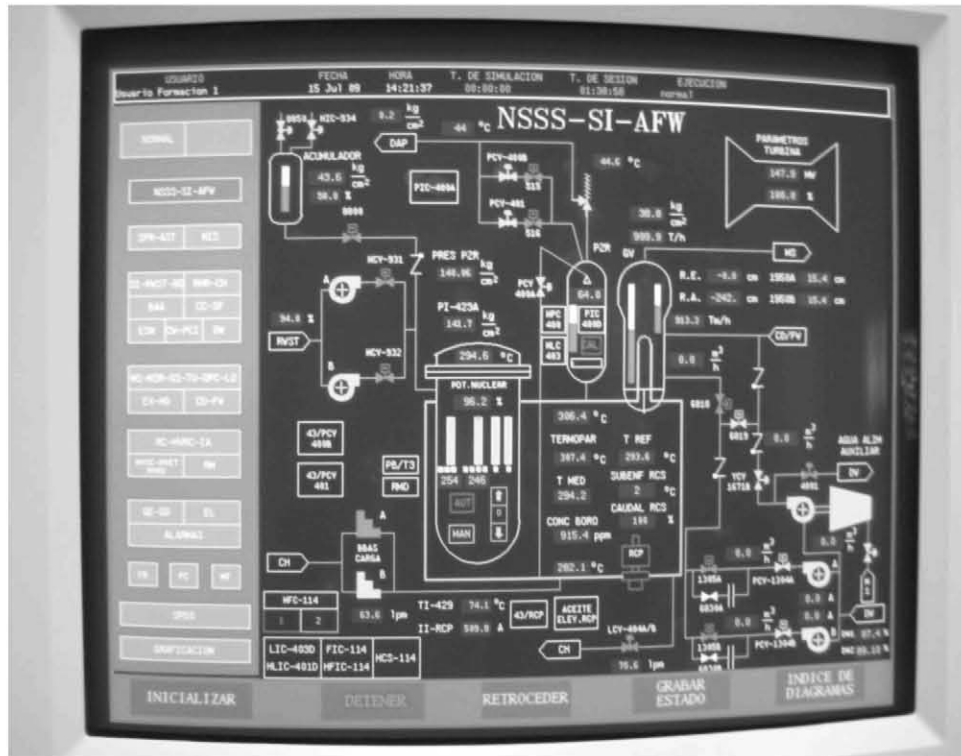
Fig. 3. One Screen with reactor vessel, injection system, and auxiliar feedwater system.
