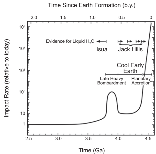
Fig. 2. The estimated meteorite-impact rate during the first 2 b.y. of Earth’s history, as proposed by Valley et al. (2002). The cool early Earth hypothesis of Valley et al. indicates that the meteoritic flux dropped precipitously over the \sim 0.15 -G.y. period of accretion, so that by 4.3 Ga, Earth was cool enough to support liquid water. Evidence for clement conditions during this era before the late heavy bombardment at \sim 3.9 Ga comes from the analysis of ^{18}\text{O} in zircon samples. Post late heavy bombardment, “Isua” denotes the oldest known water-lain chemical sediments, found in the Isua supracrustal belt in western Greenland, dating to 3.6–3.85 Ga (Nutmans et al., 1997; Whitehouse et al., 1999). Adapted from Valley et al. (2002).
