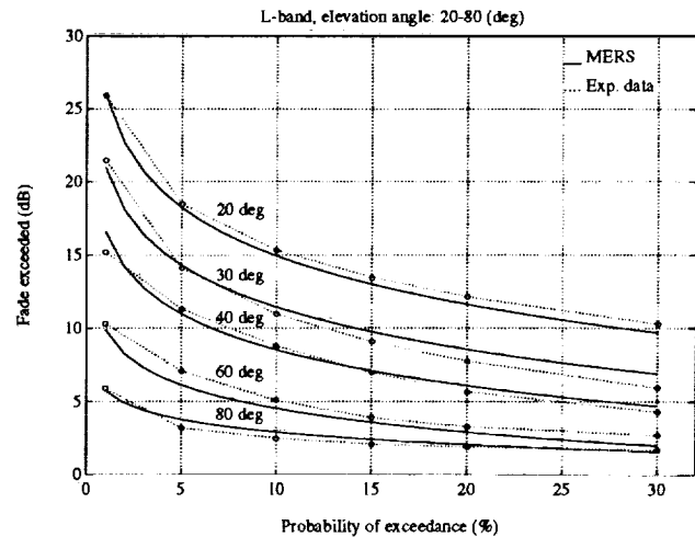
Fig. 1 MERS model vs. experimental data
