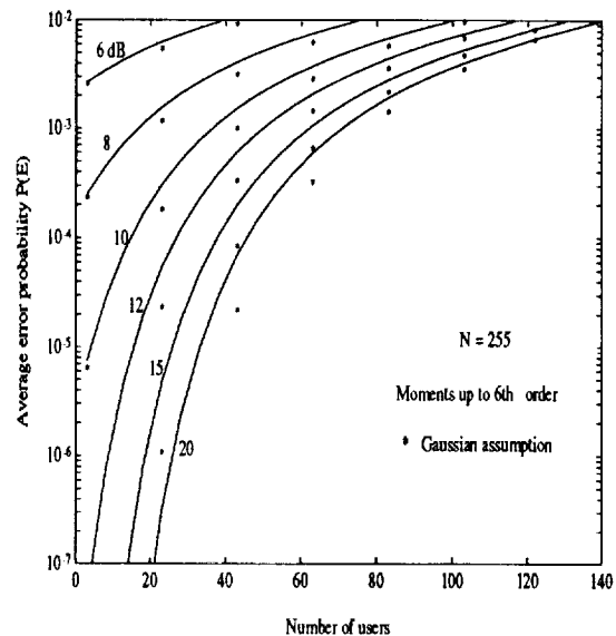
Figure 1: Average error probability P(E) versus the number of users for different values of the ratio E_b/N_0 for maximum-length sequences with N = 255 .
