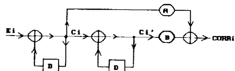
FIG. 4 EXAMPLE SECOND ORDER CONTROLLER
