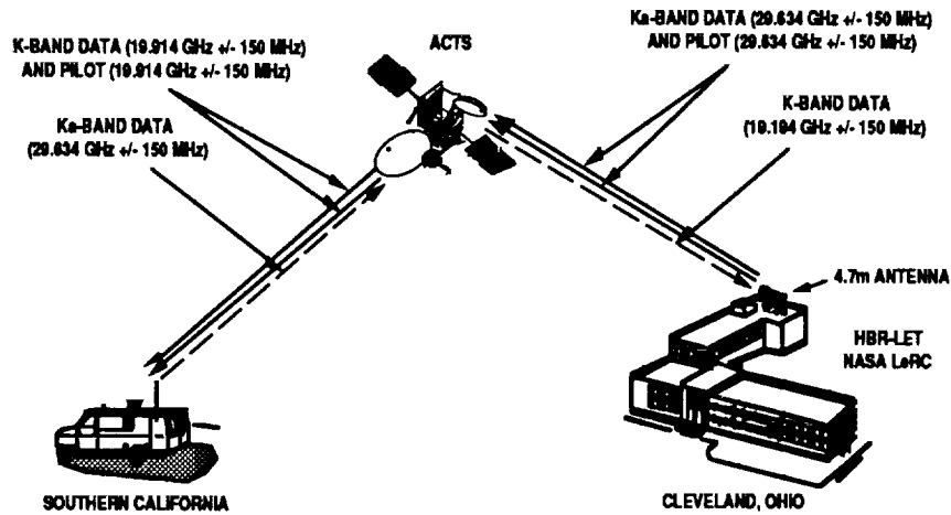
Figure 1 The AMT Experimental Setup
