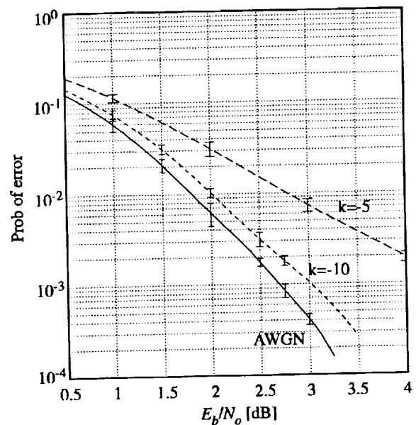
Figure 7. The average bit error rate versus the energy-per-bit-to-noise-spectral-density ratio for a single rate 1/2 code in Rician fading environments.
