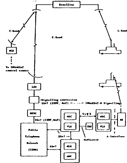
FIGURE 7. ARCHITECTURE OF INMARSAT-M INTEGRATED SERVICE
