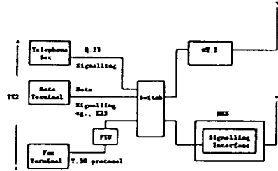
FIGURE 5. REAL-TIME TERMINAL FOR THE GSM INTERFACE
