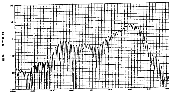
(a) elevation plane, gain = 11 dBic
