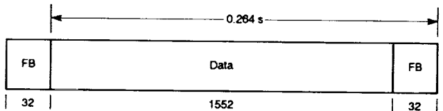
(c) 6 kbps Inmarsat-B/M TDM Signalling Channels
