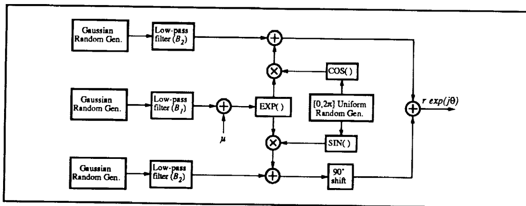
Figure 1: Land mobile satellite channel model.
