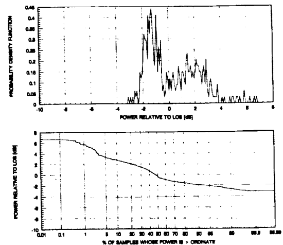
Fig. 5 PDF and CDF
