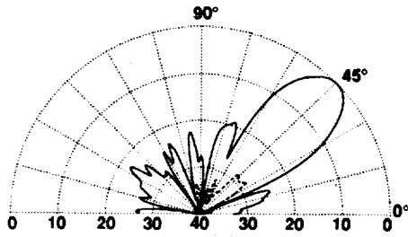
Fig. 6 Elevation Pattern, 20 GHz, Co- and X-pol.
