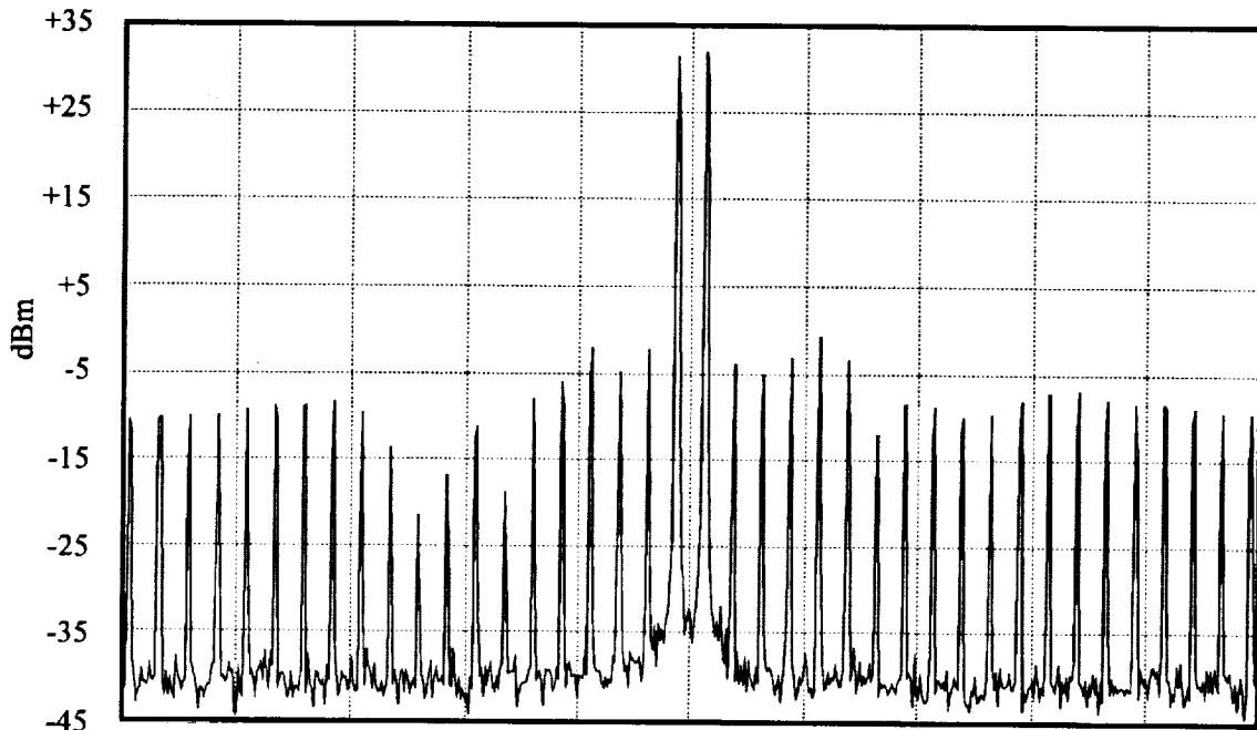
Centre Freq: 221 MHz Span: 2 MHz Res. B/W: 1 kHz Video B/W: 1 kHz Sweep: 6 s
