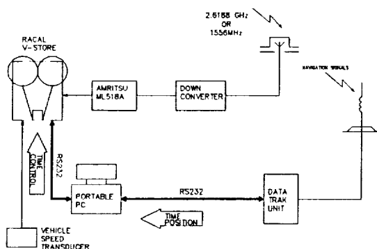
Figure 1- Mobile receiver system
