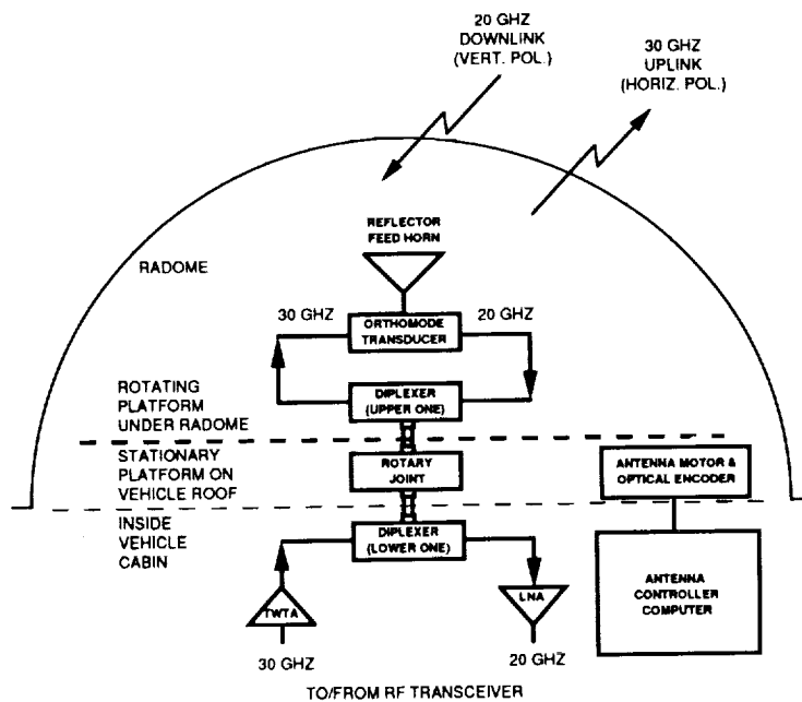
Fig. 3 Reflector Antenna Block Diagram
