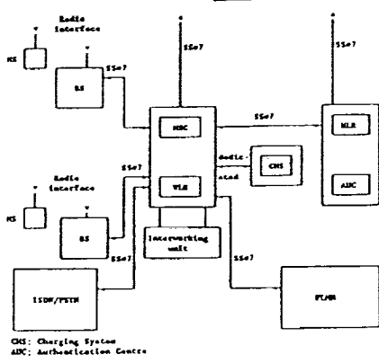
FIGURE 1. GSM NETWORK ARCHITECTURE
