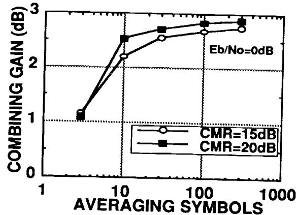
Figure 3 Relation between the Number of Symbols and Combining Gain
