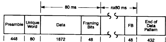
(a) 24 kbps Inmarsat-B SCPC Communications Channel
