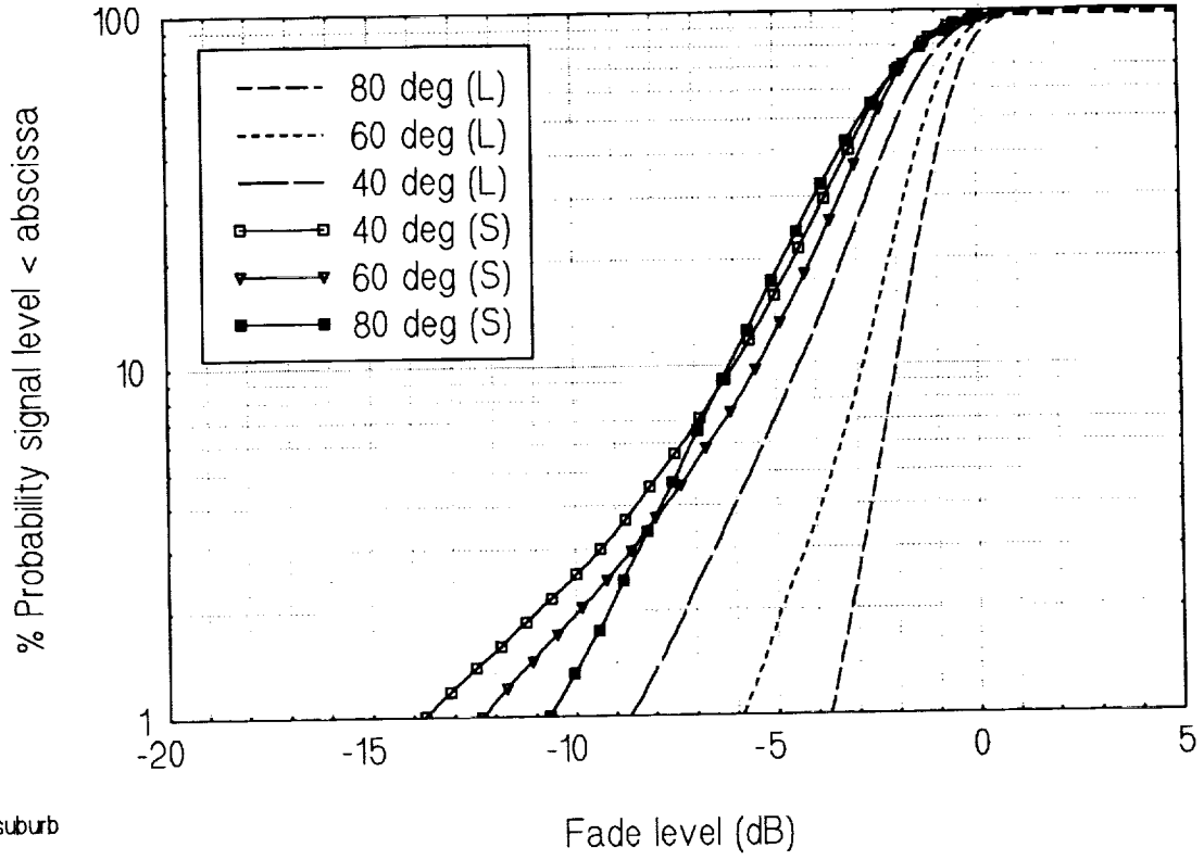
Figure 4 - Suburban area CDF's
