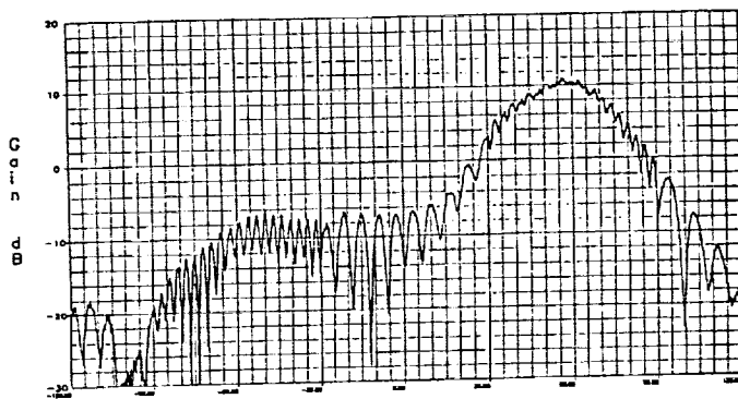
(a) elevation plane, gain = 13.4 dBic
