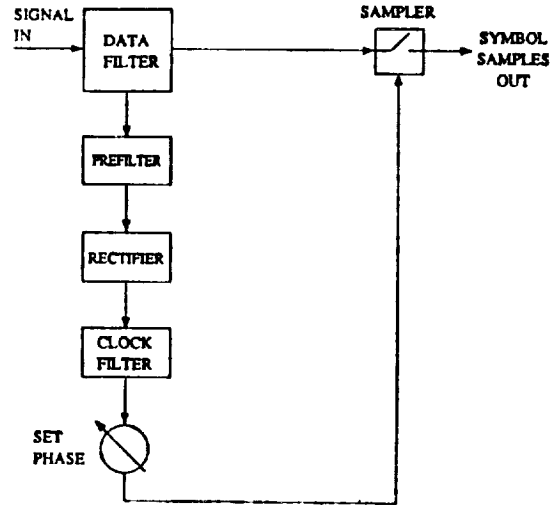
Figure 1: Feedforward clock recovery.
