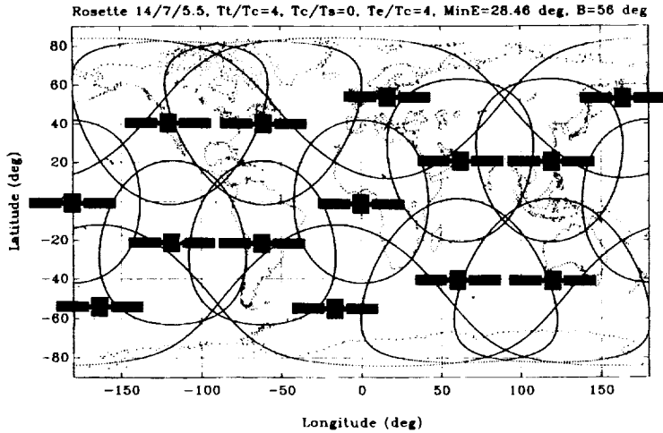
Fig. 1 MAGSS-14 Constellation (contours at 28.5^\circ )
