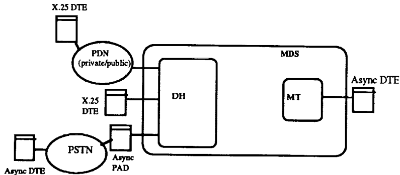
Figure 3. Asynchronous Data Service
