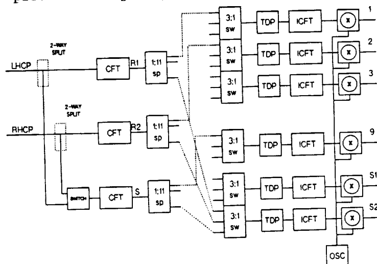
Figure 1. Option A CFT forward link configuration.
