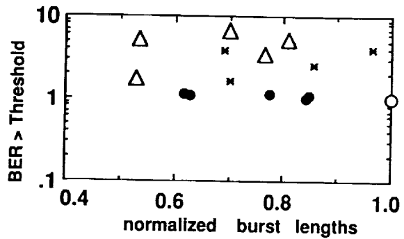
Figure 8. BER > threshold versus burst lengths normalized with the result of mode #4
