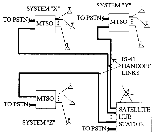
Figure 2: SHS connected to cellular as MTSO
