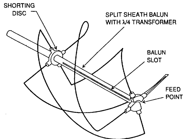
Fig. 1 4-arm helix (volute) antenna configuration
