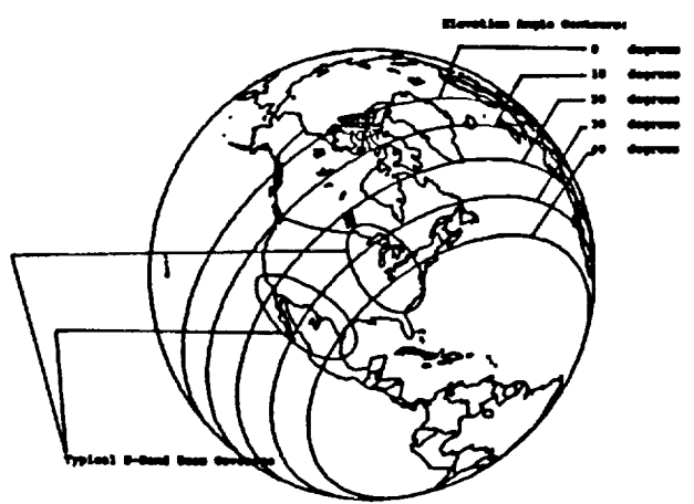
Figure 2. TDRES-1 Elevation Angle Contours From North America (Assuming a 62° West Longitude)
