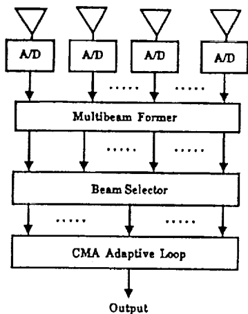
Figure 13. Consitution of the BSCMA.
