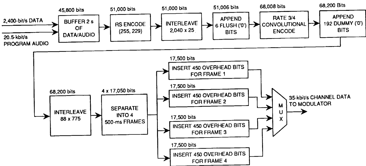
Figure 3. Frame Assembly
