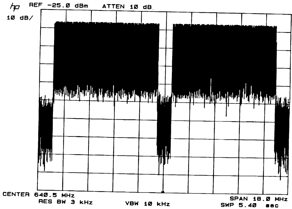
Figure 3. Noise Power Ratio measurement spectra from HP-FASS.
