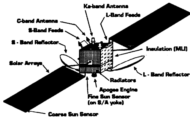
Figure 6: Odyssey Satellite
