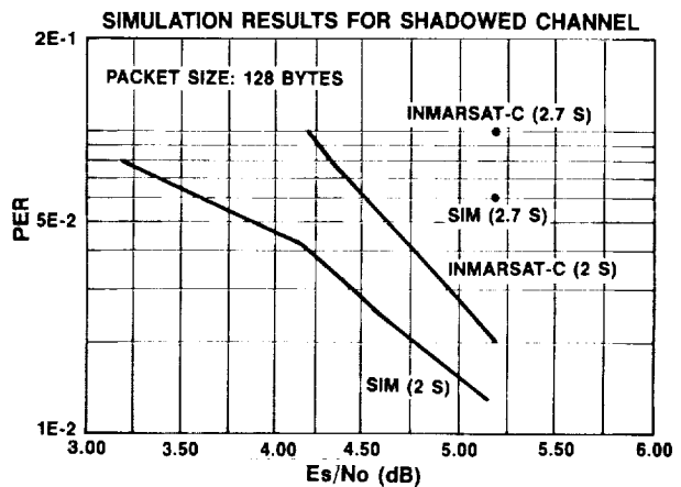
Figure 8. Blocked Channel Performance
