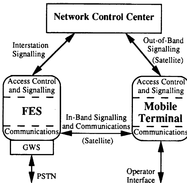
Figure 3. MSAT System Architecture
