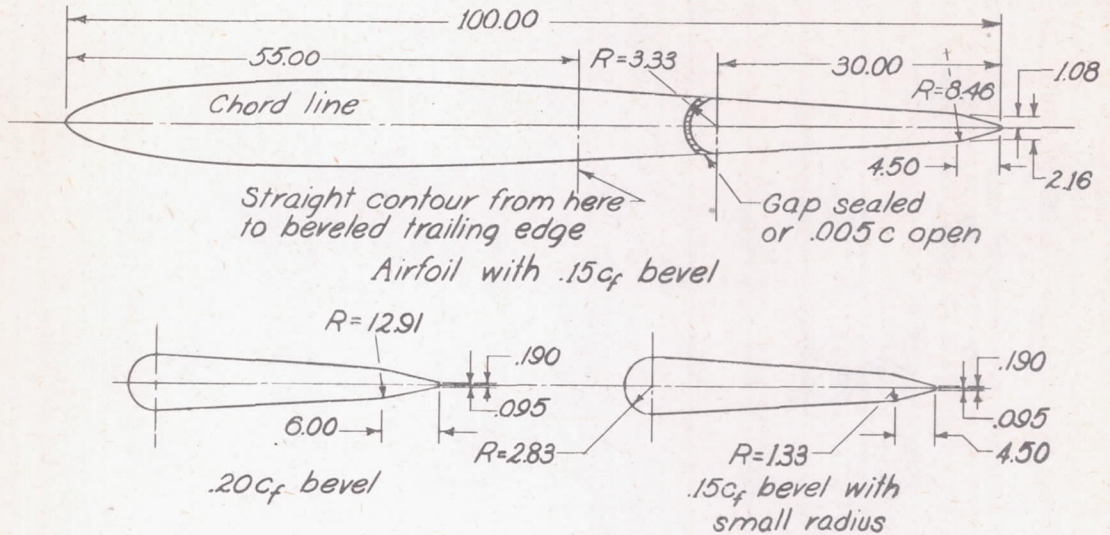
(a) Two-foot-chord NACA 0009 airfoil model with a 0.30c plain flap having 0.15 c_f and 0.20 c_f beveled trailing edges. Dimensions are in percent of airfoil chord.
