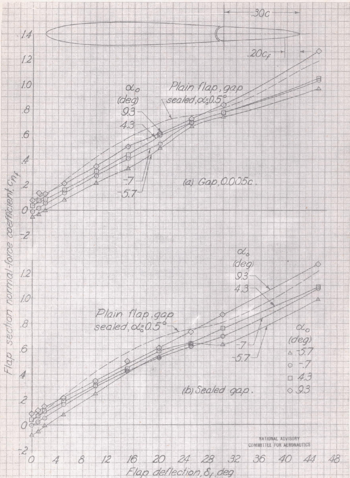
Figure 20. - Flap section normal-force coefficient as a function of the deflection of a 0.30c flap having a 0.20c f bevel on an NACA 0009 airfoil. The included angle at the trailing edge is 25.0°. Plain-flap data from reference 5.
