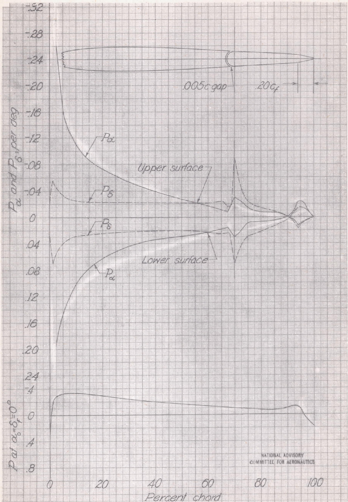
Figure 18 - Pressure-distribution characteristics of an NACA 0009 airfoil with a 0.30c flap having a 0.20c_f bevel, 0.005c gap.
