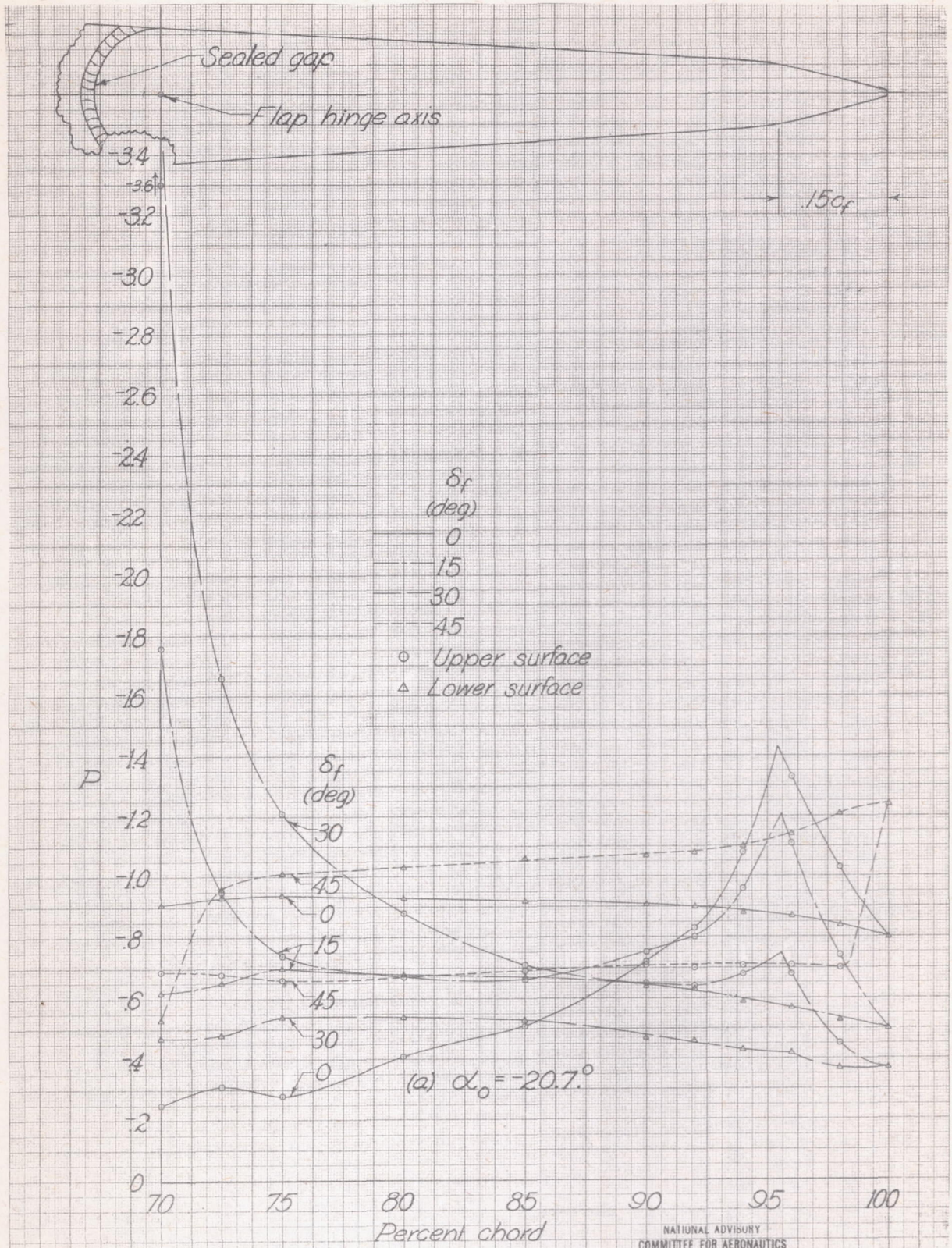
Figure 12.—Pressure distributions over a 0.30c flap having a 0.15c f bevel at various angles of attack and flap deflections. NACA 0009 airfoil; sealed gap.
