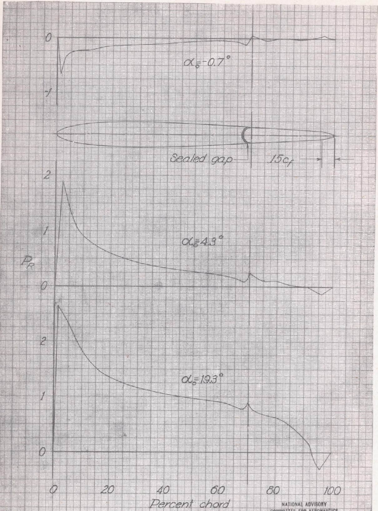
Figure 3. - Distribution of resultant pressure coefficient over the NACA 0009 airfoil at various angles of attack. c_f = 0.30c ; gap sealed; bevel chord = 0.15c_f ; \delta_f = 0^\circ .
