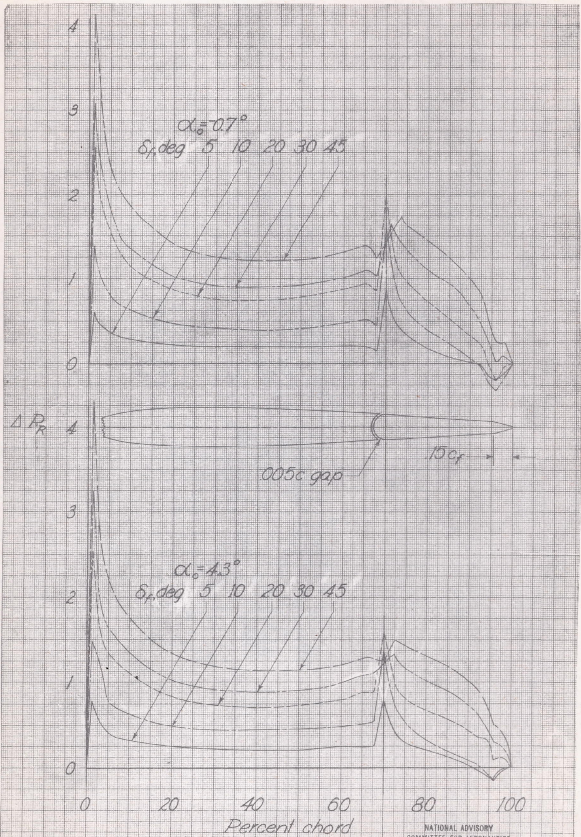
Figure 6. - Increments of resultant pressure coefficient over the NACA 0009 airfoil for various flap deflections at several angles of attack. c_f = 0.30c ; gap = 0.005c; bevel chord = 0.15c f .
