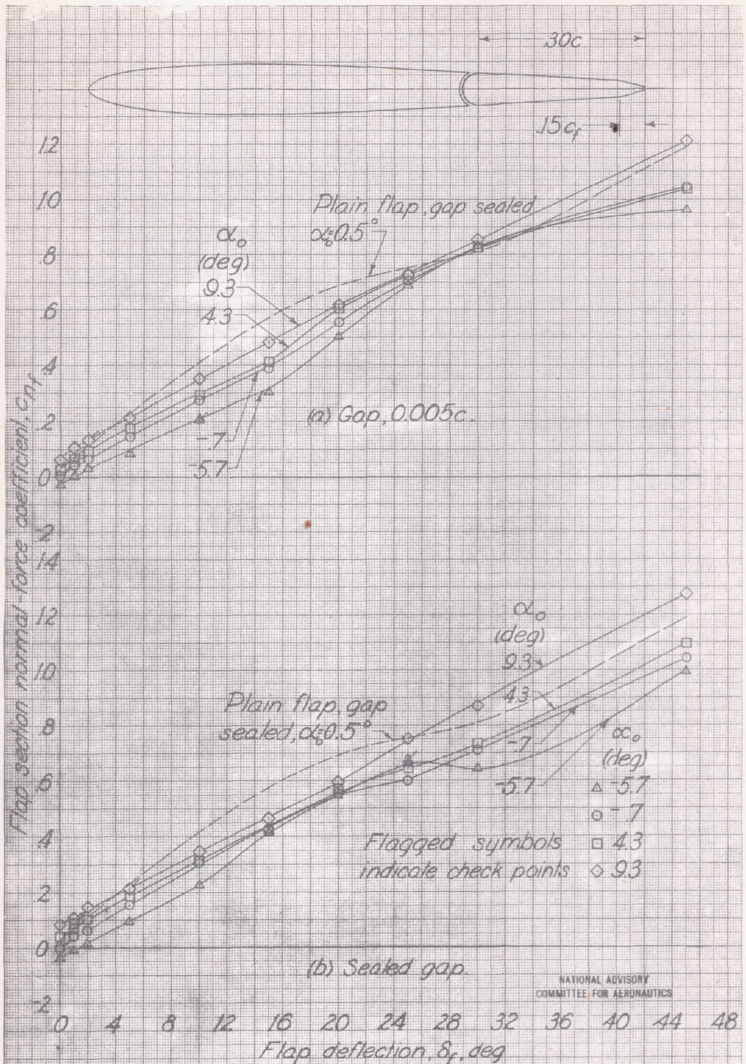
Figure 19 - Flap section normal-force coefficient as a function of the deflection of a 0.30c flap having a 0.15c f bevel on an NACA 0009 airfoil. The included angle at the trailing edge is 30.4°. Plain-flap data from reference 5.
