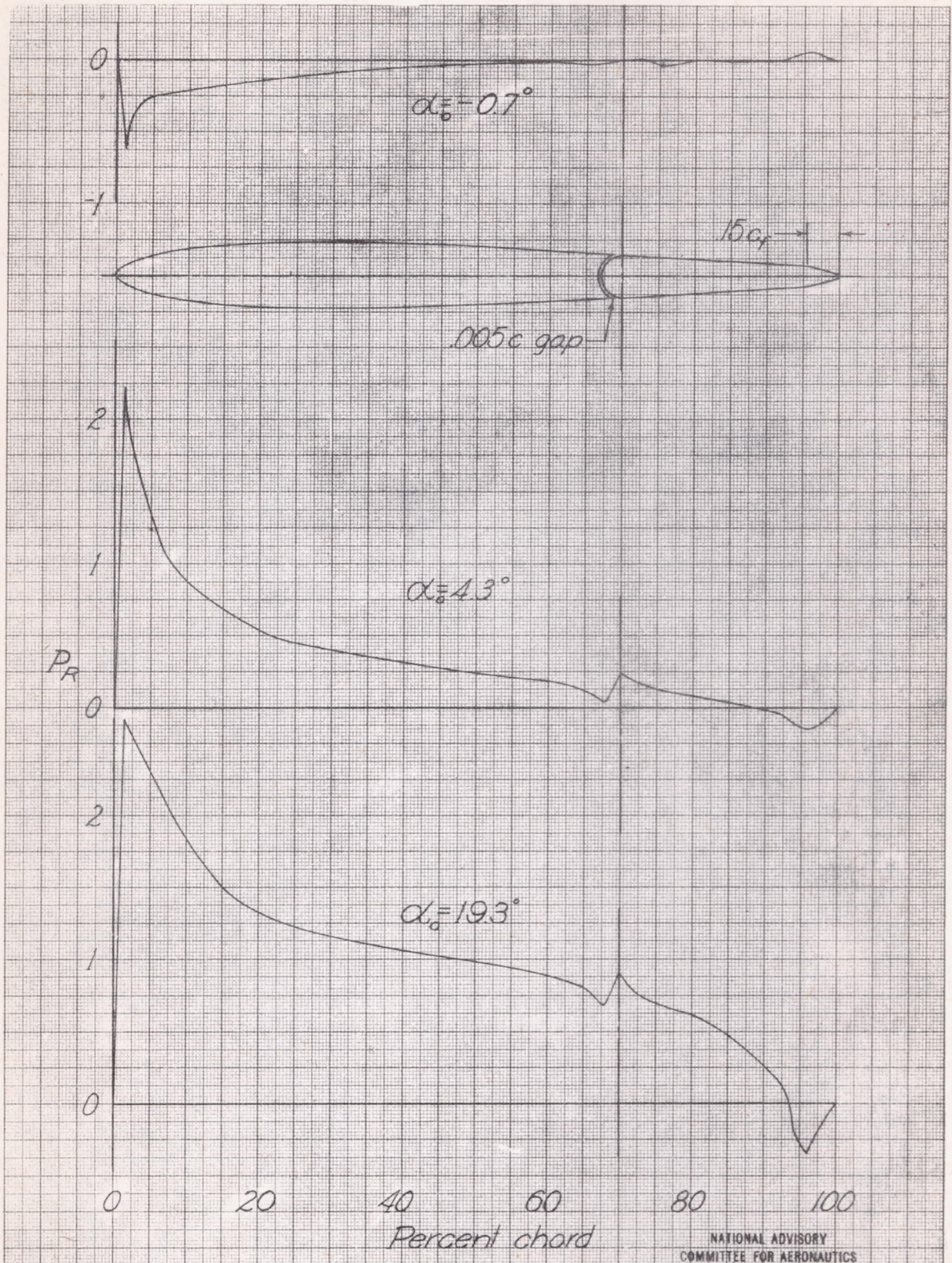
Figure 5. - Distribution of resultant pressure coefficient over the NACA 0009 airfoil at various angles of attack c_f = 0.30c ; gap = 0.005c ; bevel chord = 0.15c_f ; \delta_x = 0^\circ .
