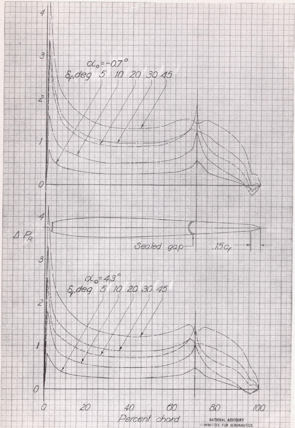
Figure 4 - Increments of resultant pressure coefficient over the NACA 0009 airfoil for various flap deflections at several angles of attack. c_f = 0.30c ; gap sealed; bevel chord = 0.15c_f .
