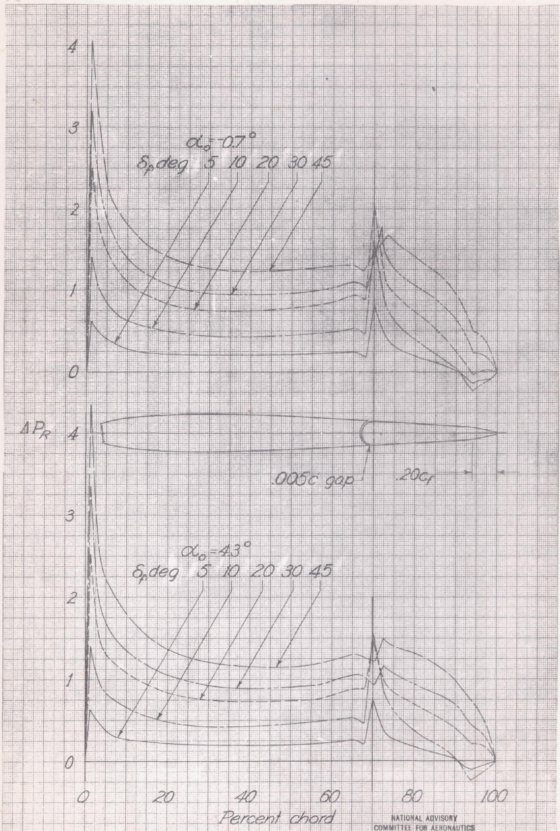
Figure 10.-Increments of resultant pressure coefficient over the NACA 0009 airfoil for various flap deflections at several angles of attack. c_f = 0.30c ; gap = 0.005c ; berel chord = 0.20c_f .
