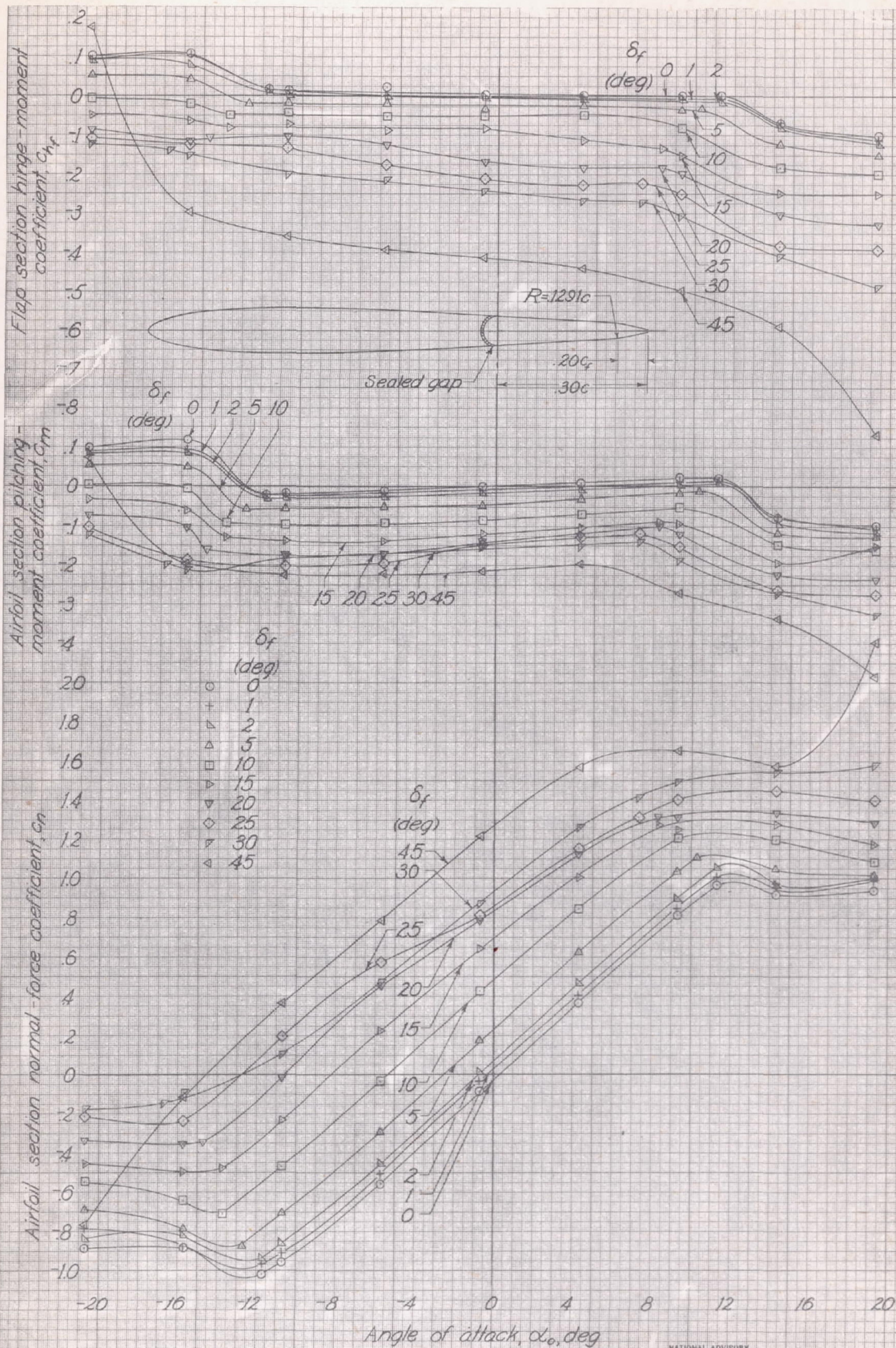
(a) Sealed gap Figure 23. - Section characteristics of the NACA 0009 airfoil with a 0.30c flap having a 0.20c f bevel Bevel radius, 0.1291c; included angle at trailing edge, 25.0°.
