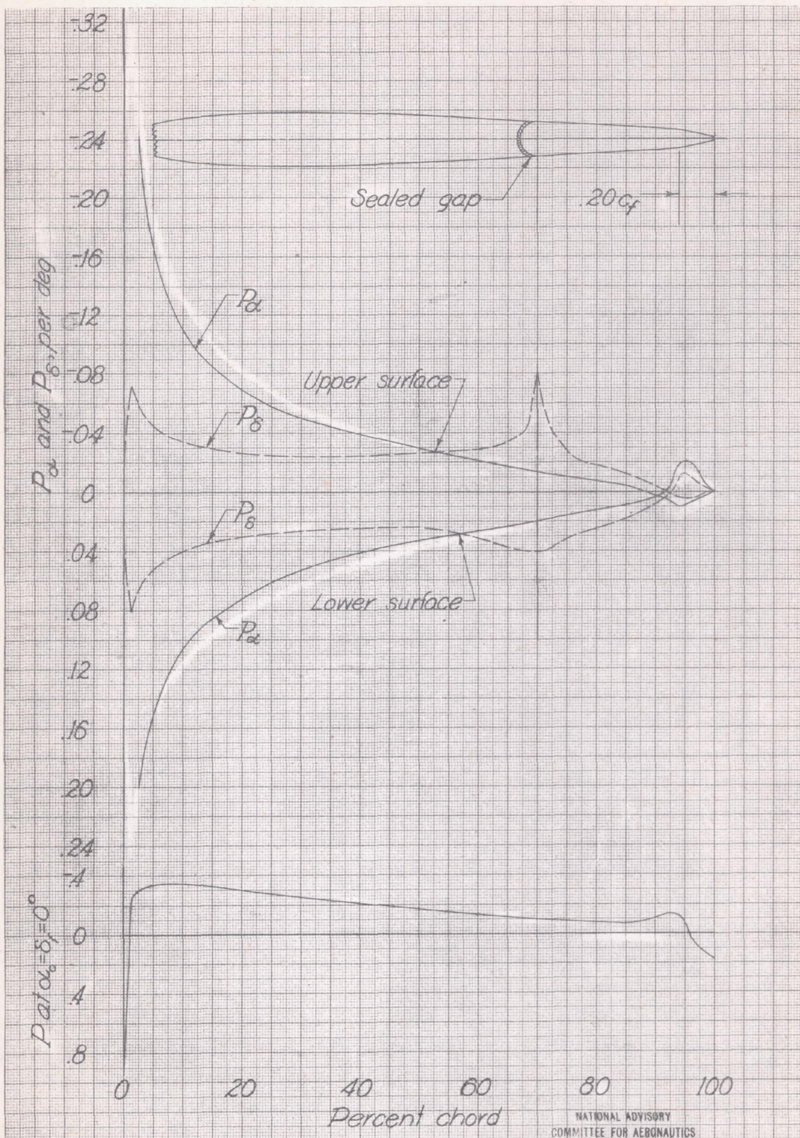
Figure 17. - Pressure-distribution characteristics of a NACA 0009 airfoil with a 0.30c flap having a 0.20c f bevel. Sealed gap.
