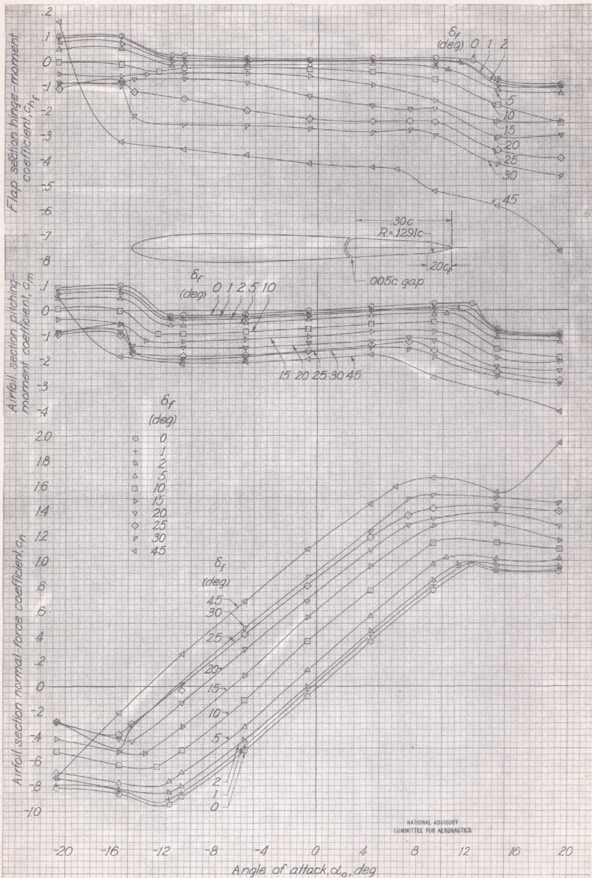
(b) Gap, 0.005c. Figure 23.-Concluded.
