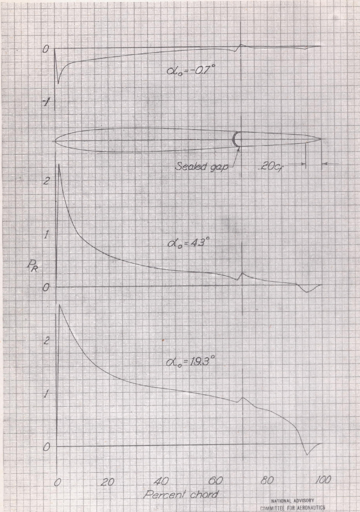
Figure 7.-Distribution of resultant pressure coefficient over the NACA 0009 airfoil at various angles of attack. c_f = 0.30c ; gap sealed; bevel chord = 0.20c_f ; \delta_f = 0^\circ .
