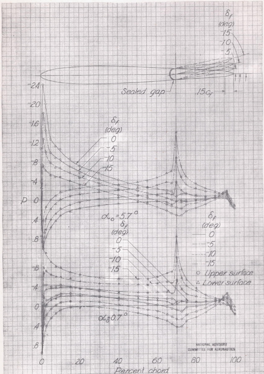
Figure 21. - Pressure distribution for various combinations of \alpha_0 and \delta_f which might occur on horizontal tail of typical dive bomber in highly accelerated maneuvers at various speeds. NACA 0009 airfoil; 0.30c_f flap; sealed gap; 0.15c_f bevel.
