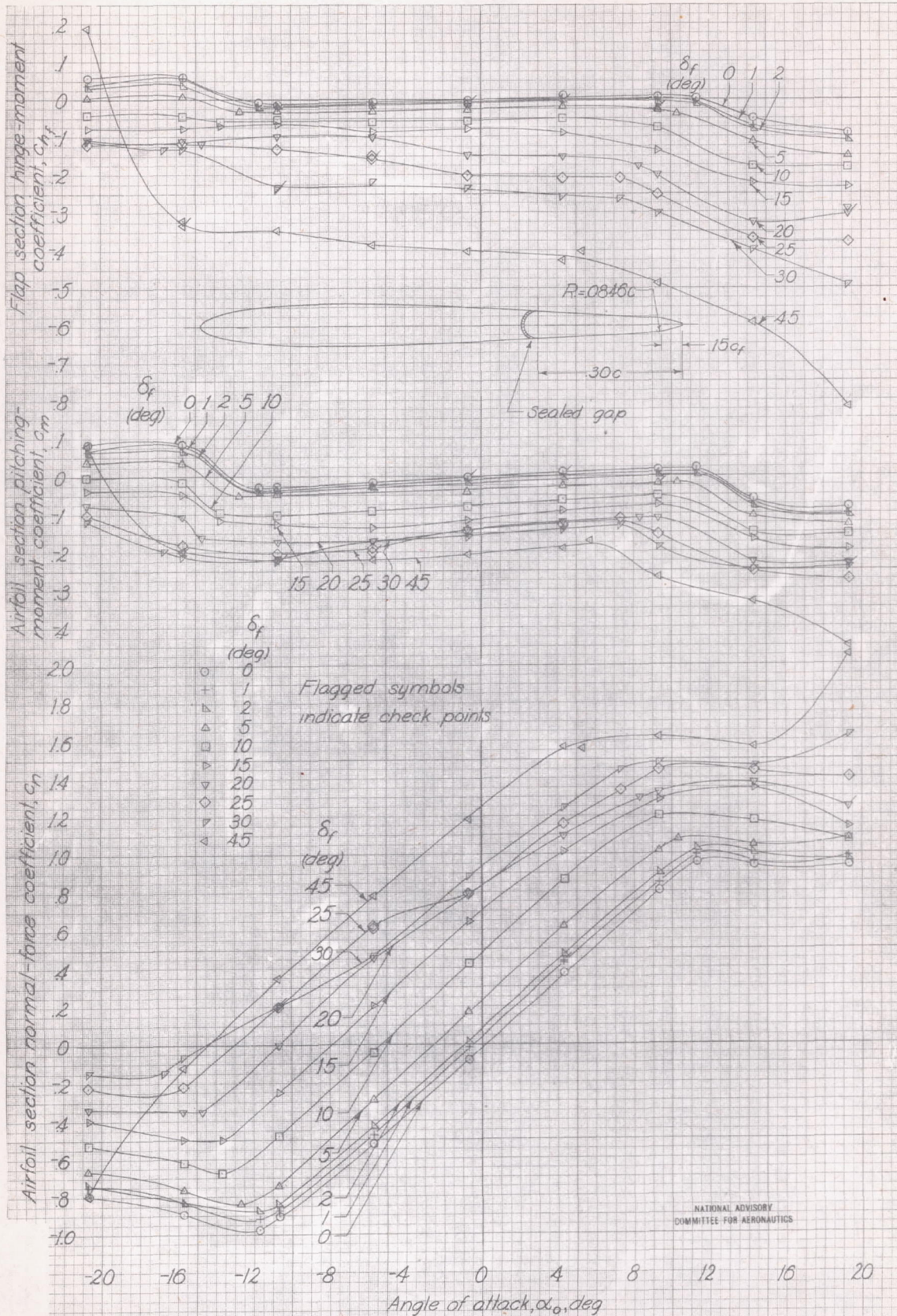
Figure 22. - Section characteristics of the NACA 0009 airfoil with a 0.30c flap having a 0.15c_f bevel. Bevel radius, 0.0846c ; included angle at the trailing edge, 30.4^\circ .
