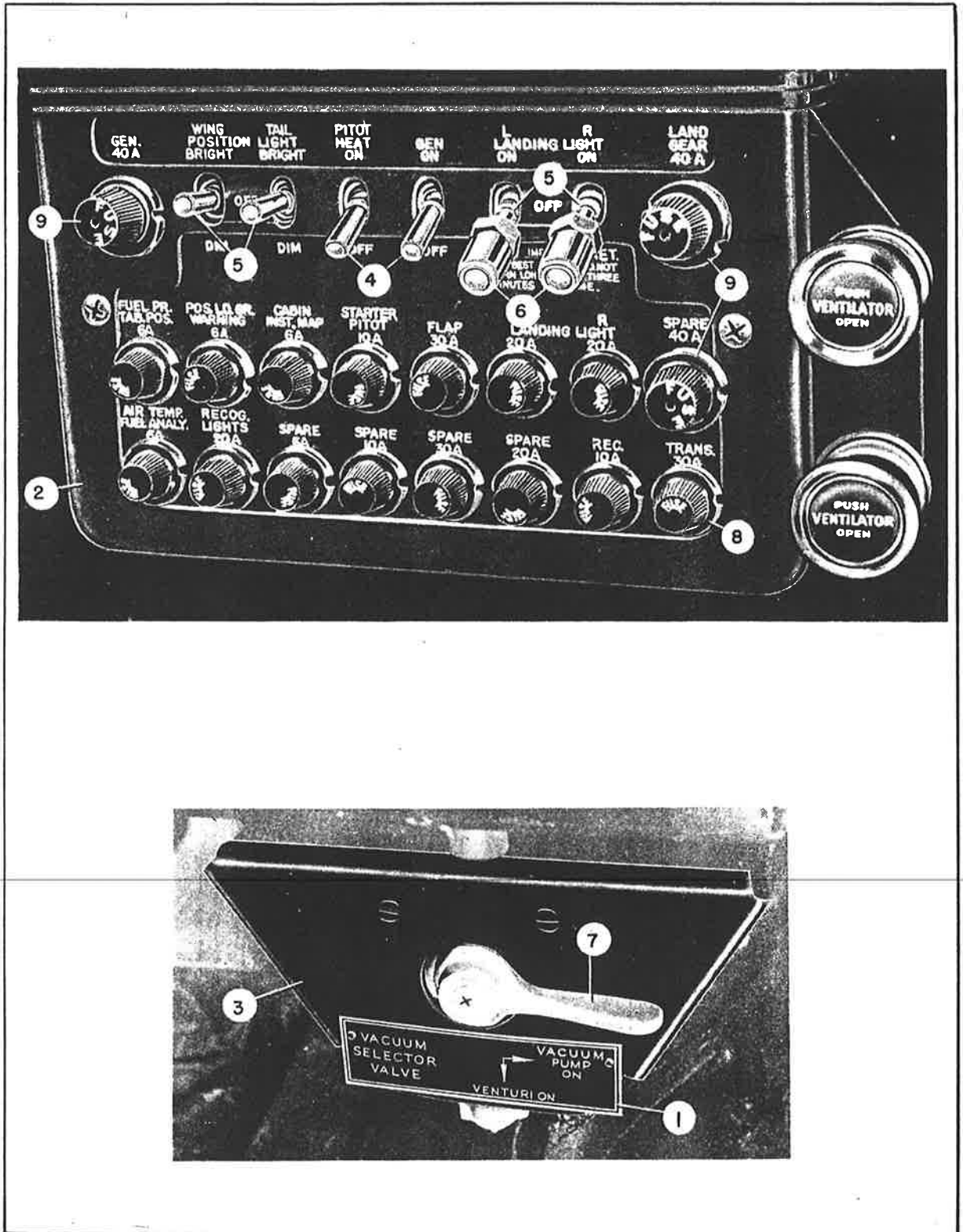
Figure 38 - Lower Auxiliary Panel Assembly
