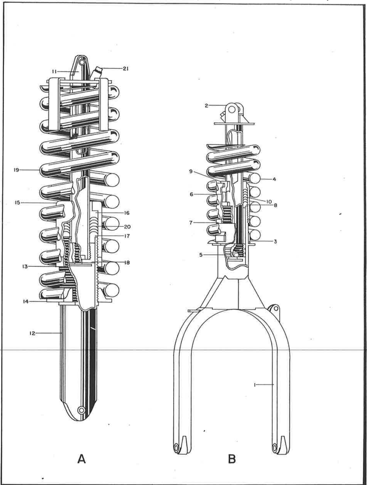
Figure 15 - Main Landing Gear and Tail Wheel Shock Struts
