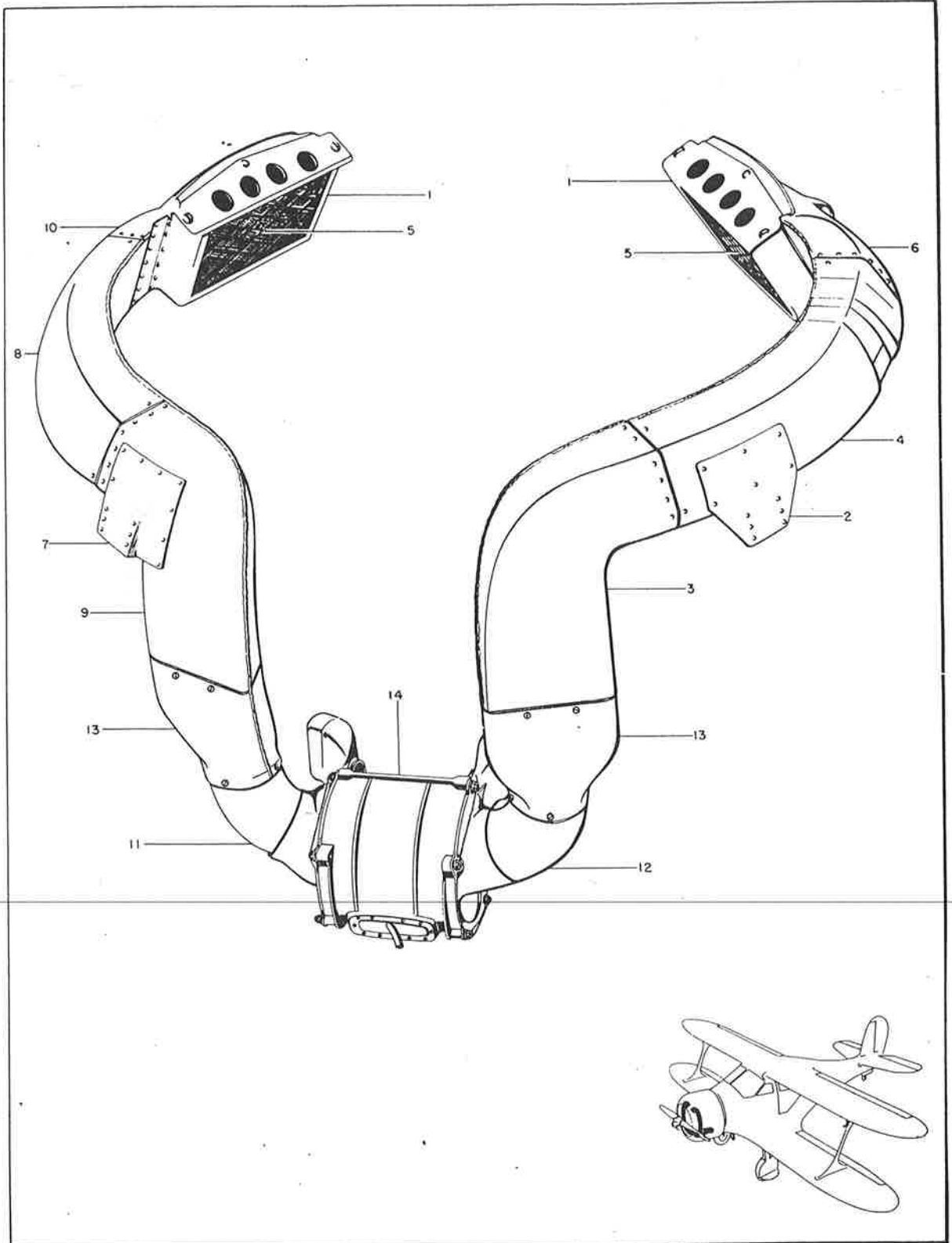
Figure 22 - Carburetor Air Duct Assembly
