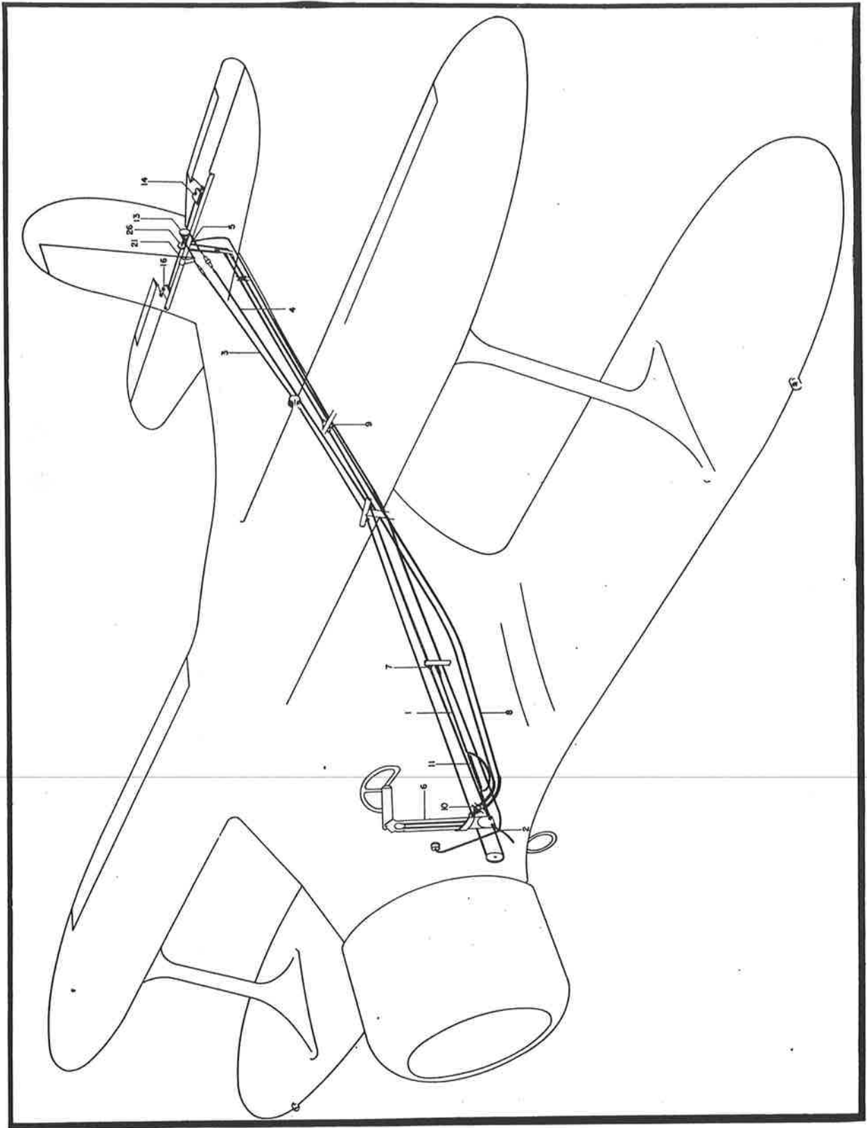
Figure 16 - Elevator and Tab Control Assembly
