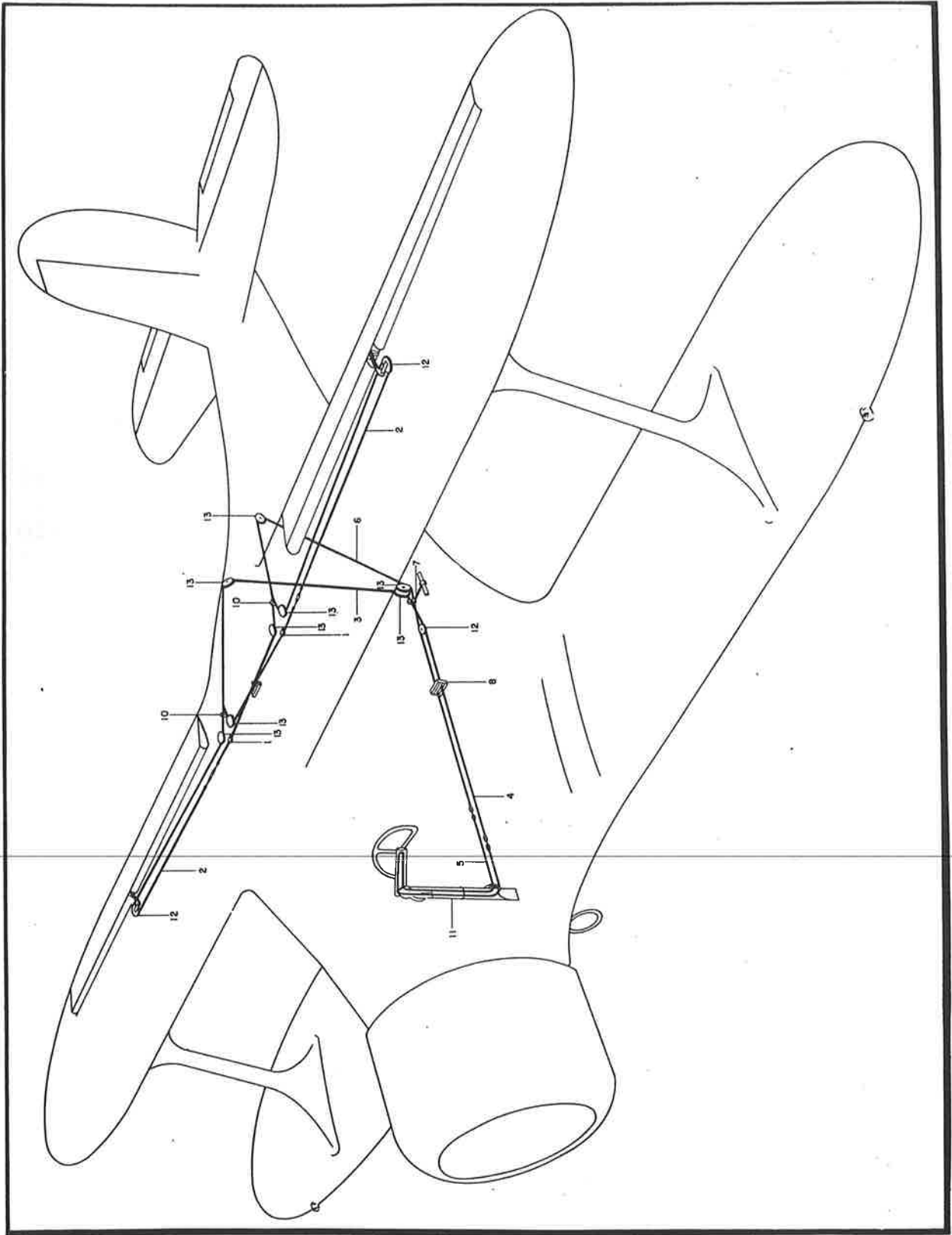
Figure 17 - Aileron Control Assembly
