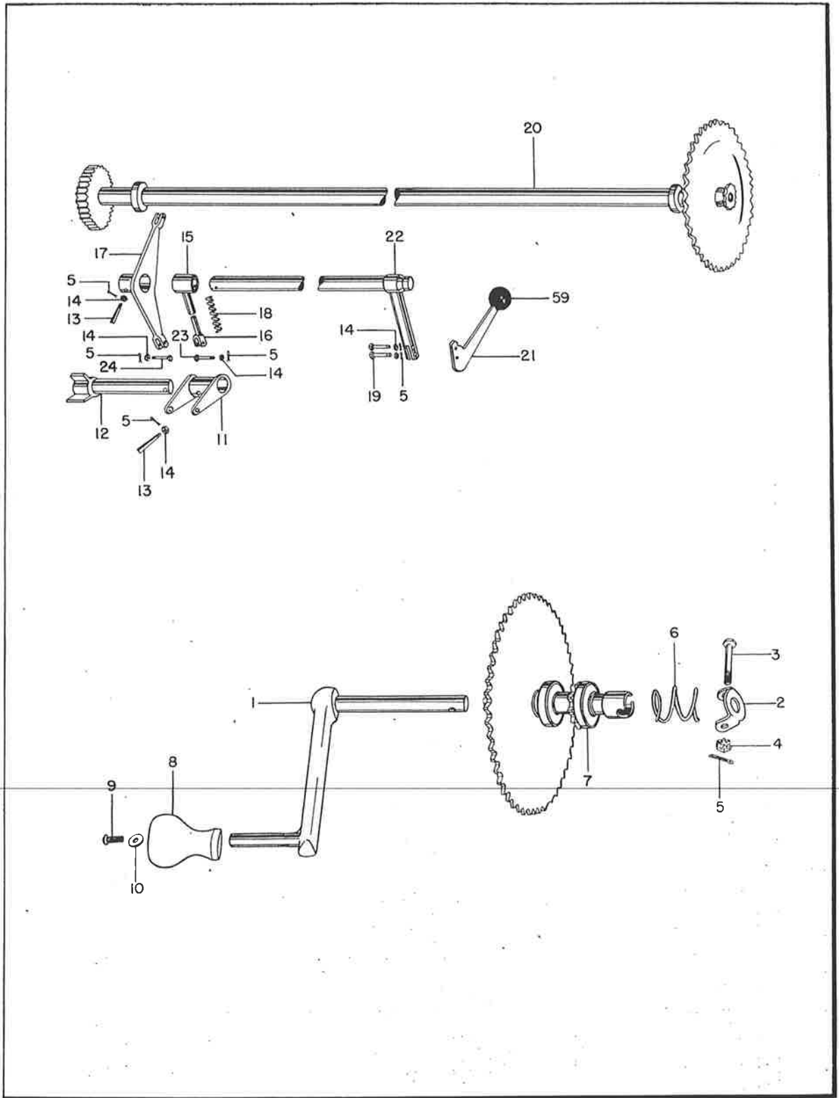
Figure 16 - Landing Gear Handcrank and Cross Shaft Assembly
