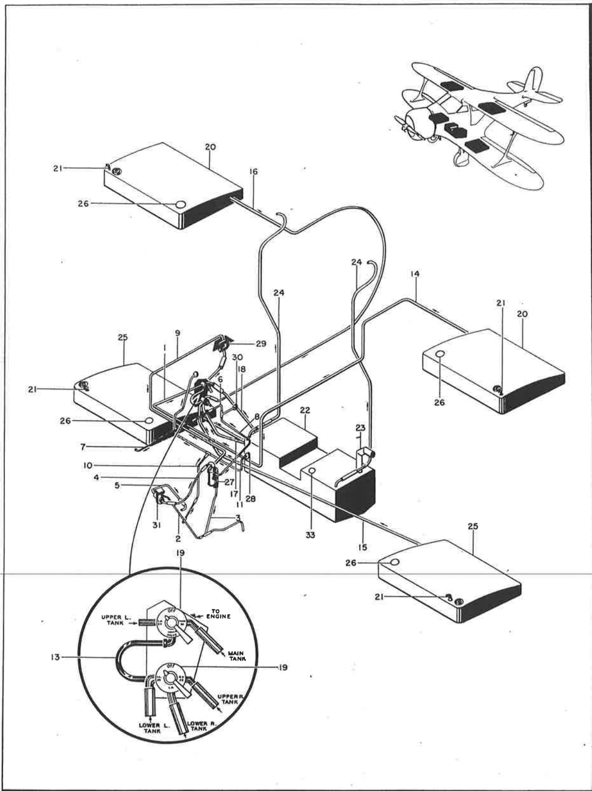
Figure 27 - Installation - Fuel System
