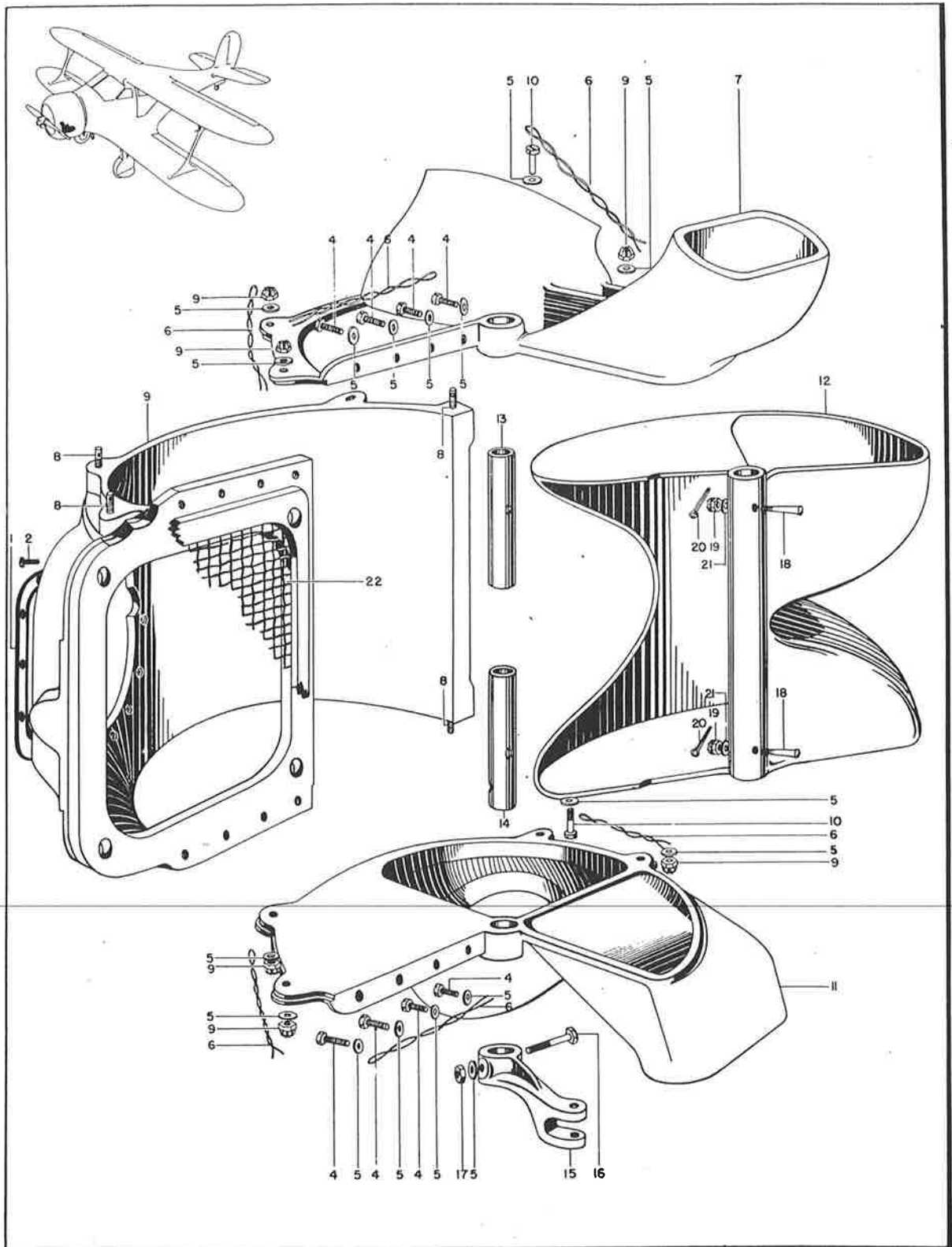
Figure 23 - Carburetor Air Scoop Assembly
