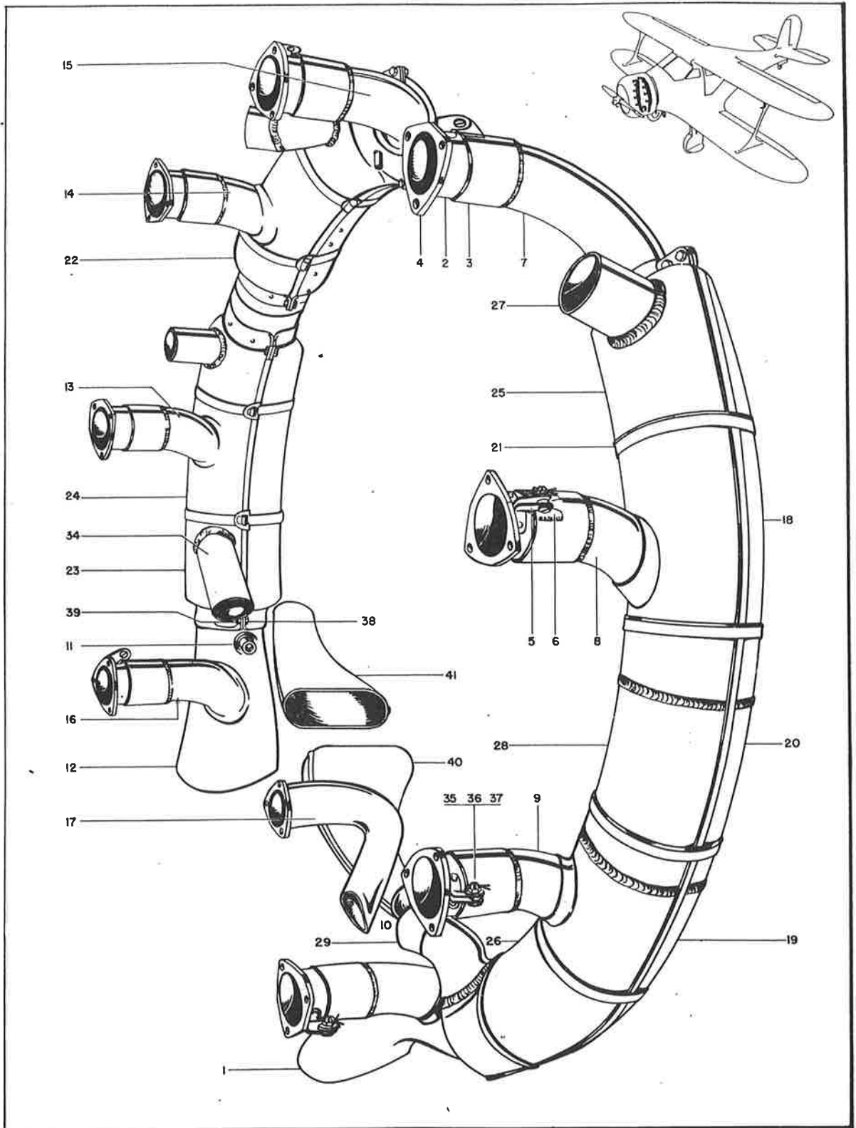
Figure 24 - Exhaust Stack and Heater Muff Assembly
