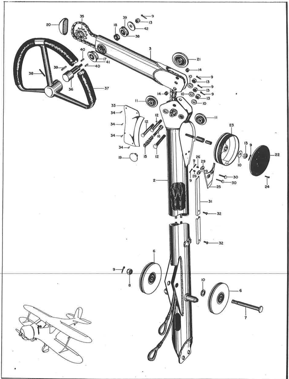
Figure 20 - Control Column Assembly
