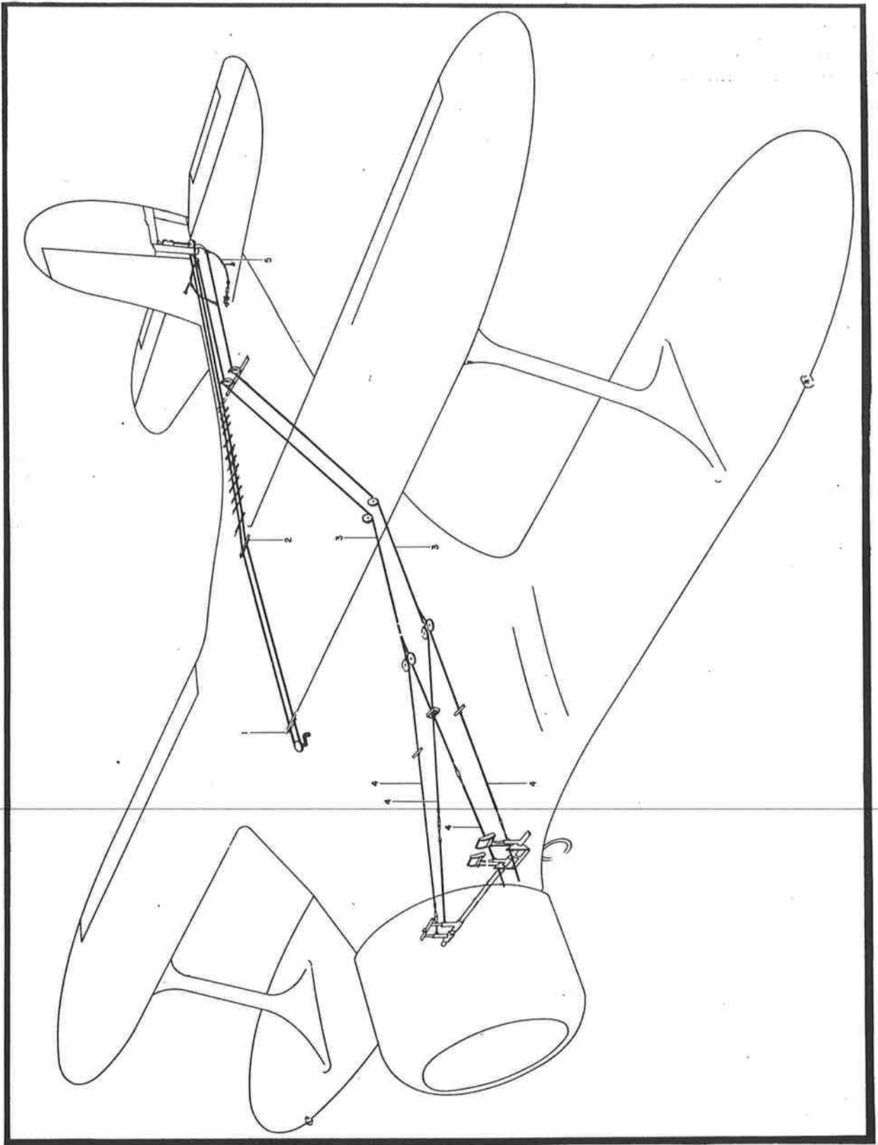
Figure 19 - Rudder and Tab Control Assembly
