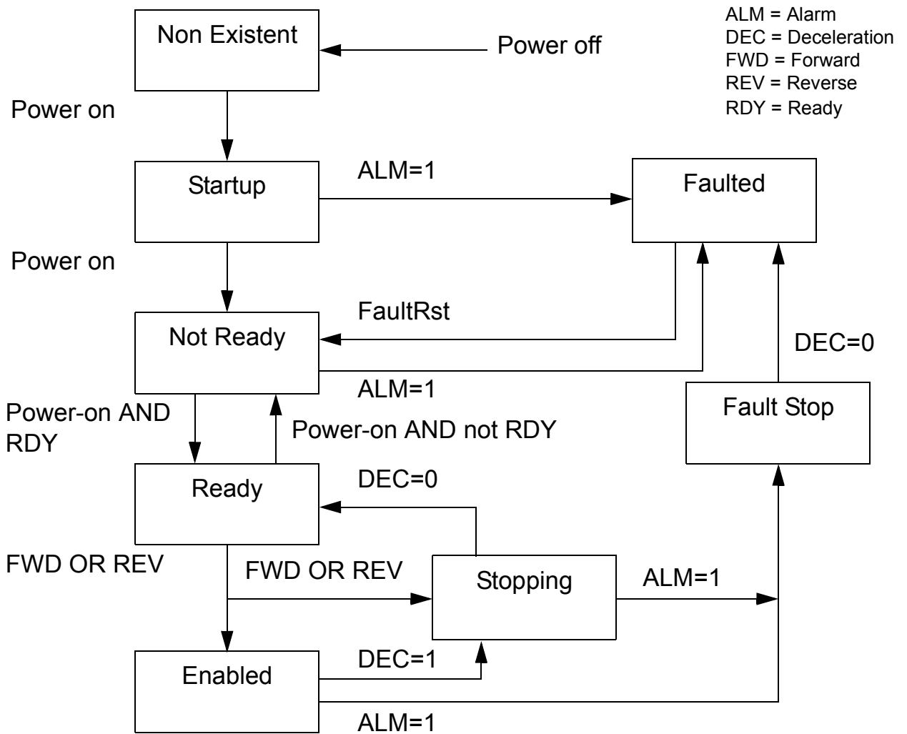
Figure 10. ODVA state transition diagram Speed Actual (AC/DC Drive Object)
