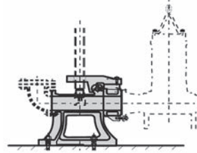
KIT LL 80/100/125/150
