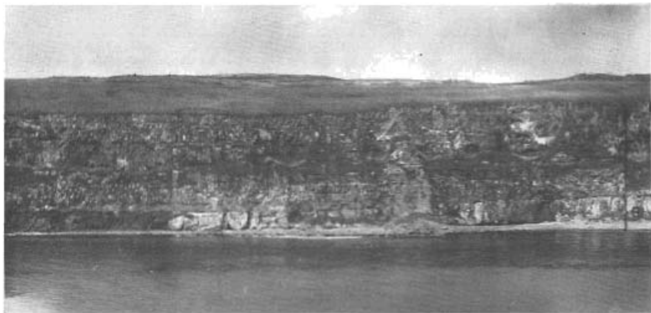
FIGURE 26.—Sea bluff north of Garden Cove showing flows, silt and tabular pediments (L) and overlying peridotite basement (B). Photograph by U. S. Navy.
