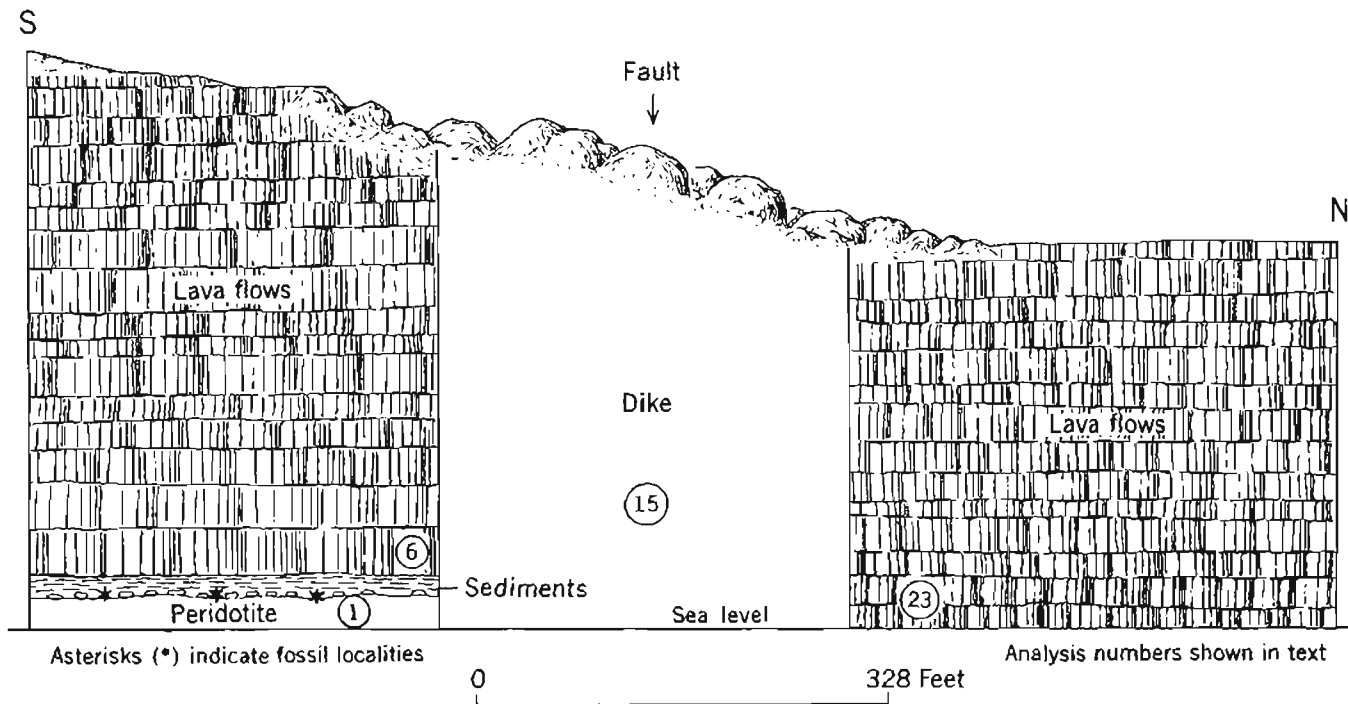
FIGURE 20.—Section about two-thirds of a mile south of Tolstoi Point, St. George Island. Numbers correspond to those of the analyzed rocks. No. 23 is described on page 115.
