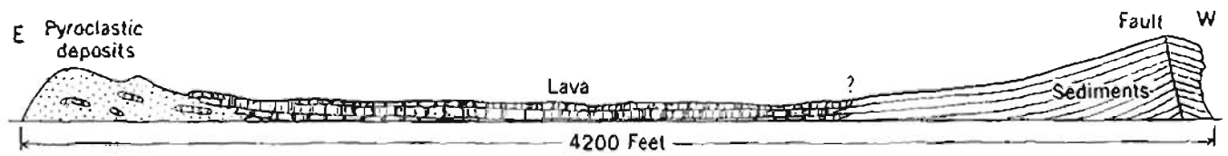
FIGURE 20.—Section of Otter Island. From east to west are pyroclastic rocks, lava, and sedimentary rocks.
