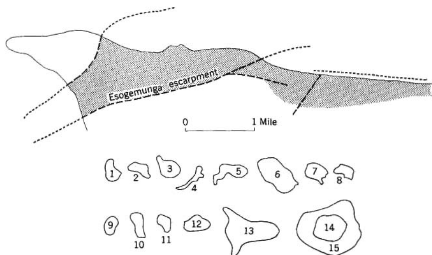
FIGURE 34.—The tuff conduit at Esogemunga, St. George Island (diagonally hatched) compared with tuff necks from Kimberley, South Africa (1-8) and from Schwaben, Germany (9-15). 1, Bulfontein; 2, Weselton; 3, Kaffyfontein; 4, Ottos-Kopje; 5, Du Toitspan; 6, Premier; 7, Jagersfontein; 8, De Beers; 9, Grafenberg; 10, Florian; 11, Metzinger-Weinberg; 12, Neuhauser; 13, Jusi; 14, Limburg; 15, Randecker Maar. (1-15 after H. Cloos, 1941).
