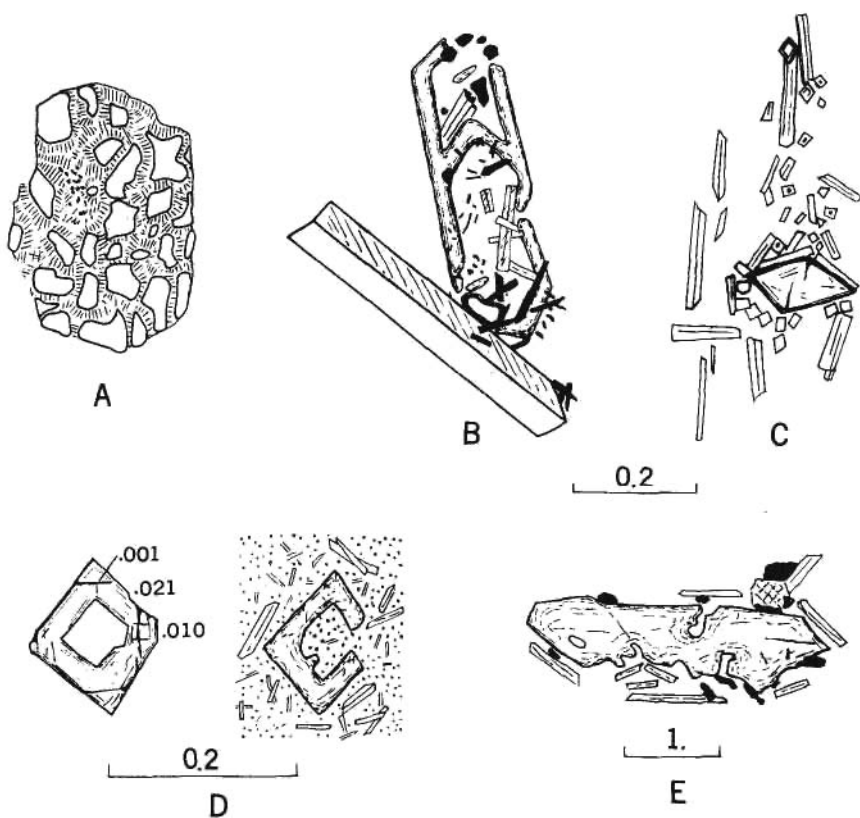
FIGURE 28.—Minerals in lavas. A , Serpentinized olivine from peridotite, Garden Cove, rock sample 1. B , Olivine, serpentine, and a small amount of magnetite. B , Olivine crystal in a state of resorption from plagioclase-hematite rock sample 18, top of road between village and Zapadni Bay, St. George Island. Olivine, plagioclase and hematite. C , Olivine phenocrysts and plagioclase laths illustrating preferred orientation in feldspathic basanite from rock sample 9 northeast shore of Otter Island. D , Hollow phenocrysts of olivine, plagioclase laths, and black pigments of magnetite in glass groundmass. Basanite rock sample 17 intrusive into Rush Hill, St. Paul Island. E , Resorbed olivine phenocryst in fluidal glass ground-mass). Basanite flow, Tolstoi Point, St. Paul Island. Scales in millimeters.
