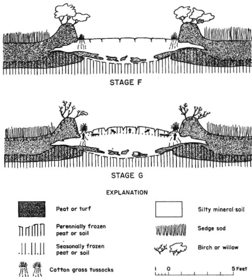
FIGURE 28.—Diagrammatic sketches showing evolution of a peat ring. Stage A , Unusually warm summer. In most areas depth of thaw does not extend below base of peat, but mineral soil is thawed in a few areas where peat is exceptionally thin. Stage B , Late autumn, same year. Thawed mineral soil expands upon freezing and breaks overlying thin cover of peat, initiating a frost scar. Stage C , Early autumn, several years later. Frost scar has been enlarged by shoving aside of peat at margins of bare soil area. Surface of scar expands upward as surface layers of soil freeze and expand. Dilation cracks (miniature zellenboden) are formed. Stage D , Late autumn, several years later. After surface layers of soil have frozen, a hard cover of frozen soil resists further uparching. Continued expansion resulting from freezing of deeper layers of soil is relieved by lateral thrusting. Ridge of peat is raised around bare soil center. Stage E , Late autumn, several years later. Ridge of perennially frozen ground beneath the peat ridge and thick layer of seasonally frozen ground in peat at the surface prevent further widening of the bare soil area by lateral thrusting. Instead, lateral expansion of soil center results in intrusion of masses of silt into peat of the ridges, forcing some of the peat to move in the opposite direction along the surface of the frozen ground beneath the frost scar. Stage F , Summer, several years later. Seedlings of cottongrass take root at inner edge of peat ridge. Stage G , Early autumn, same year. Bare soil has frozen to a depth of several inches, but soil beneath tussocks is still thawed. Lateral expansion forces freezing soil beneath tussocks, heaving them upward. Peat ridge no longer affected by lateral thrusting from soil center.
