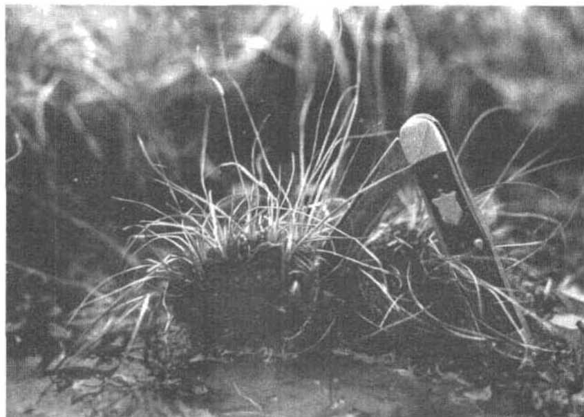
FIGURE 20.—Vertical section through seedling tussock of cottongrass. Note rhizomes resting directly in mineral soil and lack of winterkilled leaves.
