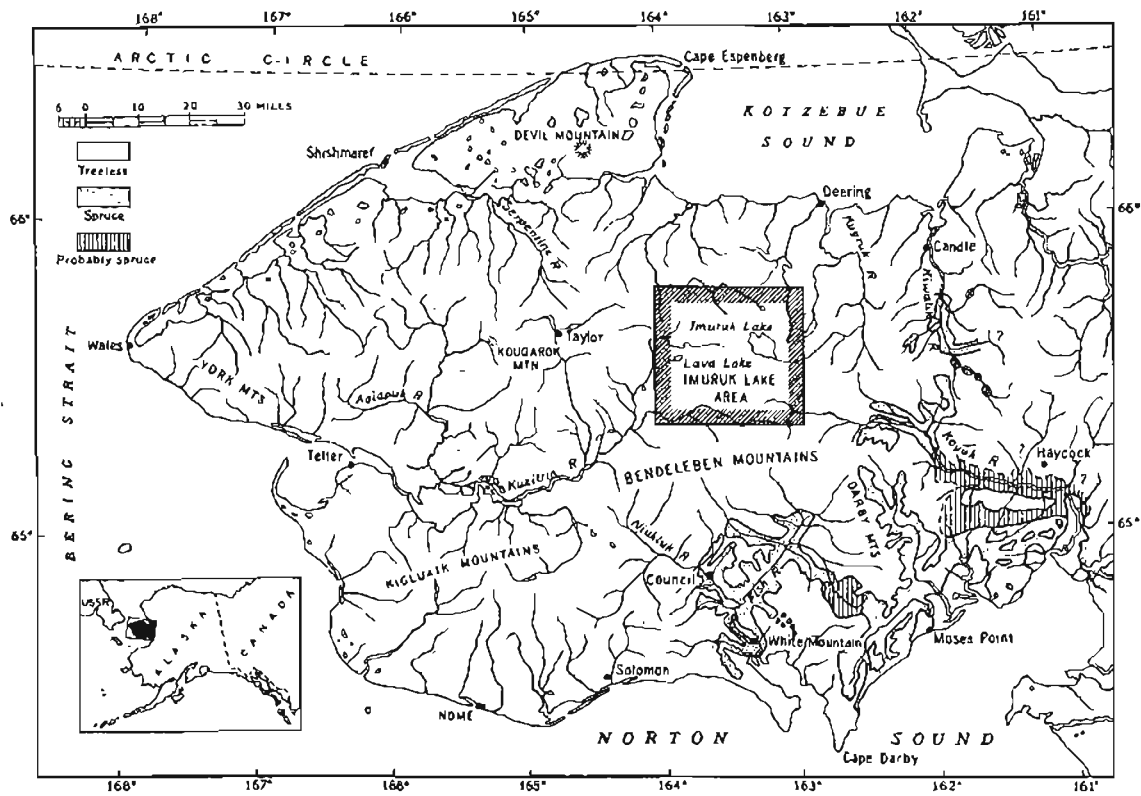
FIGURE 18.—Index map of Seward Peninsula, Alaska, showing location of Imuruk Lake area and distribution of forested areas.
