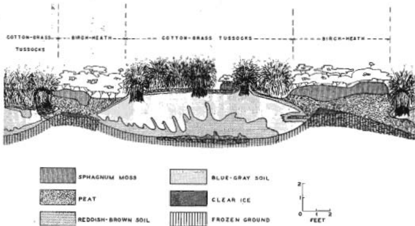
FIGURE 50.—Cross section through a tussock-birch heath polygon.
