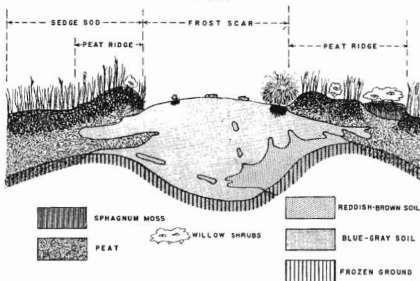
CROSS SECTION
