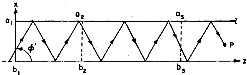
(b) UNFOLDED SIDE VIEW
