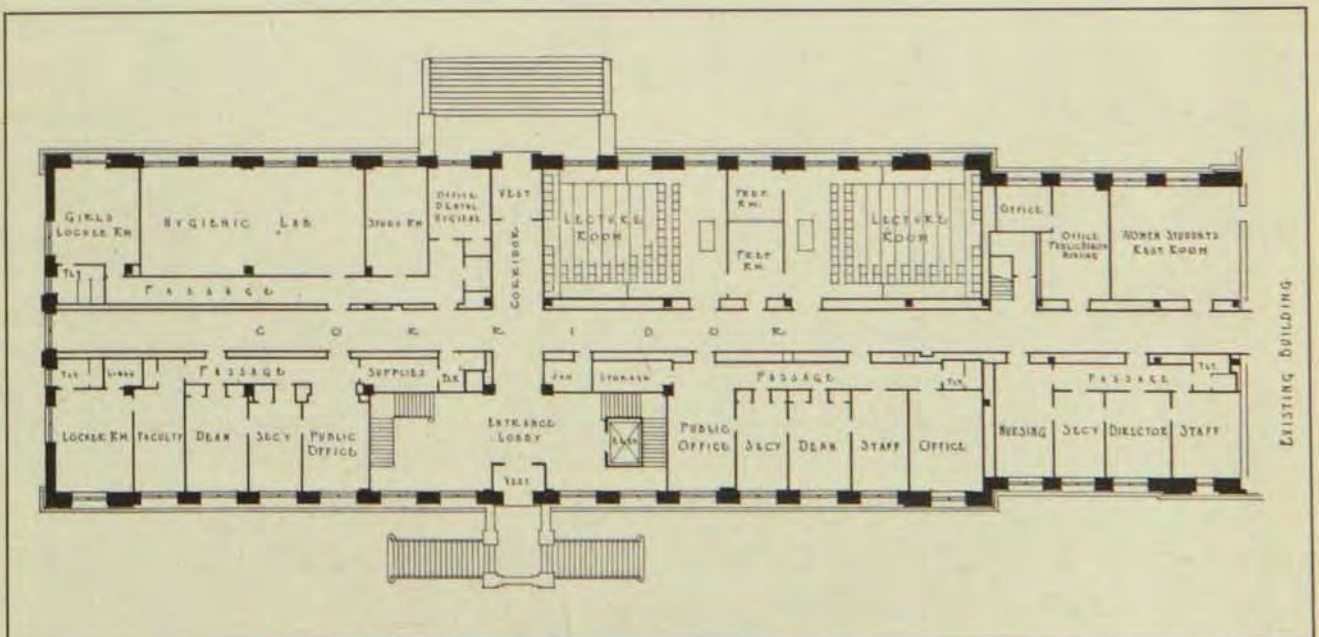
First Floor Plan, Dentistry Building
