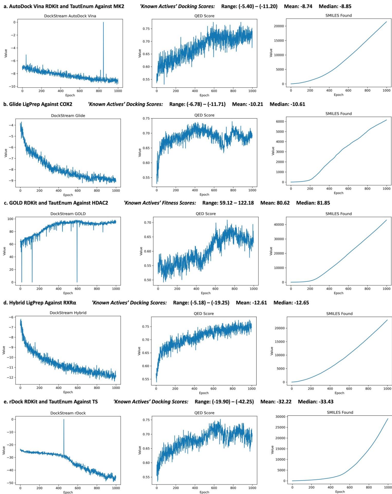
Fig. 4 REINVENT-DockStream agent reinforcement learning training progress for selected experiments: a. AutoDock Vina with RDKit and TautEnum against MK2 (PDB ID: 3KC3), b. Glide with LigPrep against COX2 (PDB ID: 1CX2), c. GOLD with RDKit and TautEnum against HDAC2 (PDB ID: 3MAX), d. Hybrid with LigPrep against RXR \alpha (PDB ID: 2P1RT), and e. rDock with RDKit and TautEnum against TS (PDB ID: 1100) (see Supporting Information Fig. S16-33 for training plots of all experiments). 'Known Actives' docking scores (fitness scores for GOLD)
