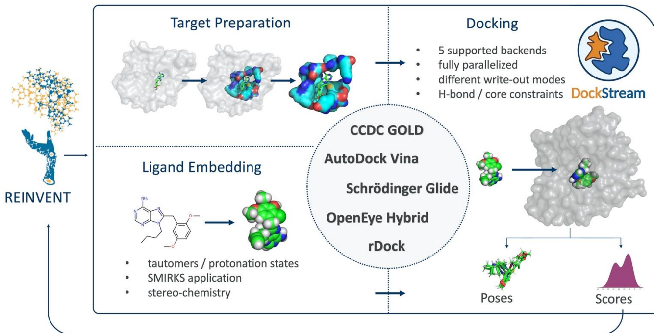
Fig. 1 Overview of DockStream platform providing access to a variety of docking backends. Target preparation, ligand embedding, and docking are handled in the unified platform. The docking scores and poses are outputted.
