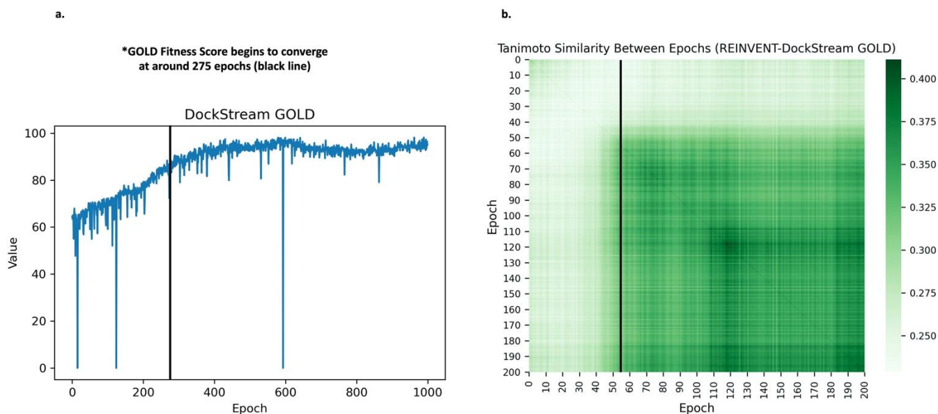
Fig. 6 Average linkage similarity between epochs (Tanimoto) for every 5 epochs for REINVENT-DockStream using GOLD with RDKit and TautEnum against HDAC2 (PDB ID: 3MAX). a. GOLD fitness score training plot (same as Fig. 4c). The vertical black line at around epoch 275 indicates the start of convergence whereby the GOLD fitness score begins to plateau. b. GOLD Tanimoto matrix illustrating the Tanimoto similarities between batches of generated compounds across the entire 1000 epochs REINVENT-DockStream experiment (x-axis is on the scale of 5 epochs, e.g. epoch 10 and 200 correspond to epoch 50 and 1000, respectively). The main diagonal is darker shaded, indicating notable intra-batch compound similarity. The overall matrix transitions from lighter (top left) to darker (bottom right) shaded areas. Cross-referencing with subplot a , neighbouring epochs display notably greater Tanimoto similarity, coinciding with GOLD fitness Score convergence. The results suggest the agent begins exploitation once a state of productivity is achieved (as measured by fitness score convergence). The overall transition of the matrix demonstrates agent exploration and exploitation.
