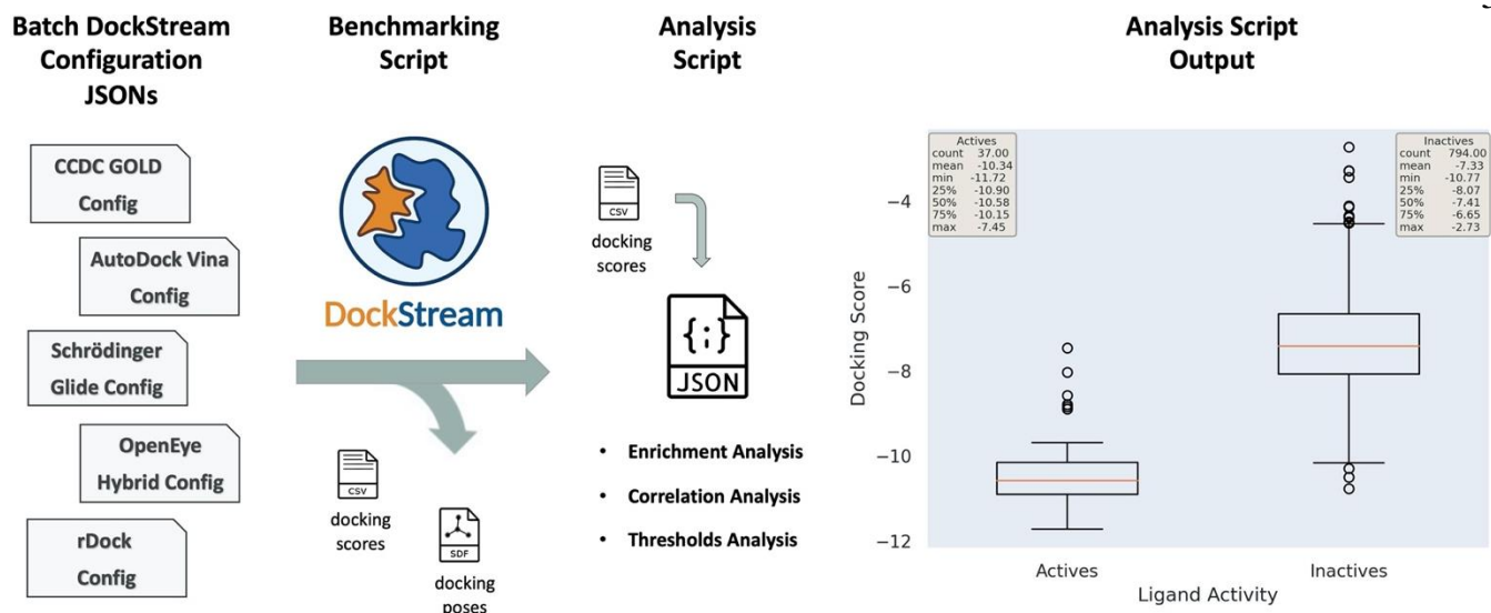
Fig. 2 DockStream automated molecular docking workflow via the benchmarking and analysis scripts. Each configuration JSON file specifies all the parameters required for a docking experiment. The analysis script supports 3 analysis modes: Enrichment, Correlation, and Thresholds (see Supporting Information for details).
