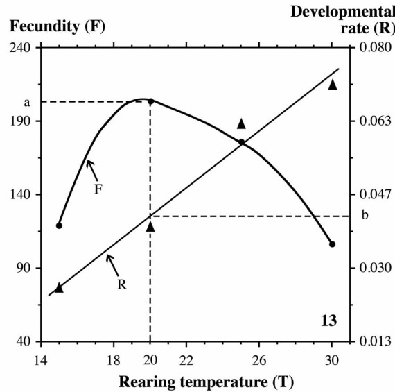
FIG. 13. Fecundity, F, as related to rearing temperature, T, and rate of larval development, R, in Adoxophyes honmai Yasuda (Tortricidae). Curve F fitted by connecting data points. Line R fitted by the improved linear model; R = 0.00435 T - 0.0462 . Data of Nabeta et al. (2005).
