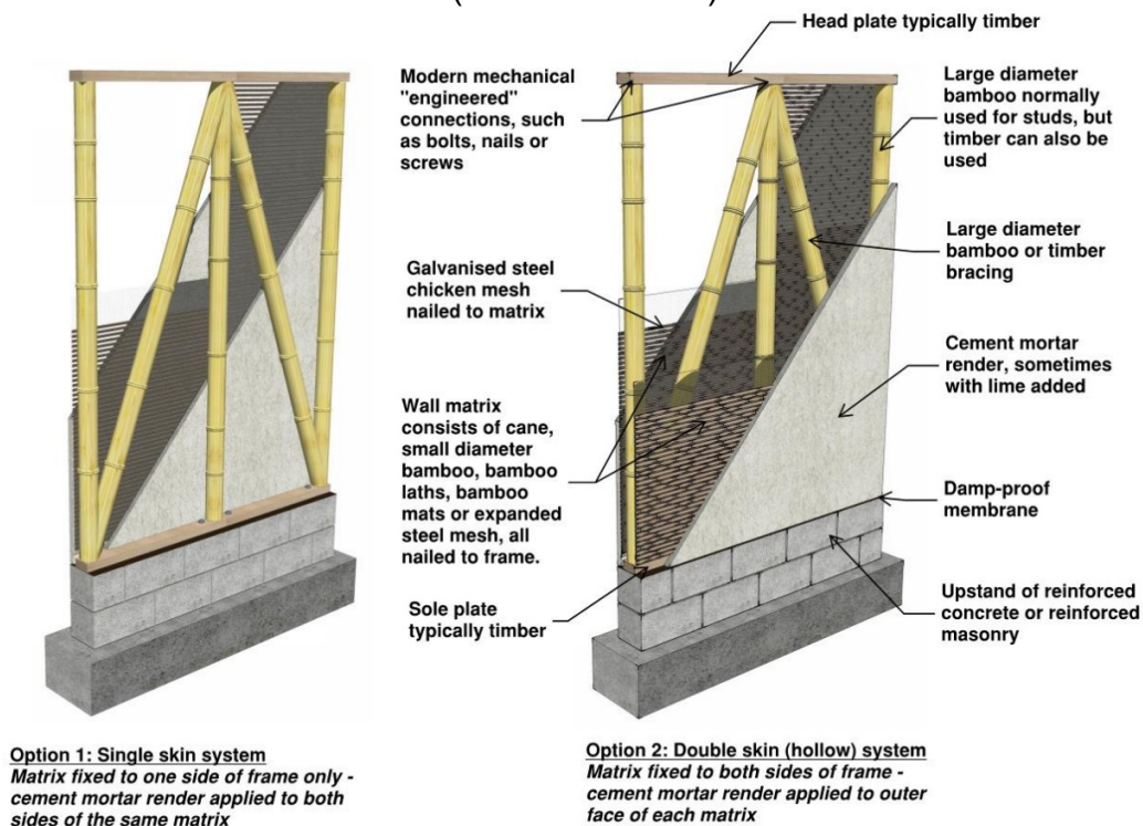
Figure 13: Characteristics of modern well-designed engineered bahareque housing: details of walling system
