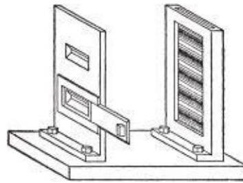
FIGURE 1.1. Niels Bohr’s depiction of the double-slit apparatus. (Cropped from Bohr [1949], 219. Reproduced with permission of Open Court Publishing Company, a division of Carus Publishing Company.)
