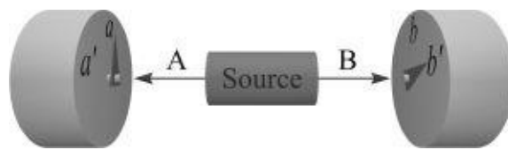
FIGURE 2.2. Bell's updated thought experiment, based on Bohm's version of the EPR setup. A source shoots out pairs of particles, A and B. Each detector has two directions along which it can measure a particle's spin, corresponding to the orientation of the magnets used to separate particles with spin up from those with spin down. As shown here, the apparatus is set to measure the spin of particle A along one direction (setting a ) and the spin of particle B along a different direction (setting b' ). (Illustration by Alex Wellerstein.)
