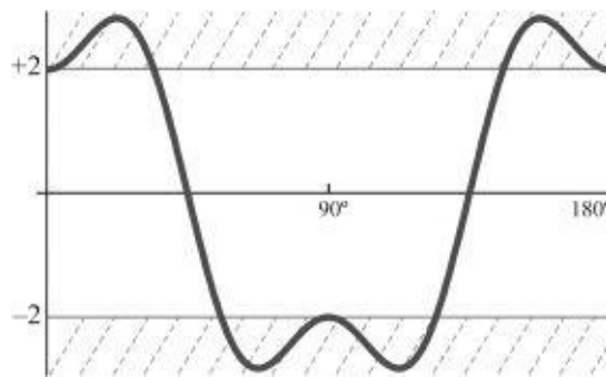
FIGURE 2.3. Predicted values for the quantity S , made up of combinations of spin measurements on particles A and B along various directions. The horizontal axis shows the angle between detector settings a and b' (or, equivalently, between a' and b ). As Bell demonstrated, the assumption that particles A and B carried definite values for spin along each direction prior to measurement—as Einstein and his collaborators had urged—limited S to lie between +2 and -2 . Yet the quantum-mechanical prediction for the correlation violated that bound by more than 40 percent for certain choices of angle. (Illustration by Alex Wellerstein, based on Aspect [2002], 130.)
