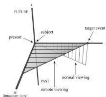
FIGURE 4.6. Elizabeth Rauscher's multidimensional approach to nonlocality and remote viewing. In this example, a subject sitting at the origin ( x = 0 and t = 0 ) can receive signals instantaneously from the “target event,” separated in space from where she is sitting, if those signals travel through the imaginary-time dimension. (Illustration by Alex Wellerstein, based on Rauscher [1979], 60.)
