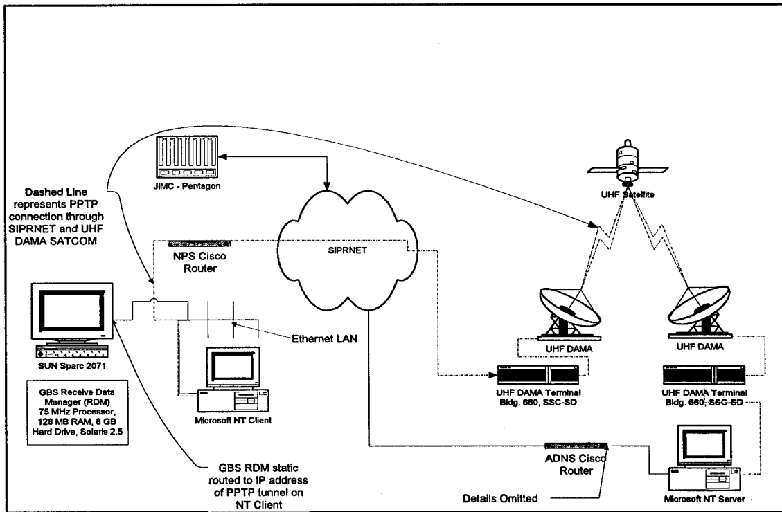
Figure 16 PPTP Tunnel
