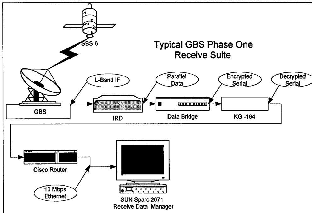
Figure 1 GBS Phase One Receive Suite
