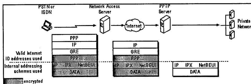
Figure 4 PPTP Connection
