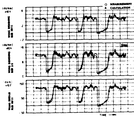
FIG.18 COMPARISON OF OLMS-CALCULATED AND FTI-MEASURED LOADS DURING DIFFERENT TAKE OFF CONFIGURATIONS
