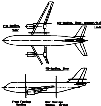
FIG. 3 MAIN COMPONENTS FOR FTI-STRAIN GAUGE MEASUREMENTS AND LOAD CALCULATIONS
