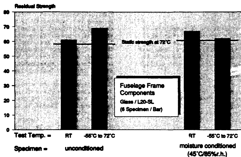
FIG.5 Influence of Combined Load- and Temperature-Cycles Residual Strength Tests at 72°C after 3*30.000 Flight Hours /4/
