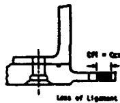
B) Dry (tab) hole at Rear Spar Location A7 Figure 7B
