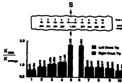
Figure 10. ABE determined stress intensity factor distribution for an open hole 3030 experiment (the crack lengths above are in inches).
