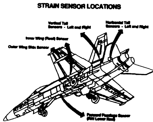
Figure 8 CF-18 Strain Sensor Locations
