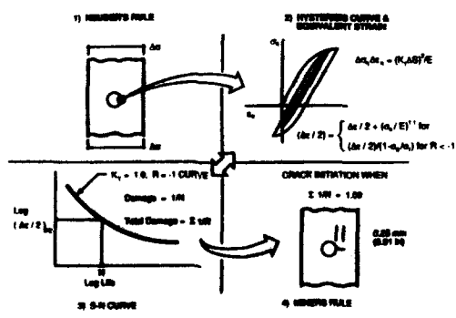
Figure 11 Crack Initiation Concept
