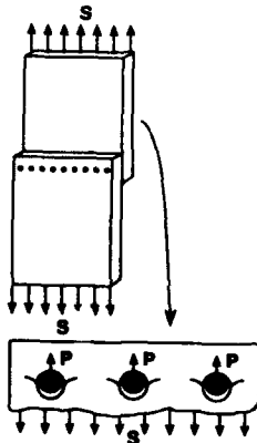
Figure 6. Fracture mechanics analyses of multiple-slit cracks.
