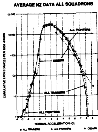
Figure 1 CF-18 Nz Exceedance Curves
