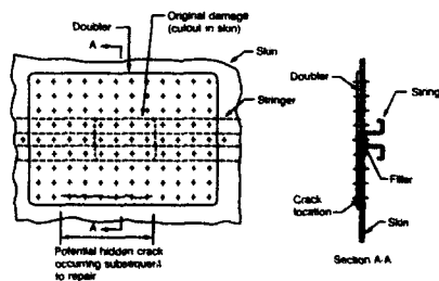
Figure 21. Typical Fuselage External Skin Repair
