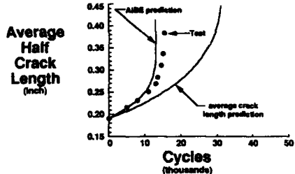
Figure 11. Predicted fatigue crack growth behavior for an open hole MSD experiment.
