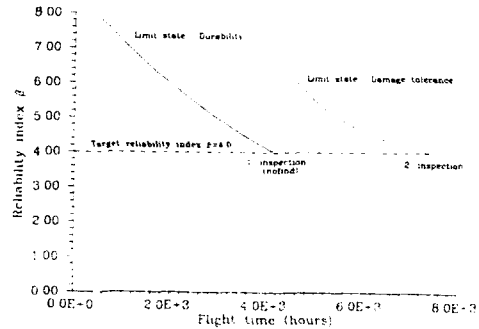
Figure 9: Results from the durability analysis ( t < 4100 flight hours) and the damage tolerance analysis, including reliability updating based on no-find in 1. inspection.
