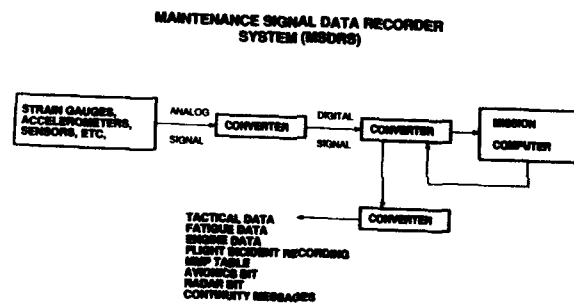
Figure 7 MSDRS System Components
