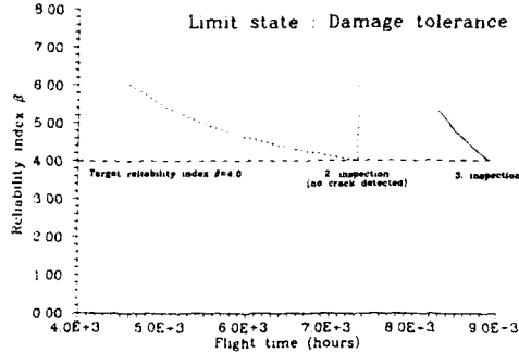
Figure 10: Results from the damage tolerance analysis ( t \geq 4100 flight hours), including reliability updating based on no-find in 1. and 2. inspection.
