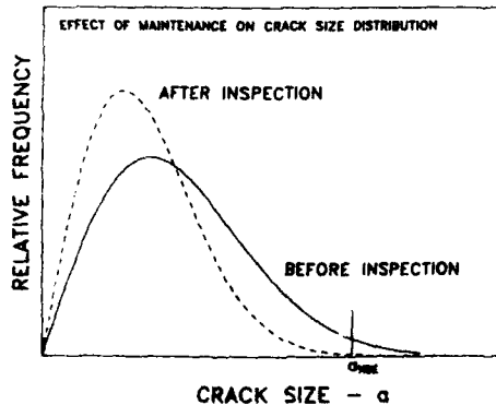
Figure 6. Effect of Maintenance on Crack Size Distribution
