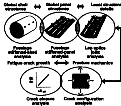
Figure 1. Integrated shell analysis-fracture analysis methodology.
