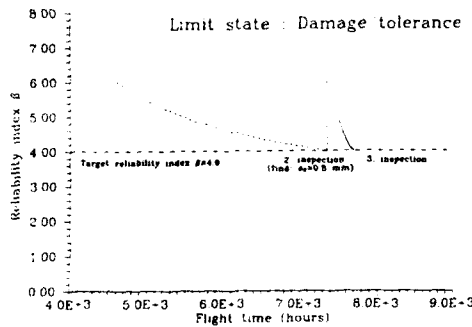
Figure 11: Results from the damage tolerance analysis ( t \geq 4100 flight hours), including reliability updating based on no-find in 1. inspection and crack is detected in 2. inspection, a_0 = a(t=7350) = 0.8 mm.
