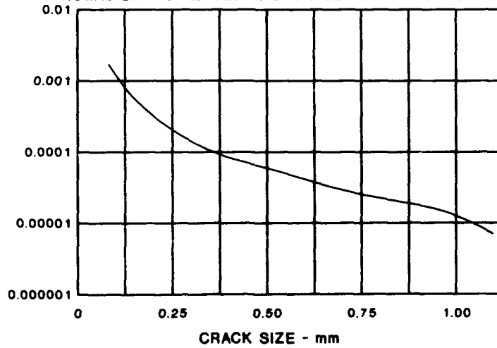
Figure 11. Crack Distribution from C-5A
