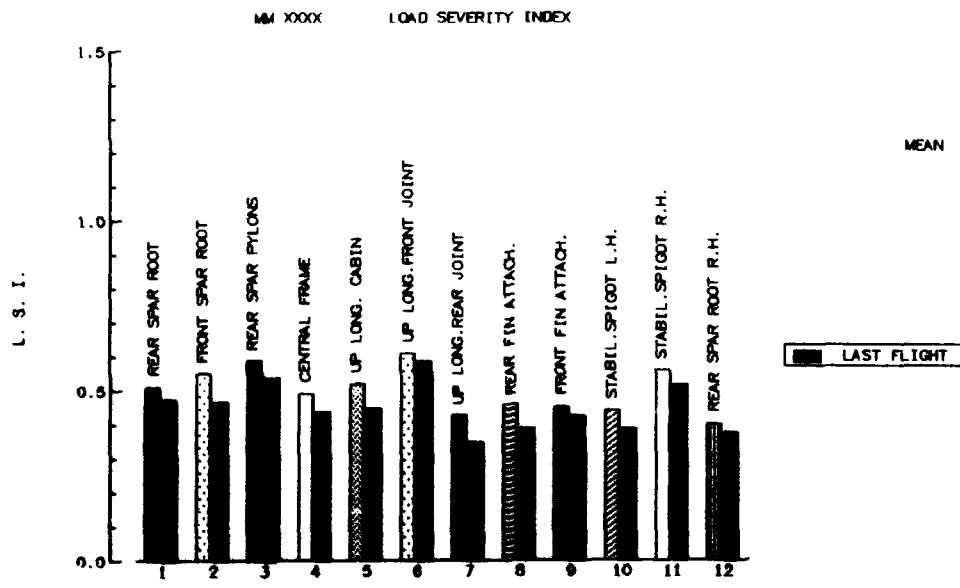
FIG.7 : Output (L.S.I.)
