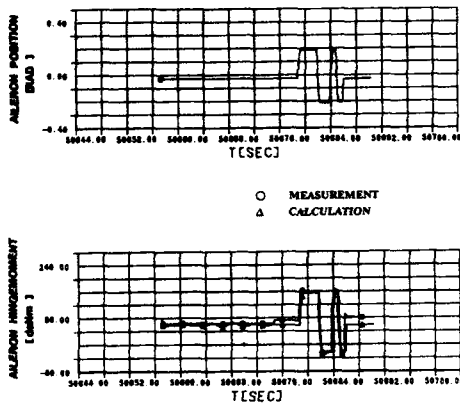
FIG.17 COMPARISON OF OLMS-CALCULATED AND FTI-MEASURED AILERON HINGEMOMENTS DURING A MULTISTEP MANEUVER
