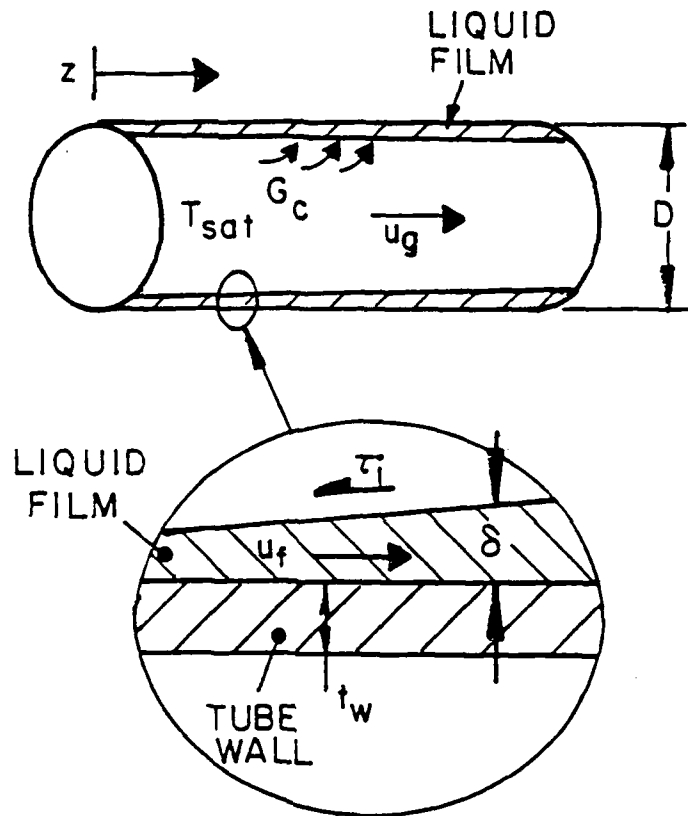
Figure 3.9. ANALYSIS VARIABLES FOR FLOW IN THE ANNULAR CONDENSATION REGIME
