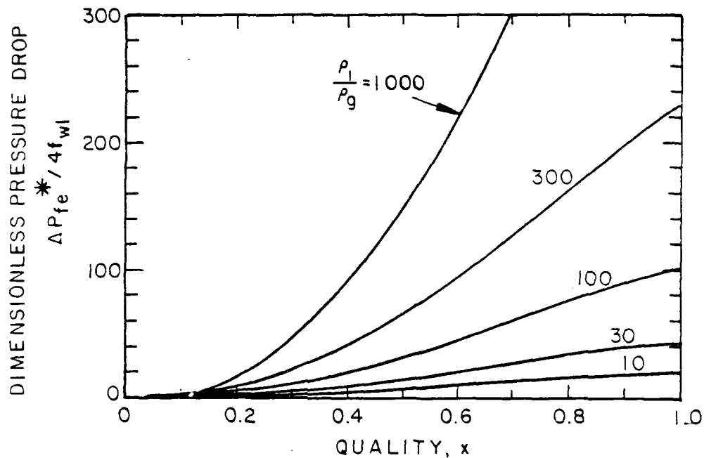
Figure 2.17. DIMENSIONLESS FRICTIONAL PRESSURE DROP IN THE EVAPORATOR
