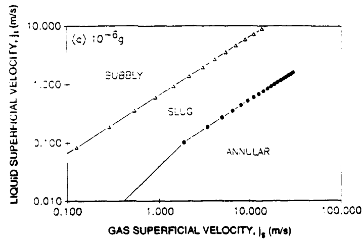
Figure 1.9. EFFECT OF GRAVITY ON FLOW REGIME MAP (SUPERFICIAL VELOCITY COORDINATES)
