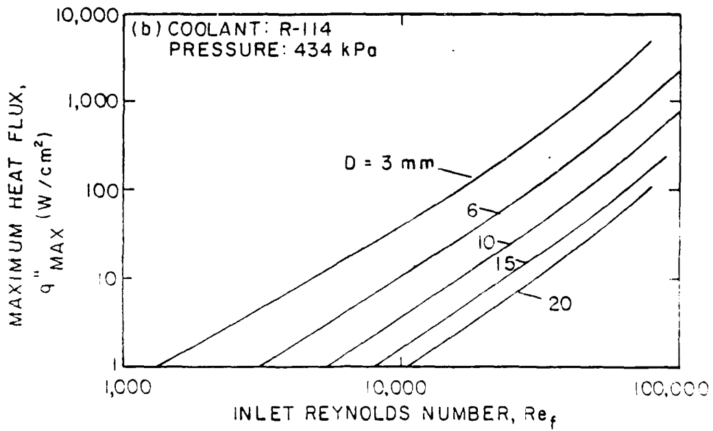
Figure 2.12. MAXIMUM HEAT FLUX FOR OPERATION IN MICROGRAVITY
