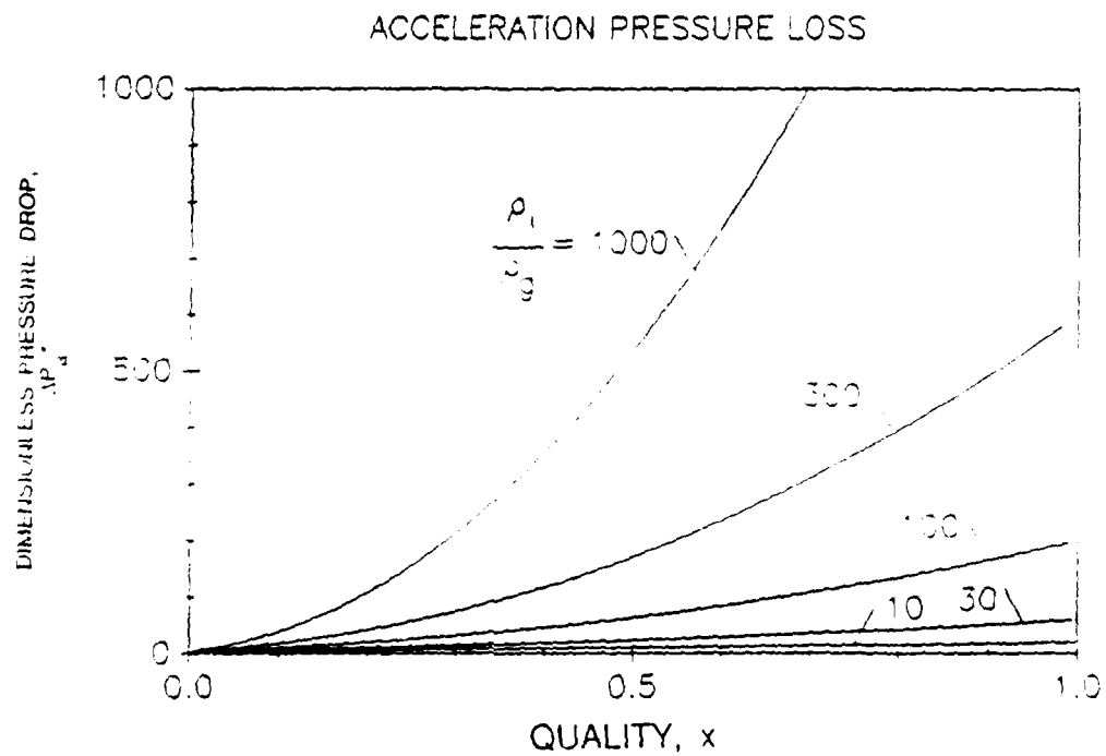
Figure 2.19. DIMENSIONLESS PRESSURE DROP DUE TO FLUID ACCELERATION IN THE EVAPORATOR
