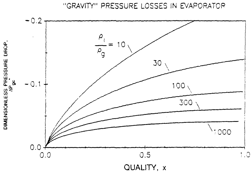
Figure 2.18. DIMENSIONLESS PRESSURE DROP DUE TO BODY FORCES IN THE EVAPORATOR
