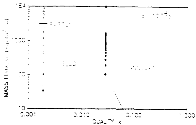
Figure 1.12. EFFECT OF GRAVITY ON FLOW REGIME MAP (MASS FLUX AND QUALITY COORDINATES)
