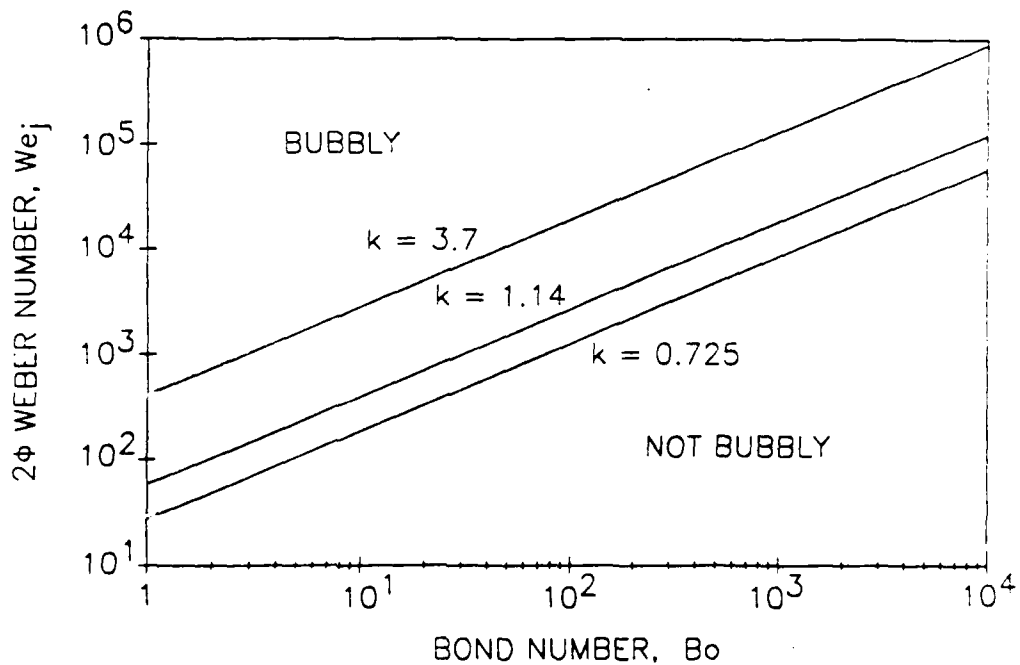
Figure 1.4. DIMENSIONLESS DESIGN MAP FOR SLUG-TO-BUBBLY FLOW REGIME TRANSITION (TURBULENCE CRITERION)
