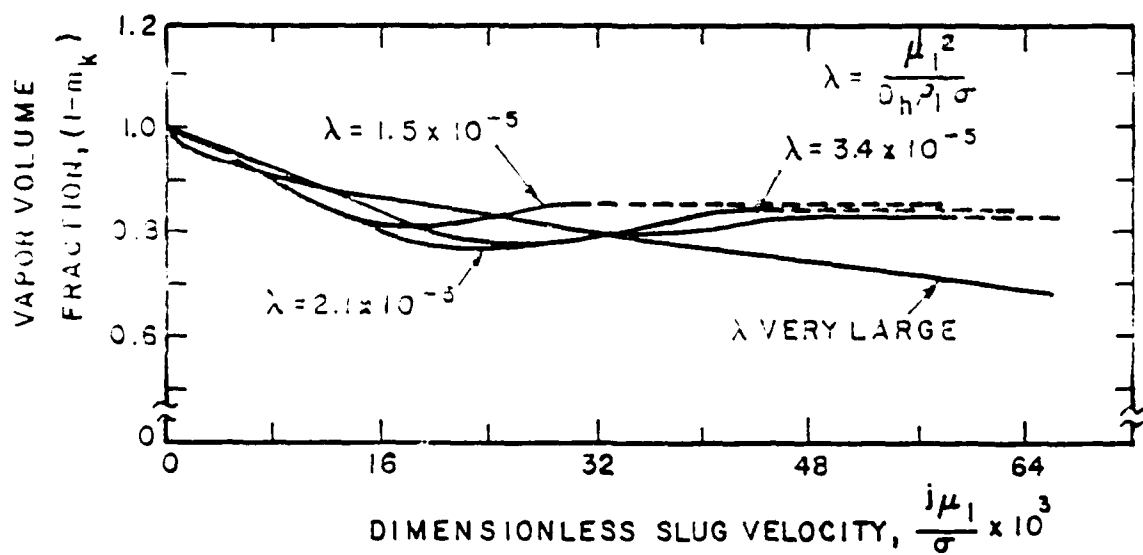
Figure 3.12. VELOCITY AS A FUNCTION OF j\mu_1/\sigma (Suo and Griffith, 1963)
