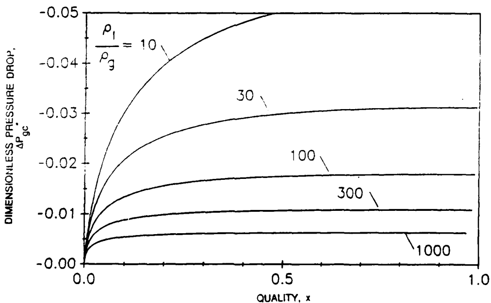
Figure 3.15. CONDENSER GRAVITY PRESSURE DROP
