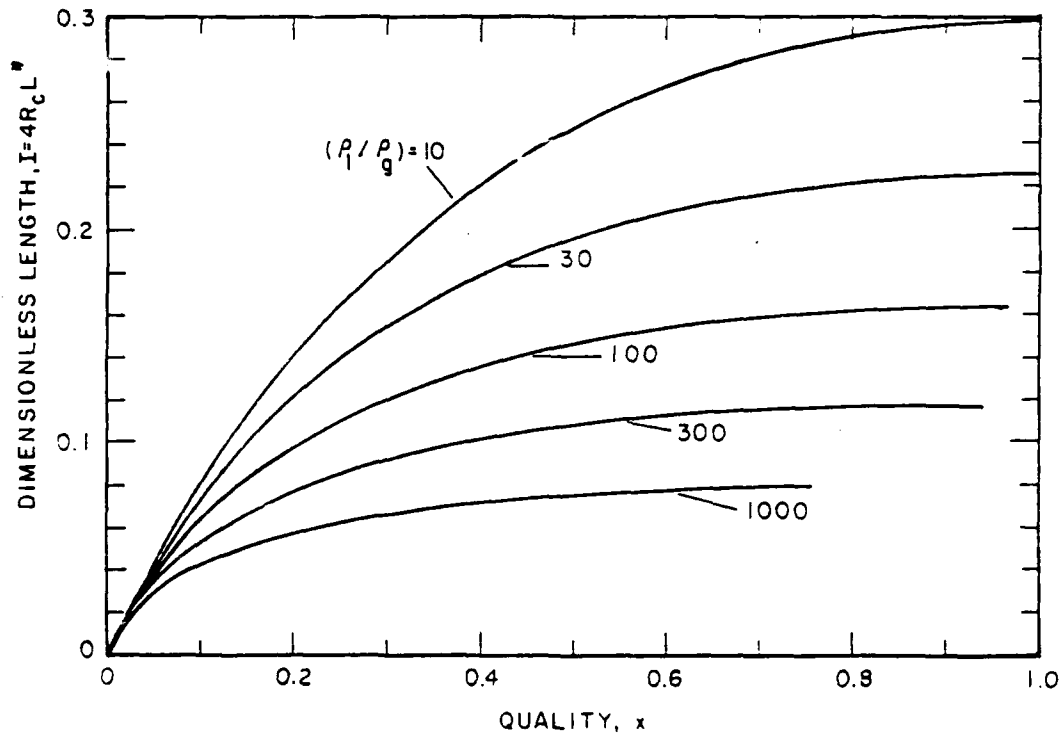
Figure 3.7. DESIGN LIMIT FOR THE LENGTH OF THE TWO-PHASE (ANNULAR) CONDENSER REGION ( f_l / f_{wg} = 1.0 )
