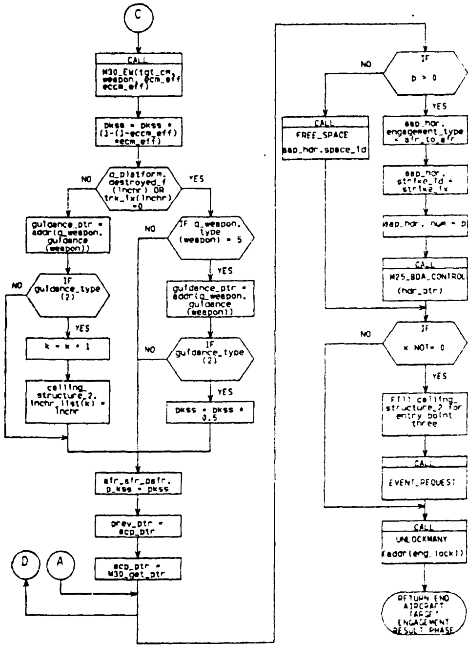
M20 AC AC 2 (1) AIRCRAFT TARGET ENGAGEMENT RESULT PHASE
