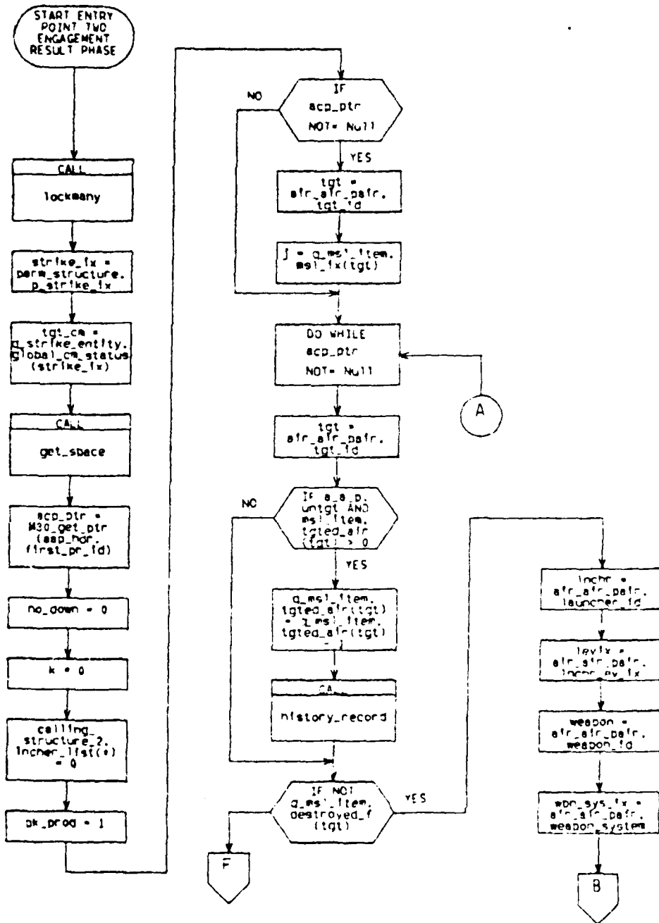
M20_AC_MSL (h) MISSILE TARGET ENGAGEMENT RESULT PHASE
