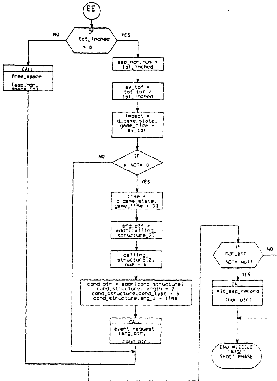
M20_AC_MSL (g) Preparation for Entry Point Two
