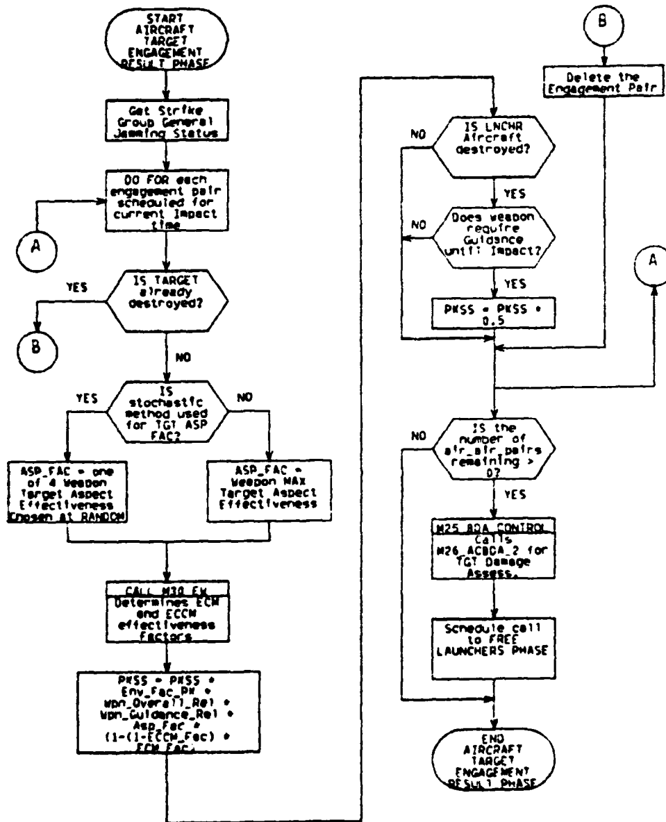
AIRCRAFT TARGET ENGAGEMENT RESULT PHASE
