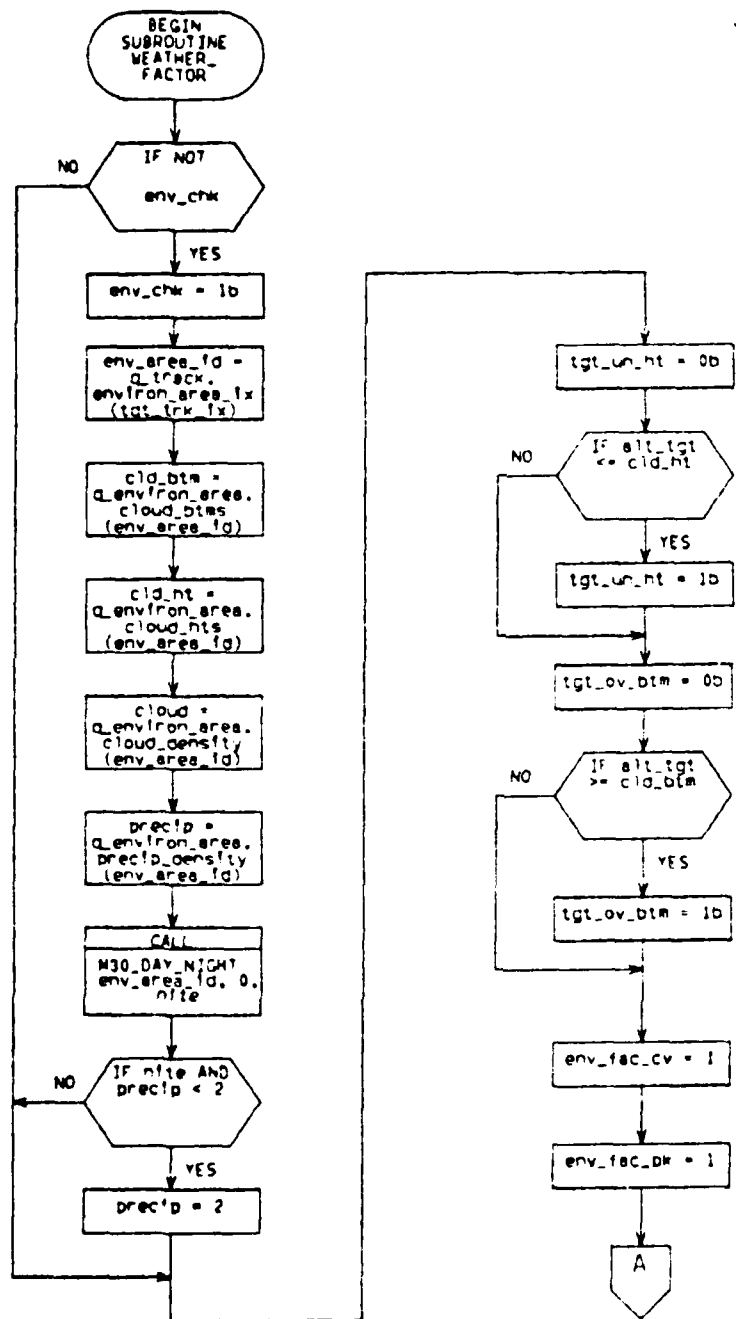
Subroutine WEATHER_FACTOR (a)
