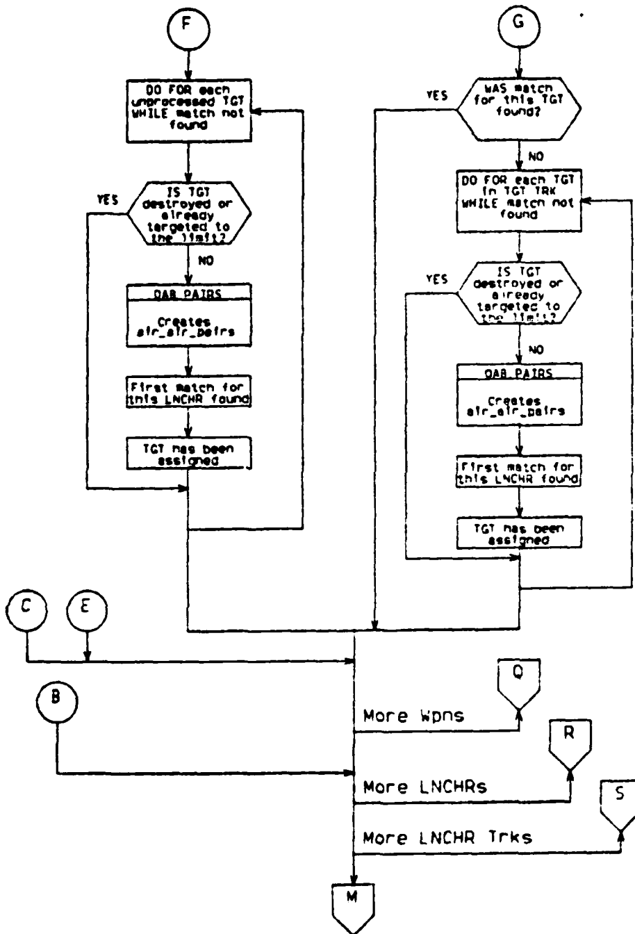
Subroutine TARGETING (b)
