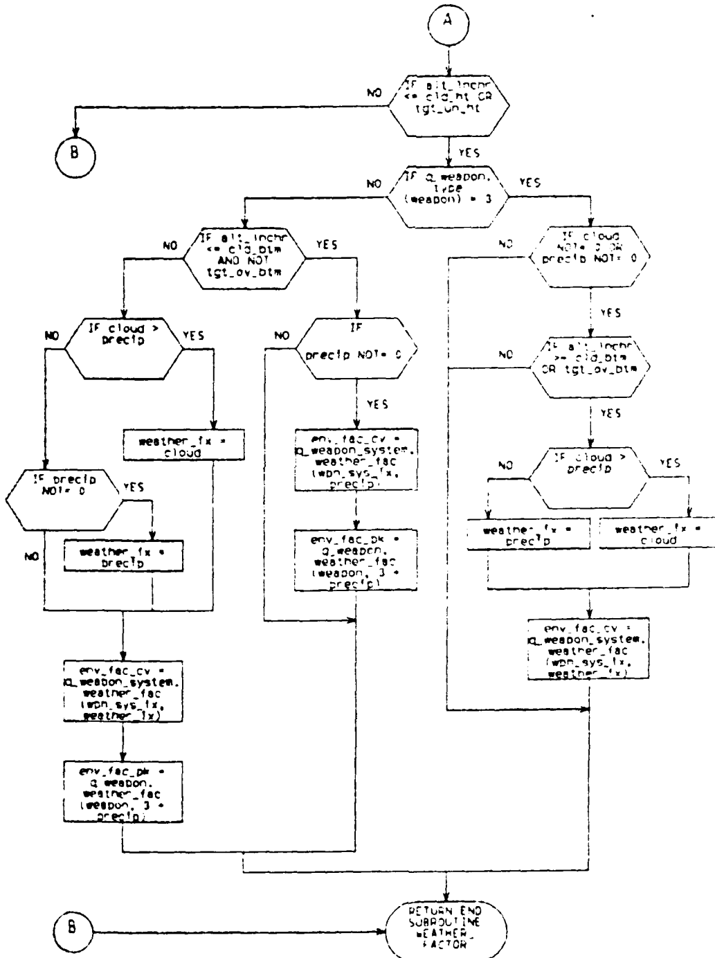
Subroutine WEATHER_FACTOR (b)
