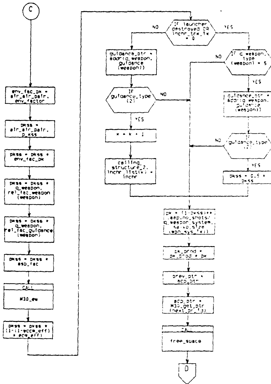
M20 AC MSL (j) Probability of Kill Determination
