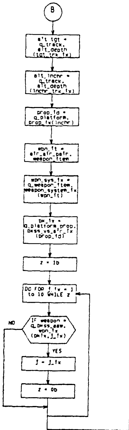
M20_AC_AC_2 (b) AIRCRAFT TARGET SHOOT PHASE
