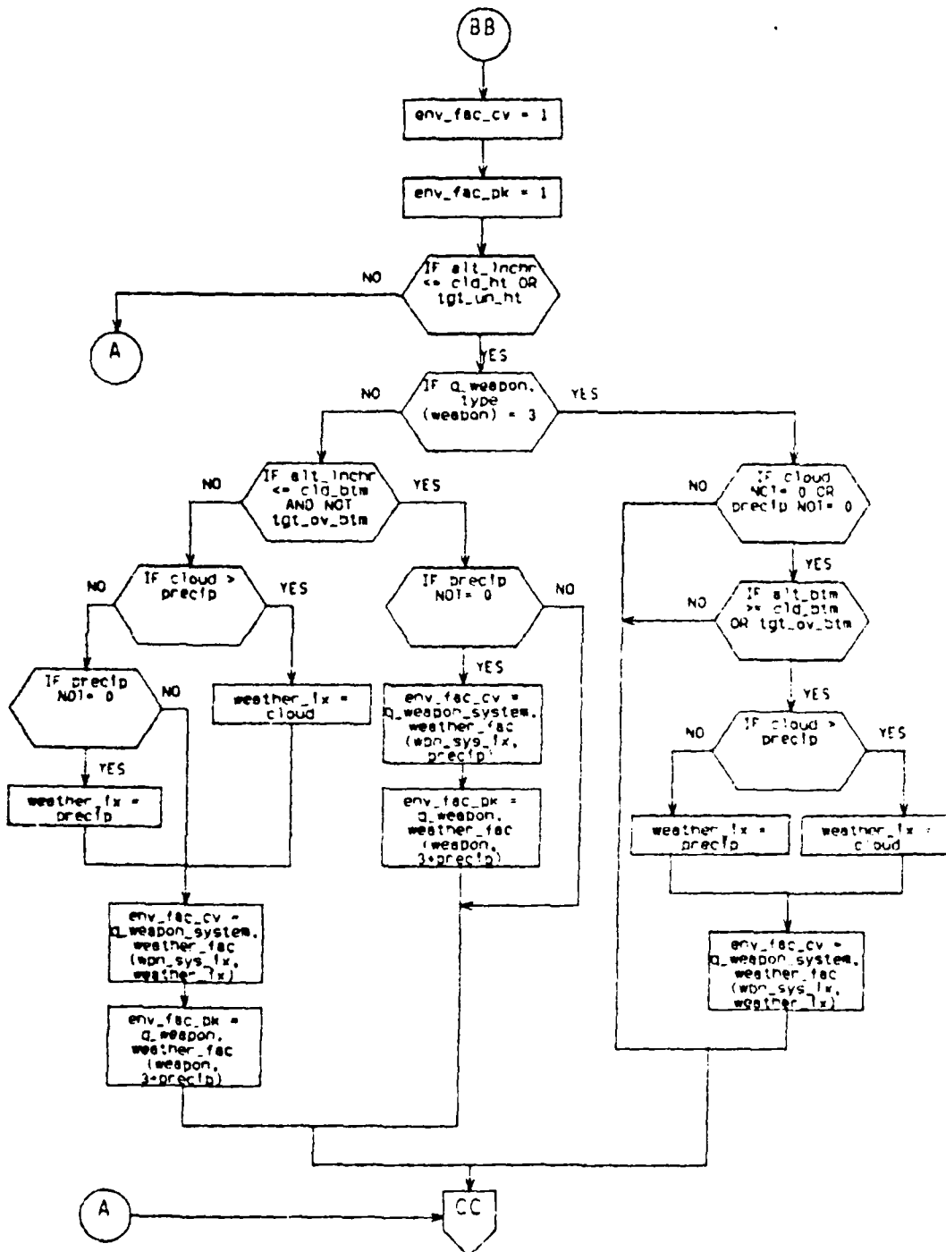
M20_AC_MSL (c) Weather Factor Determination
