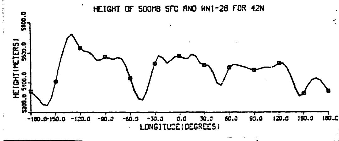
5e) Summation of wavenumber 1-28 components
