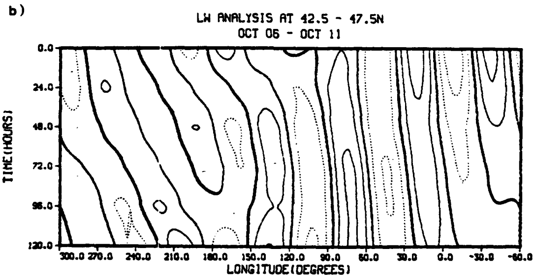
Figure 17. Same as Fig. 10 except for 06-11 Oct.
