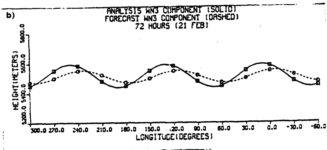
Figure 9. Wavenumber 1 and 3 Components for Case 1. a) Wavenumber 1 Component for Analysis (Solid) and Forecast (Dashed) for 00Z 21 Feb. b) Same as a except for Wavenumber 3 Component.
