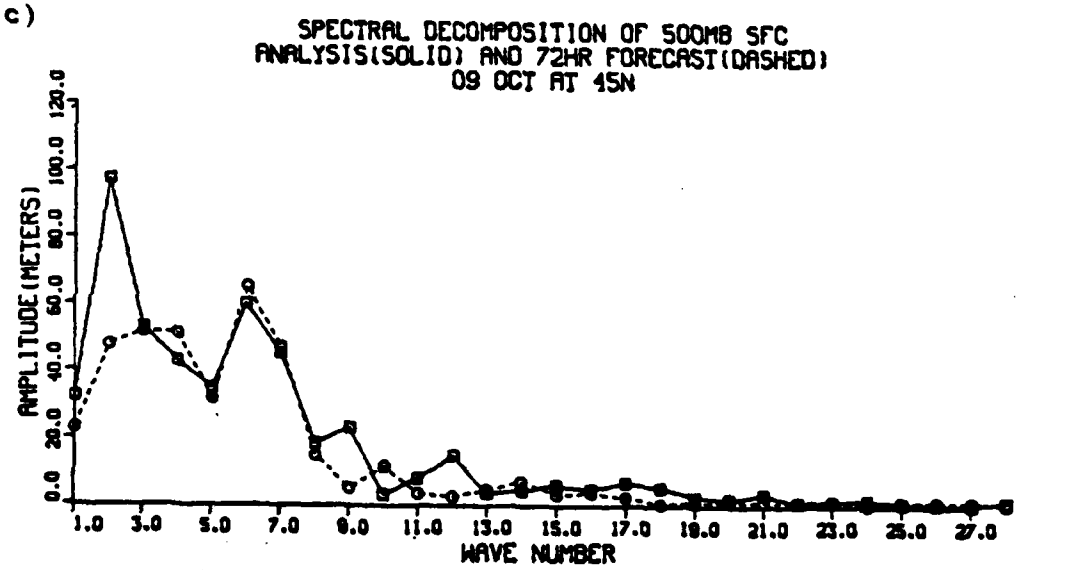
Figure 13. Same as Fig.7 except for 09 Oct.
