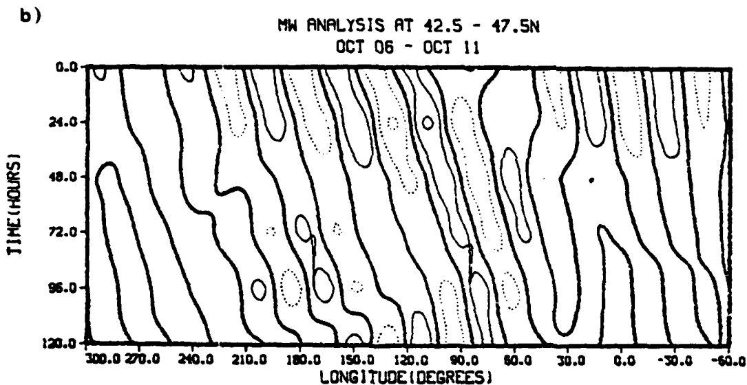
Figure 18. Same as Fig. 11 except for 06-11 Oct.
