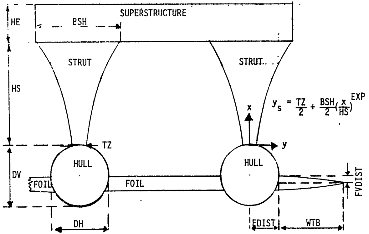
MIDSHIP SECTION
