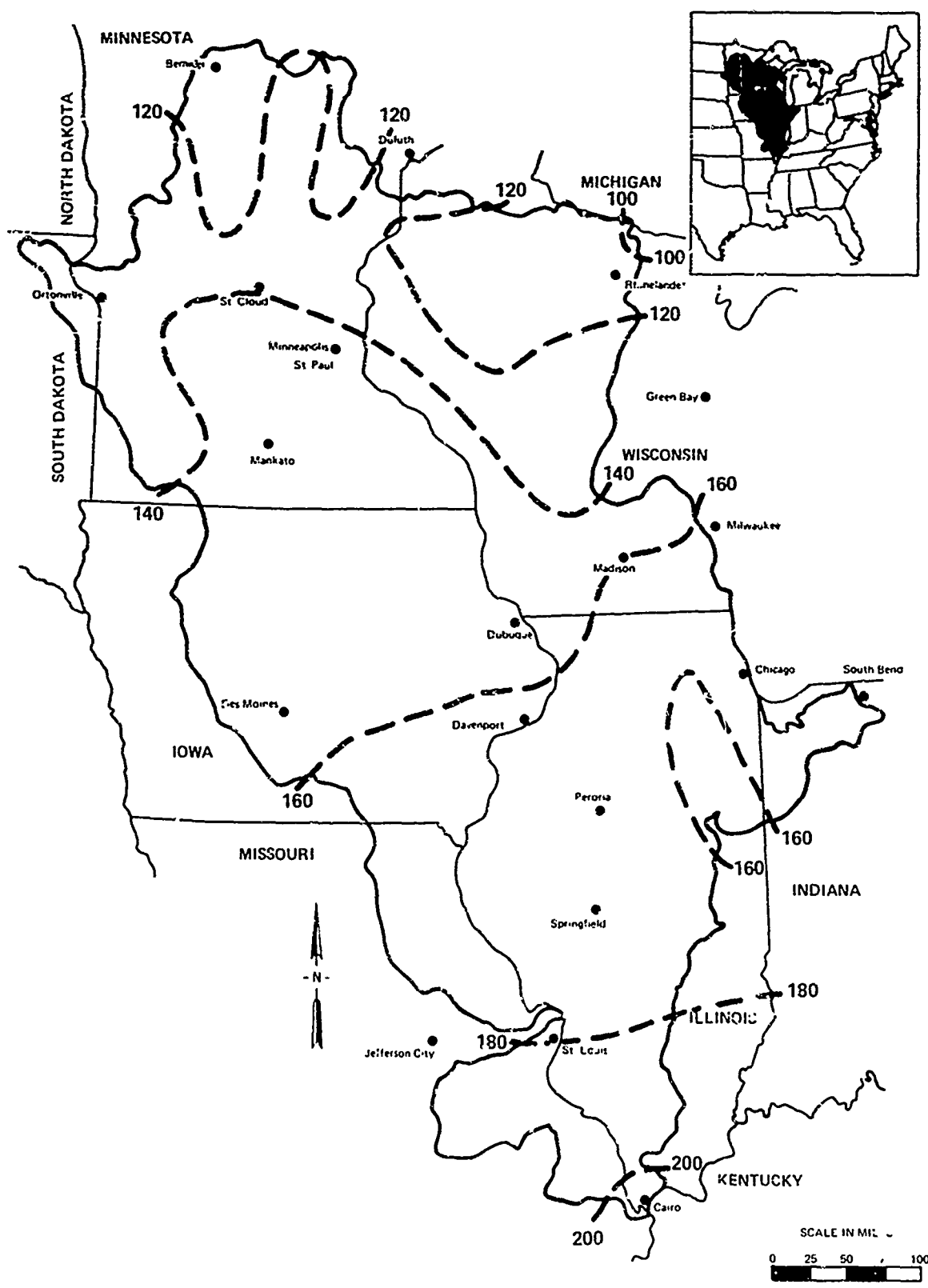
Figure P-36. Average length of frost-free period (days). Source: "Soils of the North Central Region of the United States," North Central Regional Publication No. 76, Bulletin 544, June 1960, p. 14.
