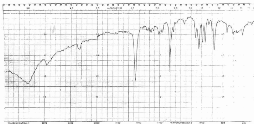
Figure 8. IR Spectrum of TMEFN.
