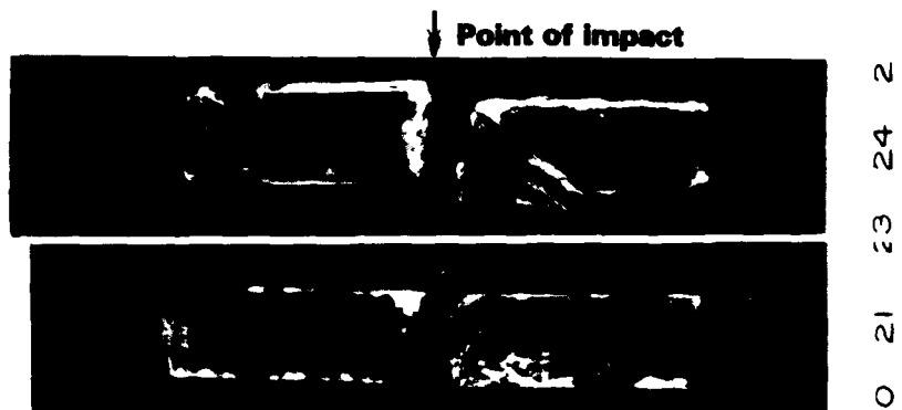
Figure 4. Typical example of normal mode fracture.
