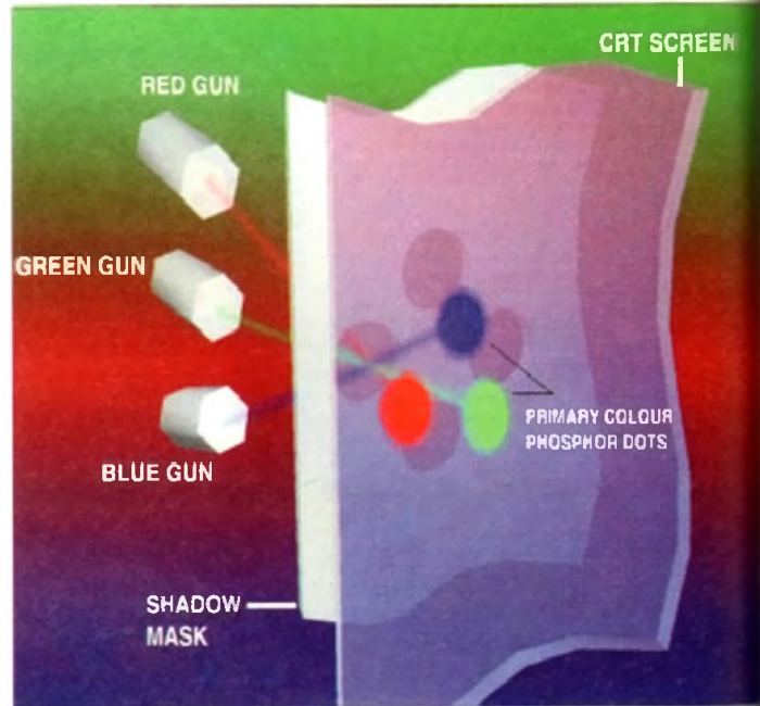
This illustration shows how the electron guns for each colour are aimed at their particular colour component of each phosphor triad. Note the Shadowmask screen to allow a degree of accuracy
