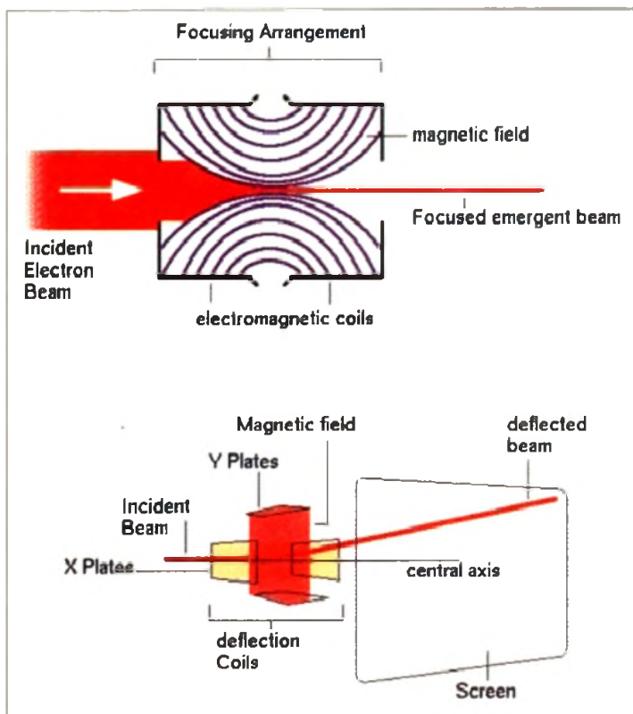
This diagram show the general layout of a cathode ray tube similar to that usually found inside an oscilloscope
