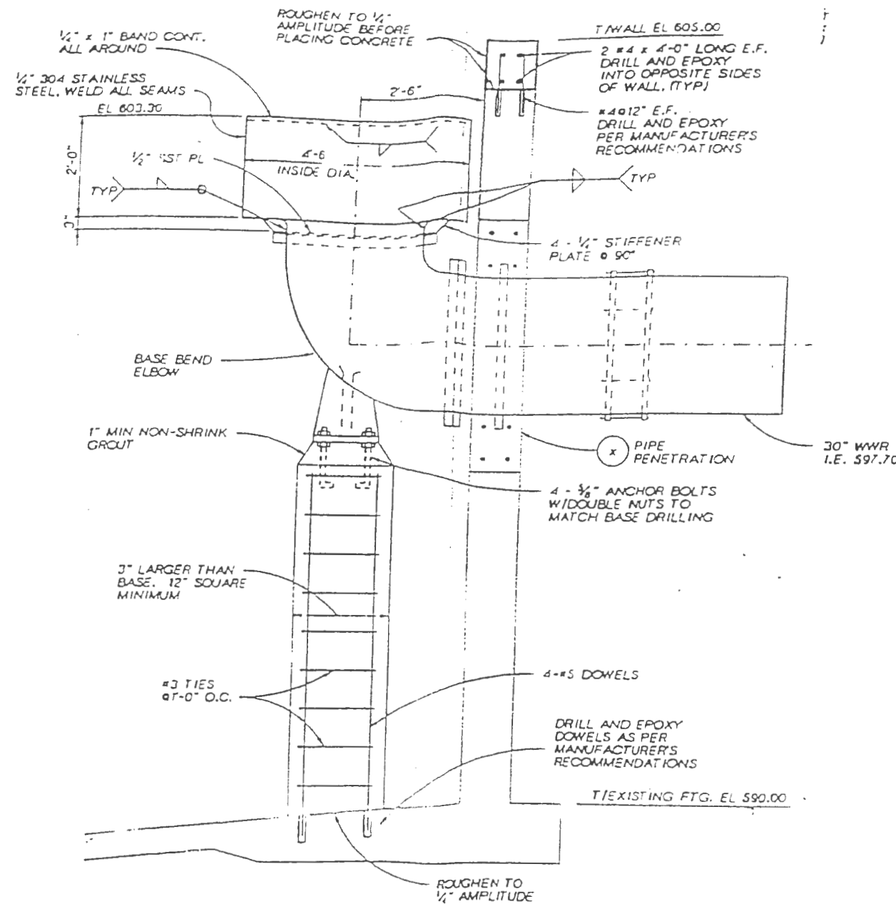
SECTION A 1/4" = 1'-0"
