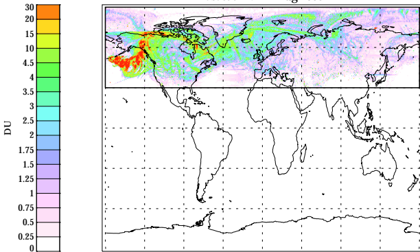
Kasatochi 7-22 Aug 2008
