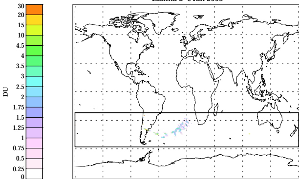
Llaima 2-6 Jan 2008
