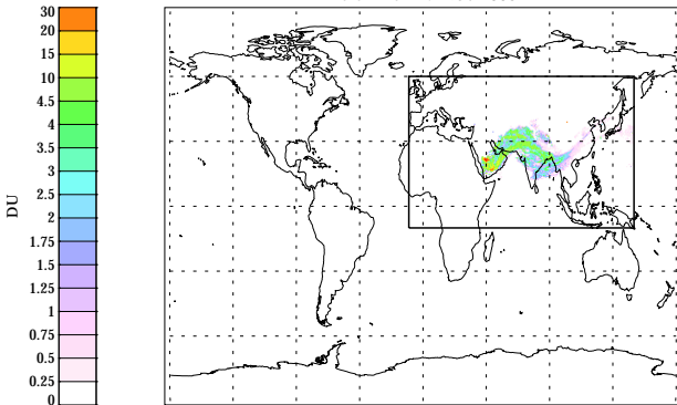
Dalaffilla 4-7 Nov 2008
