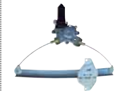
KAP1-B681EL KAP1-B681ER OPTIMA '01-06 RE WINDOW REGULATOR W/MOTOR 83403-38011 RL 83404-38011 RR
