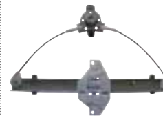
HYT3-B680ML HYT3-B680MR SONATA '99-05 FR WINDOW REGULATOR MANUAL #22 82401-38000/1 FL 82402-38000/1 FR
