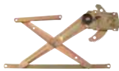
TYK2-B680ML TYK2-B680MR KIJANG '87 KF40/50 FR WINDOW REGULATOR MANUAL 69820-90K00 FL 69810-90K00 FR
