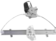
MBC4-B680EL MBC4-B680ER LANCER '93-96 MIRAGE '93-96 FR WINDOW REGULATOR W/MOTOR MB-927163 FL MB-927164 FR CW-608806 FL CW-608805 FR
