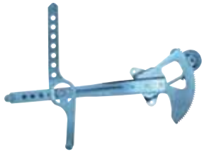
GSC6-B680ML GSC6-B680MR C/K1500/2500/3500 '88-02 SUBURBAN P/UP '95-99 ESCALADE '99-00 BLAZER '92-94 TAHOE '95-00 YUKON '92-99 YUKON DENALI '99-00 FR WINDOW REGULATOR MANUAL #95-4 22144289 FL 22144290 FR 0740-468/0740-469
